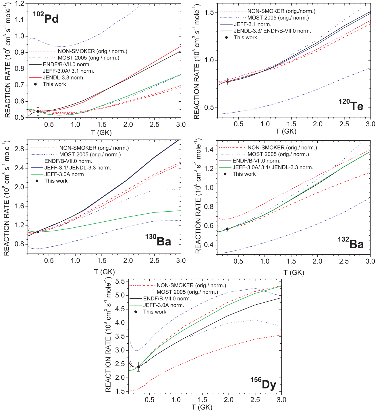
FIG. 4: (Color online) Stellar reaction rates (including f^* ) for temperatures between T=0.1 and 3 GK. Compared are the temperature-dependences of this work obtained with different extrapolations based on different evaluations. Also shown are the predictions of the Hauser-Feshbach models NON-SMOKER [17, 44] and MOST 2005 [19], each with their original values and renormalized to reproduce our data at kT=25 keV (0.29 GK). It should be noted that above 0.29 GK all values (including the ones from the evaluations) are based on energy dependences derived from Hauser-Feshbach models.
