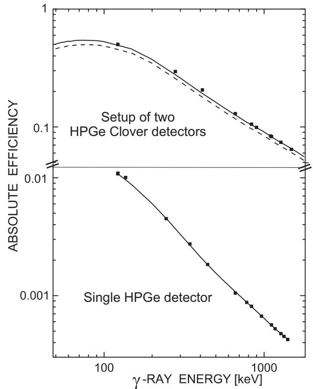
FIG. 3: Efficiency curves of the Clover detector system and the single HPGe detector. The statistical uncertainties of the calibration measurements correspond to the size of the symbols. The simulated efficiency of the Clover system (dashed line) was normalized to fit the measured data points.
