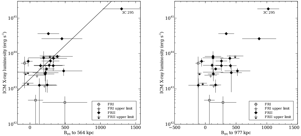
FIG. 7.— ICM luminosity vs the galaxy-quasar spatial covariance function B_{gq} (values taken from Herbert et al. 2013). B_{gq} is calculated within 564 kpc (left) and 977 kpc (right). The regression line is calculated for the FRII sources only.
