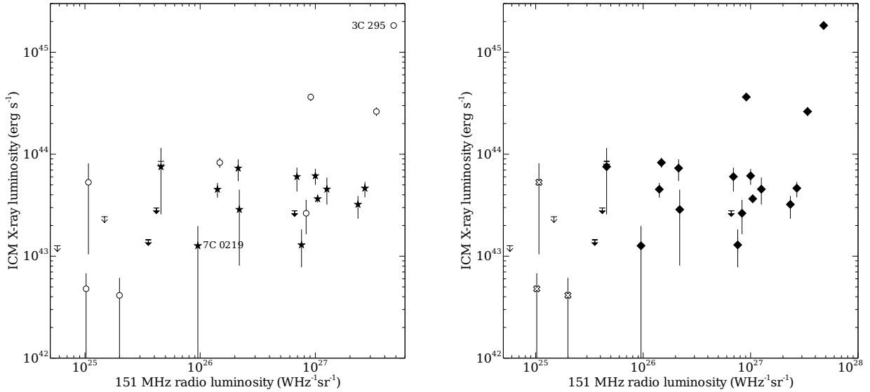
FIG. 4.— Radio luminosity vs ICM X-ray luminosity, separated into excitation classes (left), and FRI and FRII galaxies (right). In the left plot, open circles are LERGs, open arrows are LERG upper limits, filled stars are HERGs and filled arrows are HERG upper limits. In the right plot, open crosses are FRIs, open arrows are FRI upper limits, filled diamonds are FRIIs and filled arrows are FRII upper limits.
