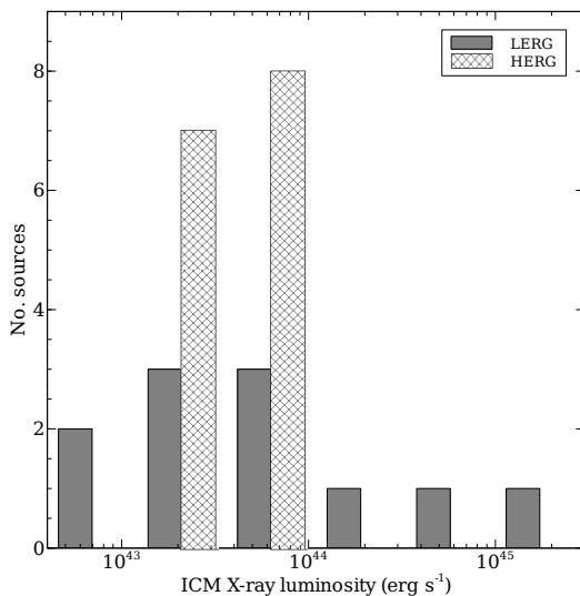
FIG. 5.— ICM X-ray luminosity coverage, separated into excitation classes.
