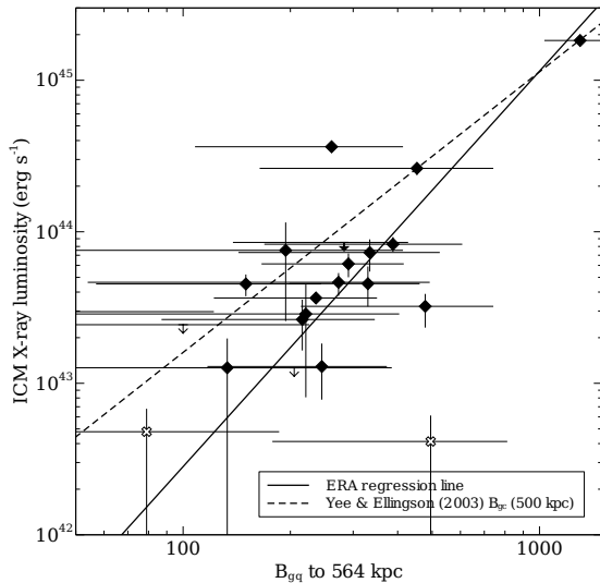
FIG. 8.— ICM luminosity vs \log_{10} B_{gq} for all positive values of B_{gq} (calculated within 564 kpc) overlaid with the scaling relations from the ERA sample (solid line) and Yee & Ellingson (2003) (dashed line). Note that Yee & Ellingson used B_{gc} calculated within 500 kpc.
