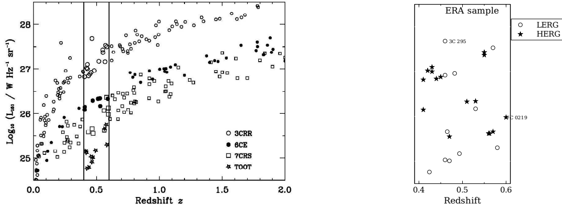
FIG. 1.— On the left, 151-MHz radio luminosity vs redshift for narrow-line radio galaxies in the 3CRR, 6CE and 7CRS samples, with galaxies from the TOOT survey added in the range 0.4 < z < 0.6 (McLure et al. 2004). The McLure et al. sample is in the 0.4 < z < 0.6 redshift interval. On the right, the ERA subsample used in this project.
