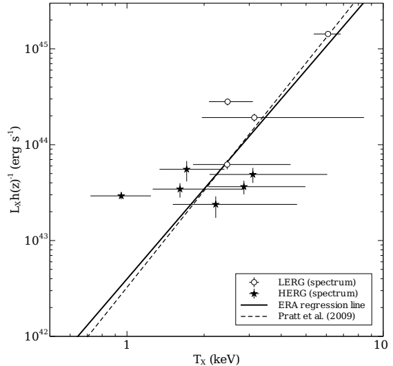
FIG. 6.— ICM luminosity vs temperature for the temperatures obtained by spectral analysis. The heavy, solid line shows the L_X - T_X relationship from all the ERA results (including estimated temperatures and upper limits) and the dashed line shows Pratt et al. (2009)'s L_X - T_X relation.
