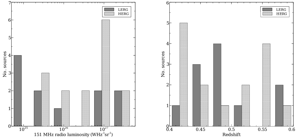
FIG. 2.— The ERA sample; Radio luminosity coverage (left) and redshift coverage (right).
