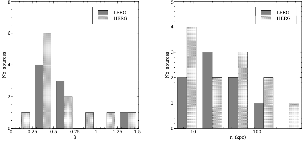
FIG. 3.— Distribution of the \beta model parameters; \beta (left) and core radius (right).
