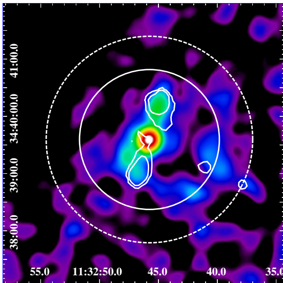
FIG. 10.— 6C 1132+3439. The chip edge was excluded for the analysis.
