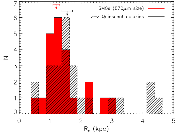
FIG. 7.— Comparison of the FWHM of the rest-frame FIR emission in SMGs to z \sim 2 quiescent galaxies, the proposed progenitors of local elliptical galaxies. The quiescent galaxies are selected to have strong 4000 Å / Balmer breaks, suggestive of an old stellar population, and are found to be compact in F160W/ HST imaging, with a median half light size of R_e = 1.5 \pm 0.2 , (van Dokkum 2008; Krogager et al. 2013).
