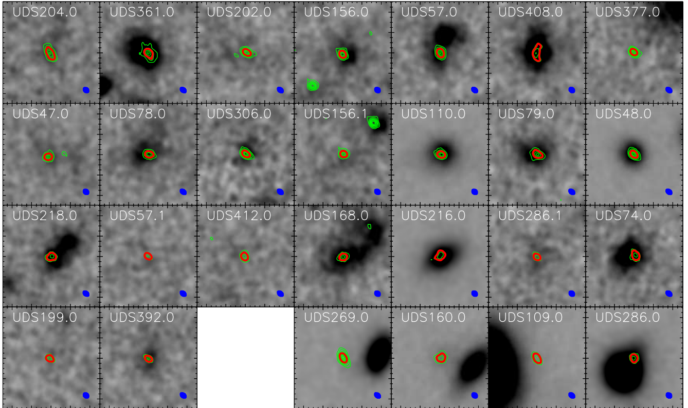
FIG. 1.— Grayscale K-band images of the 27 bright ( \text{SNR} > 10\sigma ) ALMA-identified SMGs in our sample. The images are in order of decreasing 870\ \mu\text{m} flux density, except for the final four panels, which are classed as potentially lensed SMGs (images are separated by a blank panel). Each panel is 5'' \times 5'' and we contour the ALMA maps over the images of the galaxies. The green contours on each image represent ALMA 870\ \mu\text{m} emission at 4, 8, 12, \dots \times \sigma , and a single red contour represents where the ALMA 870\ \mu\text{m} surface brightness is 50% of the peak value; for an ideal point source this contour should be identical to the size of the ALMA beam FWHM (bottom right of each panel). We note that the red contour appears more extended than the beam, indicating that these SMGs are resolved in the 0.3'' resolution ALMA data. Overall, 15% of the SMGs are not detected in the K-band imaging ( 5\sigma detection limit 25.0 mag).
