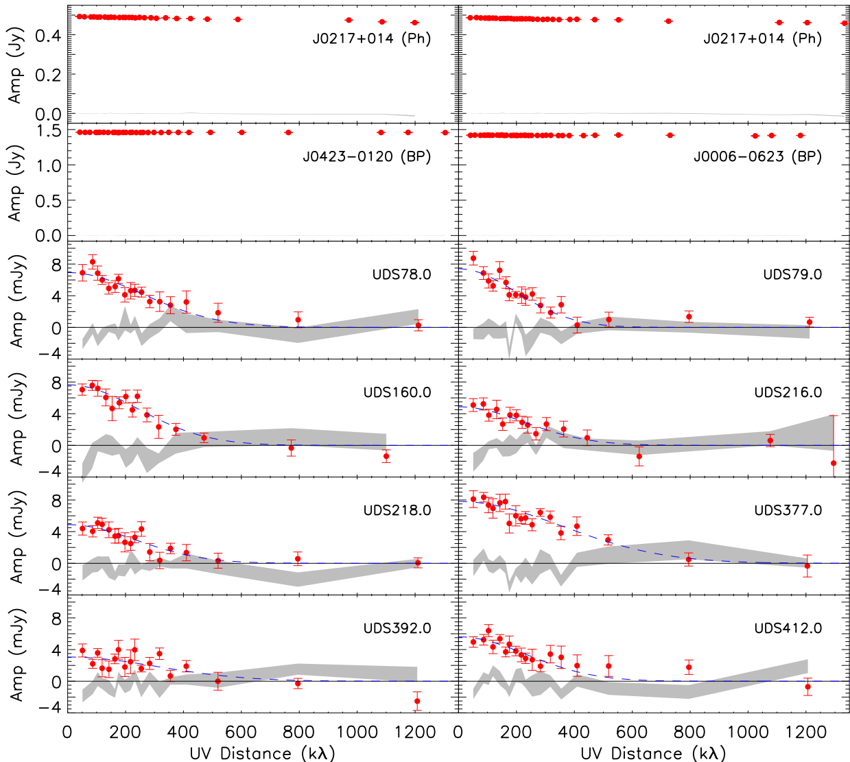
FIG. 2.— Components of the complex visibility versus uv -distance for the phase (Ph) and bandpass (BP) calibrators from both measurement sets (top), and an example eight SMGs from our sample (lower panels). The real components of the complex visibilities are plotted as data points, while the 1\text{-}\sigma range of the imaginary components is shown as a grey shaded region. Both the real and imaginary components are plotted on the same scale on the left axis. The amplitudes of both sets of calibrators are relatively flat with uv -distance, indicating that they are unresolved point sources, although we note a marginal drop in the flux of the phase calibrator, which suggests it is weakly resolved. In contrast the amplitudes for seven of the SMGs decline strongly with uv -distance, confirming our conclusion that these sources are resolved in the sub-mm imaging at 0.3'' resolution. We plot on each SMG a dashed line representing the best-fitting Gaussian to the amplitudes. We note that our measurements of the size and flux density of these SMGs in the image plane are consistent with the Gaussian fits to the amplitudes (the median ratio in size is \text{FWHM}^{\text{uv}} / \text{FWHM}^{\text{image}} = 0.9 \pm 0.2 ).
