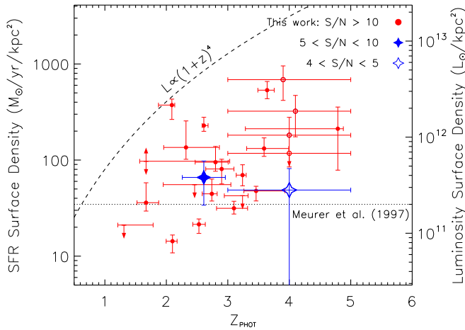
FIG. 6.— Star formation rate surface density of the SMGs in our sample as a function of redshift. The dashed line represents luminosity evolution L_{\text{IR}} \propto (1+z)^4 . A dotted line shows the 90 th percentile luminosity surface density for a sample of ultraviolet-selected sources (Meurer et al. 1997). The SMGs have a median star formation rate density of 90 \pm 30 \text{ M}_{\odot} \text{ yr}^{-1} \text{ kpc}^{-2} , and we note that no SMGs exceed the Eddington limit for a radiation pressure supported starburst ( \sim 1000 \text{ M}_{\odot} \text{ yr}^{-1} \text{ kpc}^{-2} ; Andrews & Thompson 2011)
