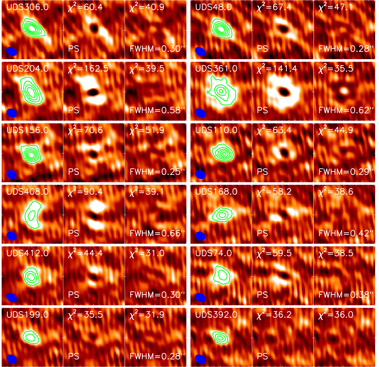
FIG. 3.— Examples showing 2'' \times 2'' images of our high resolution 870 \mu\text{m} maps ( 0.3'' ; left) alongside the residuals from fitting a point source model (PS; middle of each set of three panels) and an elliptical Gaussian model (resolved; right) for 12 example SMGs in our sample. The green contours represent 870 \mu\text{m} emission at 4, 8, 12, \dots \times \sigma , and the color-scale in each image is clipped at \pm 3\sigma . The ALMA beam is shown in the bottom left of the left-hand column. The SMGs presented here are chosen such that they span the full range in detection significance for the sample, and are a fair representation of the data quality of our ALMA maps. In eleven of these images there are significant residuals when fitting a point source model to the 870 \mu\text{m} emission, indicating that these sources are resolved in our ALMA maps. In contrast we highlight UDS392.0, which is well-described by a point source model and is classed as unresolved in our analysis. For the full sample of 23 SMGs the median difference in \chi^2 between the best-fit extended and point-source model is \Delta \chi^2 = 20 \pm 2 . We find that 22/23 SMGs are resolved in our 0.3'' resolution imaging, and derive a median angular size for the sample of 0.30 \pm 0.04'' (deconvolved FWHM of the major axis).
