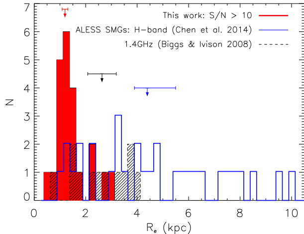
FIG. 5.— Comparison of the 870\ \mu\text{m} sizes of the SMGs in our sample, to the sizes of SMGs measured in 1.4 GHz/VLA imaging (Biggs & Ivison 2008) and H -band/ HST imaging (Chen et al. 2014). To allow a fair comparison between the samples we present all of the sizes in terms of an effective radius. The median size of the 12 SMGs identified in the 1.4 GHz imaging is R_e = 2.6 \pm 0.6 kpc, approximately double the median 870\ \mu\text{m} size of SMGs, R_e = 1.2 \pm 0.1 kpc. Convolution of the 870\ \mu\text{m} emission with a kernel of scale length 1–2 kpc, which is appropriate for modelling cosmic ray diffusion in star-forming galaxies at low redshift (Murphy et al. 2008), increases the median size of the SMGs to 3.8–5.2 kpc. Chen et al. (2014) measure a median size of R_e = 4.4^{+1.1}_{-0.5} kpc from rest-frame optical HST imaging of 17 interferometrically-identified SMGs at z = 1 –3. The H -band sizes of these SMGs are on average 3 times larger than the 870\ \mu\text{m} sizes presented here, indicating that the obscured star-forming region in SMGs is compact relative to the stellar emission.
