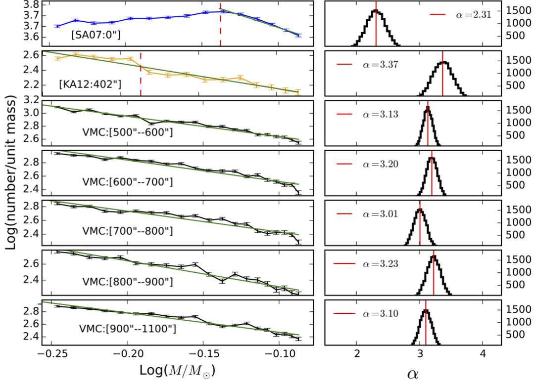
FIG. 7.— 47 Tuc MFs, obtained by dividing the slope of the MLR by the LFs of Fig. 5. Top two panels: The SA07 MF, pertaining to the cluster’s central region, shows a decline in stellar numbers for m_* < 0.72M_\odot . In contrast, the KA12-based MF in the outer region reveals a deficit for m_* > 0.65M_\odot . Bottom five panels: MFs at different radii in the outskirts of 47 Tuc. All annuli exhibit power laws, with no evidence of any deficit or surplus for masses in excess of 0.6 M_\odot . We thus fitted all the MFs with the power laws and performed Monte Carlo simulations, shown on the right.
