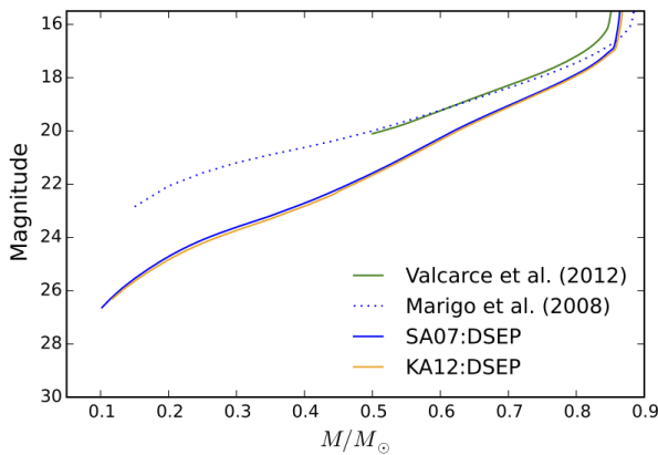
FIG. 6.— MLR based on the DSEP, PGPUC (Valcarce et al. 2012), and Padova (Marigo et al. 2008; Girardi et al. 2010) models for both the VMC's Y-band magnitudes and the HST F606W filter. The blue and orange curves are the DSEP MLRs for the HST data, while the green curve represents the PGPUC model for the VMC data. The dotted line is the Padova model pertaining to the VMC data, shown for comparison.
