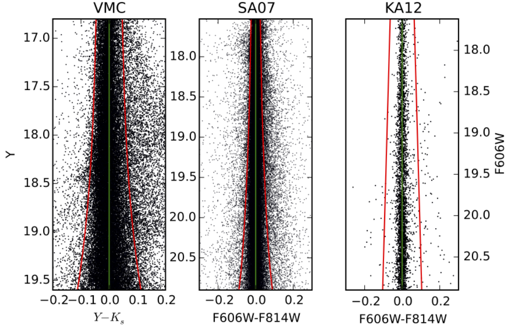
FIG. 4.— 47 Tuc CMD, “normalized” by removing the trend defined by the MS ridge line. The red lines are the 5\sigma , 4\sigma , and 3\sigma selections used to correct for the presence of background field stars. The green line is the zero-color reference.
