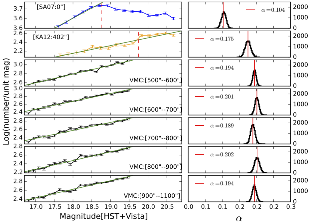
FIG. 5.— 47 Tuc MS LFs. LFs based on (top) the SA07 catalog for stars in the cluster center and (second panel) the KA12 catalog, containing stars located 6.7' west of the cluster center. The bottom five panels are local LFs for radial annuli covered by our VMC observations. The full annulus, r \in [500, 1100]'' , is divided into five radial subsets, i.e., r \in [500, 600]'' , r \in [600, 700]'' , r \in [700, 800]'' , r \in [800, 900]'' , and r \in [900, 1100]'' . The numbers of MS stars per unit magnitude versus apparent magnitude F606W are plotted; the error bars were estimated based on Poissonian counting statistics. The green line is the power-law fit to the LF, and the two arrows in top two panels are an indication of a possible LF break magnitude. The Gaussian distributions on the right are the results of our Monte Carlo simulations to determine the best-fitting power-law index \alpha .
