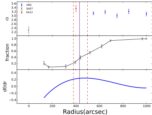
FIG. 9.— Top: \alpha as a function of radius in 47 Tuc. Middle: Fraction of FG stars, obtained by averaging the distributions of RGB and subgiant-branch stars in Li et al. (2014). Bottom: Derivative of the fraction of FG stars versus radius. The purple solid indicates the half-mass radius at about 9.6 pc ( 430'' ); we adopted a distance of 4.6 kpc to 47 Tuc) from the center of the cluster.
