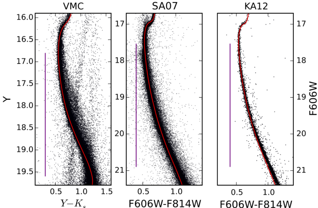
FIG. 2.— 47 Tuc CMDs. The red curves are the model isochrones defined in Table 1. The vertical purple lines indicate the magnitude ranges adopted for selecting MS stars.
