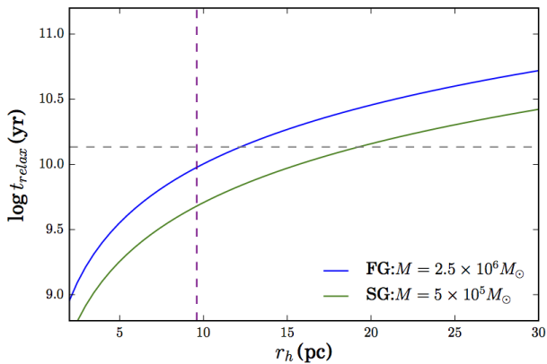
FIG. 8.— Half-mass relaxation timescale for (blue) first-generation stars and (green) second-generation stars as a function of radius in 47 Tuc. The grey dashed line represents an age of 13 Gyr, which intersects the first-generation prediction at r = 12.3 pc and the second-generation curve at r = 19.1 pc. The purple dashed line represents the observed half-mass radius at r = 9.6 pc.
