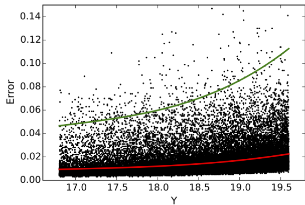
FIG. 3.— Photometric uncertainties as a function of magnitude for the VMC data set in the Y filter. The red solid curve represents the bin-averaged photometric uncertainties, while the green curve represents the 5\sigma range.
