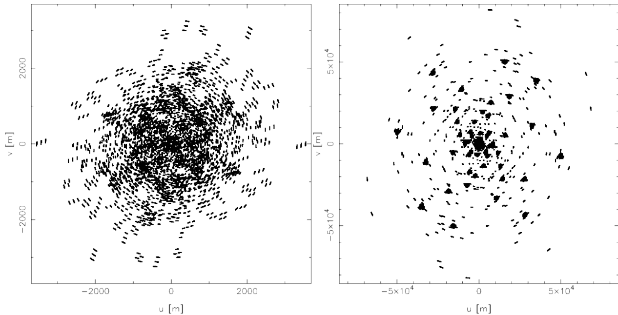
Fig. 3. The uv coverage for the MSSS-HBA field H229+70, core only (left) and all Dutch stations (right).
