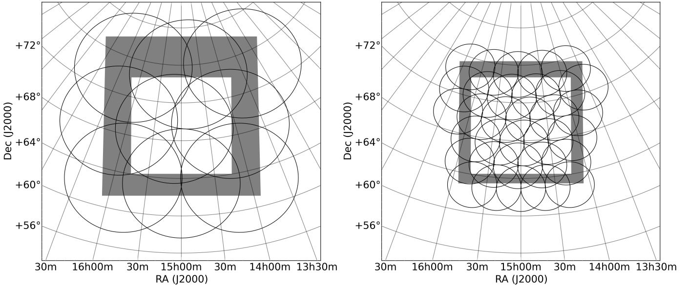
Fig. 9. Mosaic layout of the MSSS Verification Field (MVF). Left: The nine LBA fields making up the MVF, overlaid on the 10^\circ \times 10^\circ mosaic field (central white square). The gray border around the mosaic area is a guard area used to ensure that sufficient edge fields are included and to ensure flat sensitivity within the mosaic. Right: The 32 HBA fields making up the MVF, overlaid on the same central mosaic field. The guard border is smaller in proportion to the HBA field diameter.
