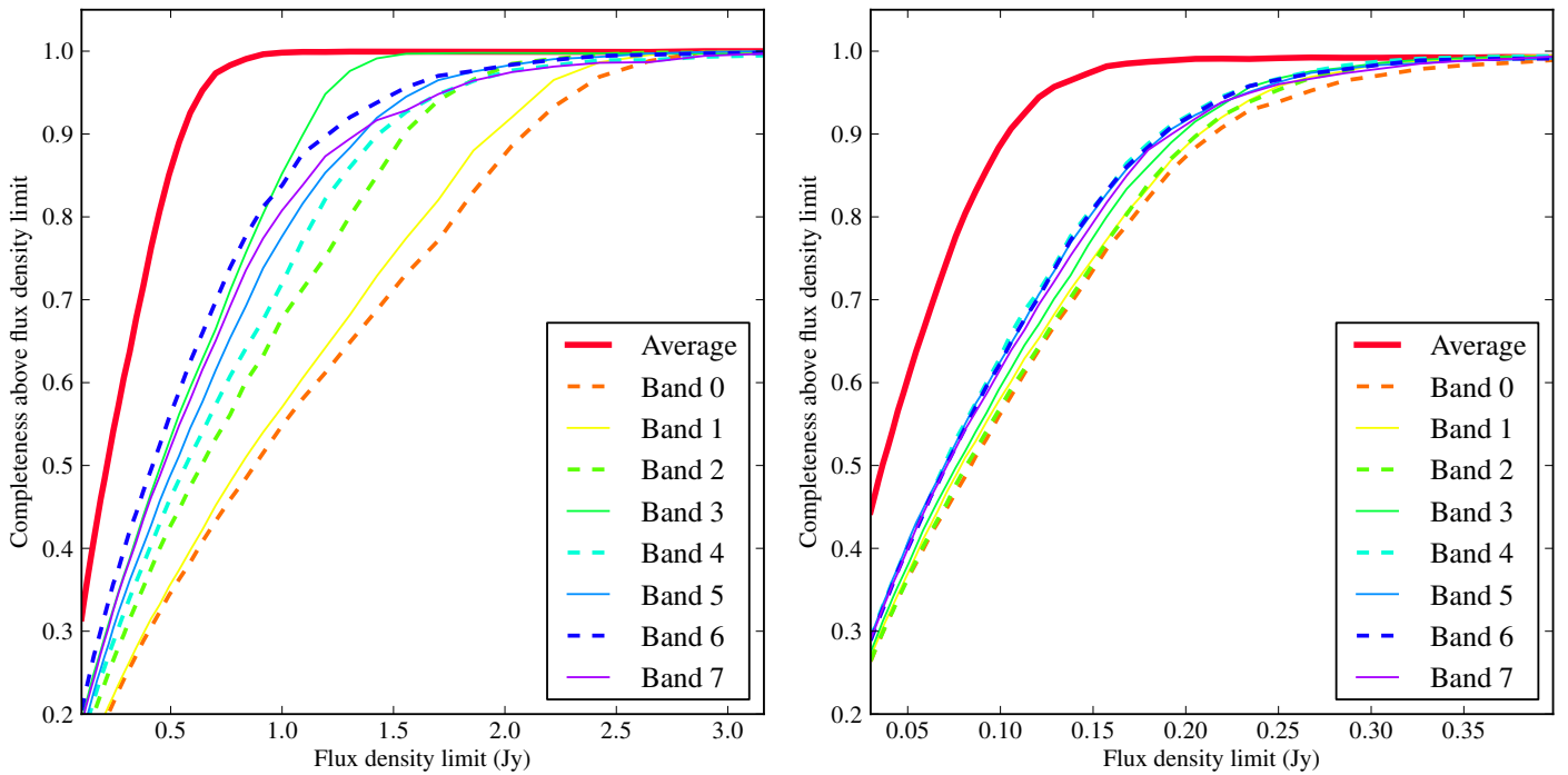
Fig. 13. Results of completeness simulations for LBA (left) and HBA (right). Curves show the cumulative completeness for the individual frequencies in the LBA and HBA and for their combination at a nominal reference frequency of 50 and 135 MHz, respectively.
