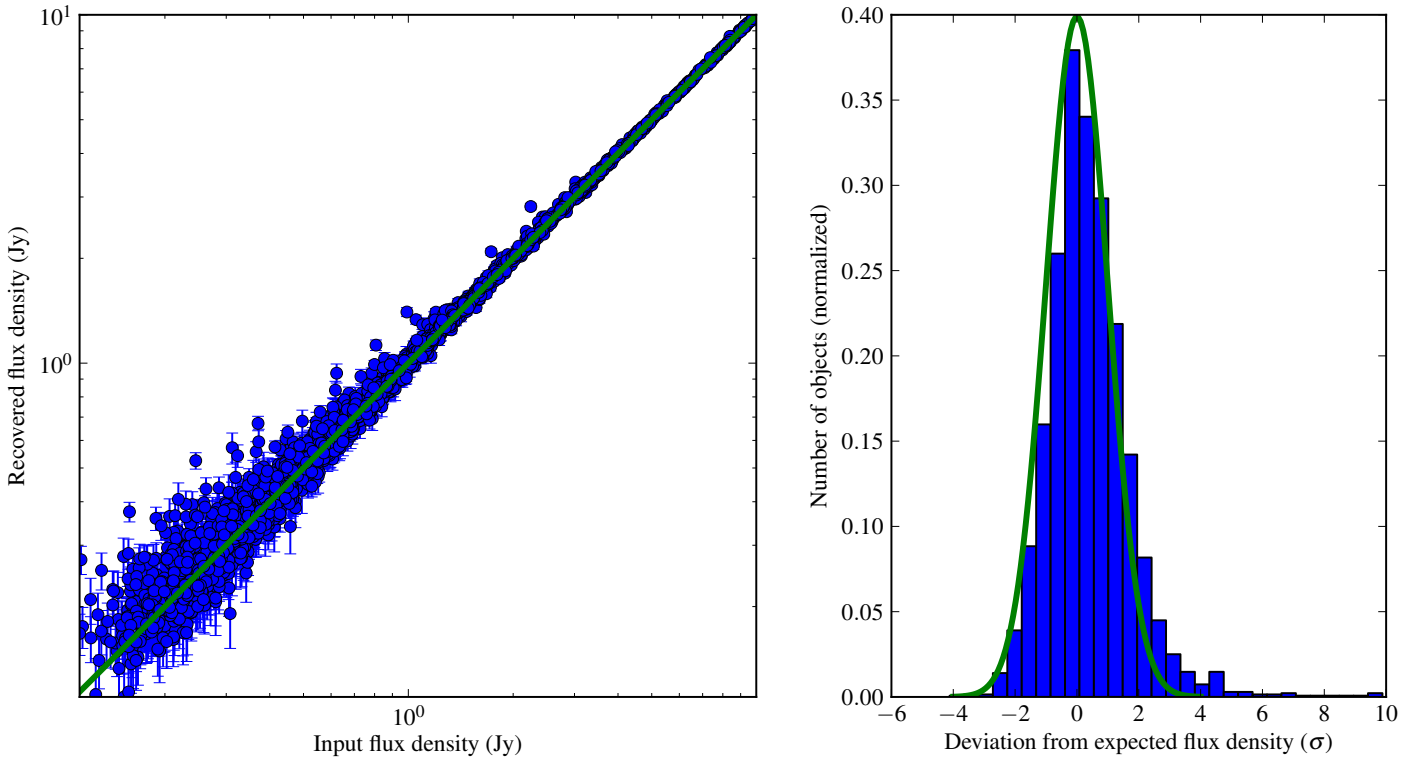
Fig. 14. Comparison of input and output model source flux densities for one band of the HBA (left) and histogram of the deviation from the expected value (right). The green line on the left shows the line of equality, on the right the expected normal distribution if the fluxes are simply affected by the noise estimated from the fit.
