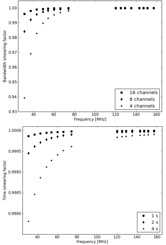
Fig. 7. Bandwidth ( top ) and time ( bottom ) smearing factors relevant to LOFAR MSSS observations, expressed as percentages and where unity is equivalent to no smearing. These values are calculated for 2' angular resolution and for sources at the half-power point of the station beam. In the top panel, points are plotted for averaging single subbands to 4 ( stars ), 8 ( diamonds ), and 16 ( squares ) channels. In the bottom panel, the smearing is calculated for visibility time averaging intervals of 1 ( squares ), 2 ( diamonds ), and 4 ( stars ) seconds.
