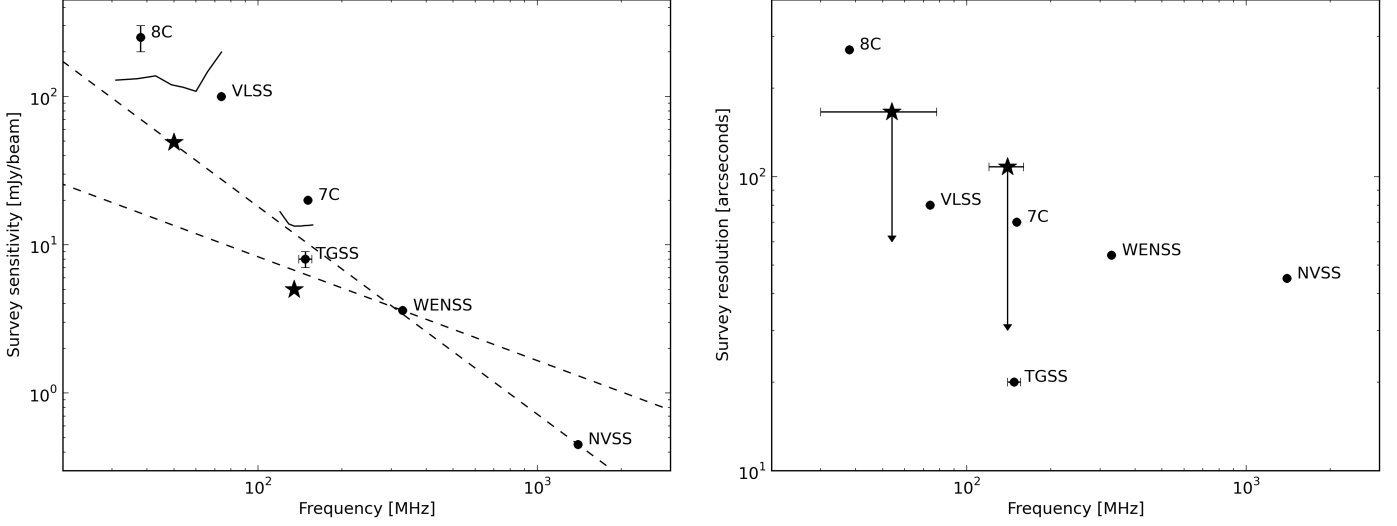
Fig. 17. Comparisons between MSSS sensitivities ( left ) and resolutions ( right ) with those of other existing radio surveys as summarized in Table 4. In the lefthand panel, dashed lines indicate representative spectral indices of \alpha = -0.7 and \alpha = -1.4 . The solid black lines illustrate the frequency dependence of the sensitivity in the 8 bands in each of the LBA and HBA survey segments, while the black stars show the frequency-averaged sensitivity demonstrated in § 5. In the righthand panel, the downward-pointing arrows indicate that the angular resolution of the initial MSSS catalog is limited with respect to the capabilities of the visibility data. Processing the full array will improve the survey performance.
