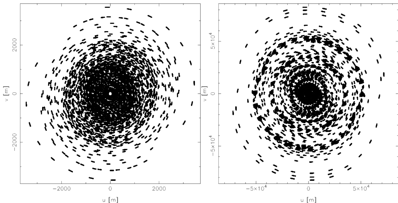
Fig. 2. The uv coverage for the MSSS-LBA field L227+69, core only (left) and all Dutch stations (right).
