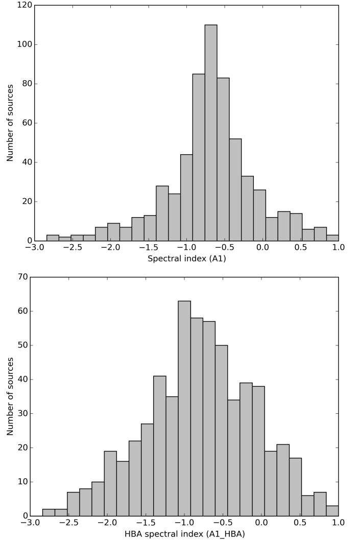
Fig. 12. Spectral index histograms for the MVF catalog sources with A0_{\text{HBA}} > 0.2 Jy, based on the cataloged A1 values ( top ), and the same but for HBA values only, catalogued as A1_HBA ( bottom ).
