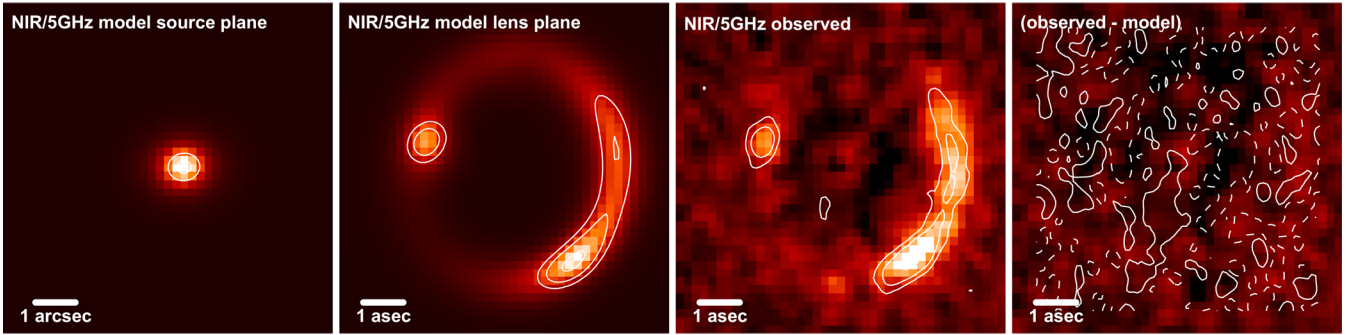
Figure 6. Mass modelling results based on joint fitting of the near-infrared imaging (colour map) and 5 GHz imaging (shown as contours at levels of 0.0033 \times (3.9, 27) mJy beam ^{-1} ). Left: source plane model (centre left) the reconstructed image in the lens plane with the lensing galaxies G1 and G2 subtracted, (centre right) observed data linearly scaled between -3\sigma and 10\sigma , (right) residual (observed–model). The residual colour scale (near-infrared) is the same as the previous panel and the contours are at levels of 0.0033 \times (-1, 1) mJy beam ^{-1} . Images are orientated north up, east left.
