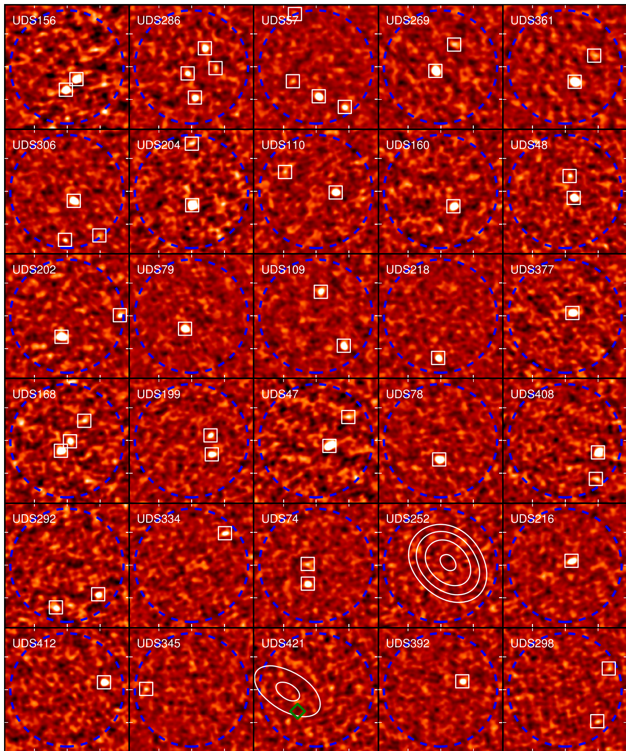
Figure 1. ALMA 870\ \mu\text{m} continuum maps, at 0''.8 resolution, of 30 bright sub-mm sources in the UDS field. These sources are selected to be representative of the brightest sources detected in the S2CLS survey of this \sim 0.8\ \text{deg}^2 field. The 18'' \times 18'' non-primary-beam-corrected maps (roughly 150\ \text{kpc} \times 150\ \text{kpc} at the typical SMG redshift, z = 2.5 ) are ordered by decreasing single-dish flux density and have a median 1\text{-}\sigma rms of 0.26\ \text{mJy beam}^{-1} . The dashed circle on each thumbnail represents the primary beam (FWHM) of ALMA at 870\ \mu\text{m} . We detect 52 SMGs at >4\sigma (marked by a squares) in the 30 ALMA maps, with 870\ \mu\text{m} flux densities of 1.3\text{--}12.9\ \text{mJy} . In 18/30 ALMA maps the single-dish sub-mm source fragments into two or more individual SMGs. In particular, we highlight UDS 57, 168, 286 and 306, where the ALMA observations demonstrate that the single-dish source is comprised of three-or-four SMGs. In two ALMA maps, UDS 252 and 421, we do not detect any SMGs, but note that both SCUBA-2 sources are detected in Herschel /SPIRE imaging. We plot contours representing the single-dish SCUBA-2 emission at 3, 3.5, 4.0, 4.5 \times \sigma for these sources, note that UDS 421 has a potential VLA/1.4 GHz counterpart (diamond; Arumugan et al. submitted) that is not detected in our ALMA maps.
