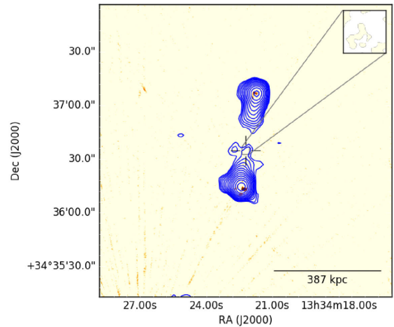
(ah) J133422.15+343640.5
