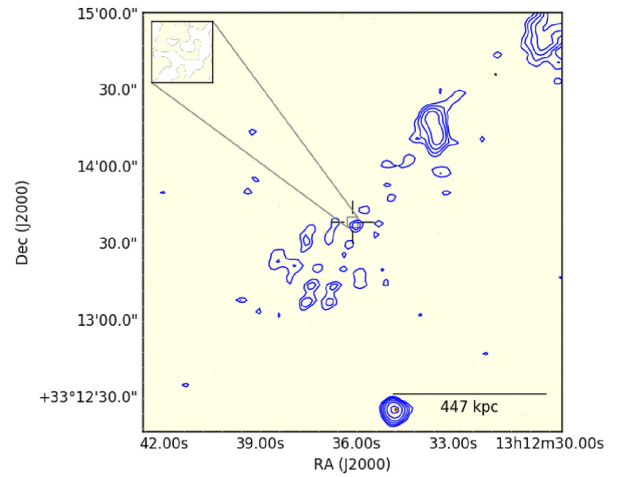
(t) J131235.35+331348.6
