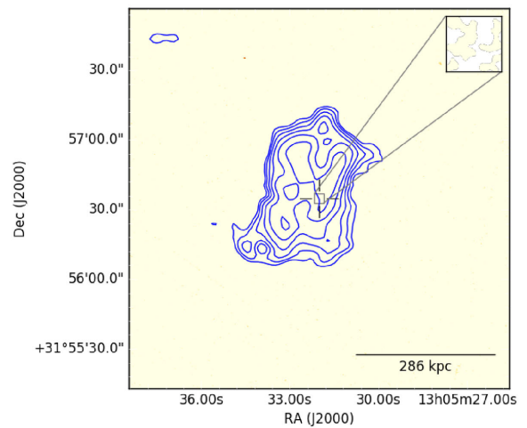
(j) J130532.49+315639.0
