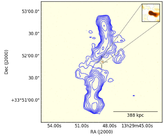
(ad) J132949.25+335136.2
