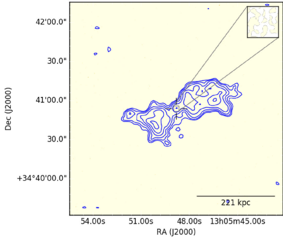
(k) J130548.65+344052.7
