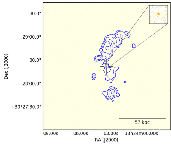
(z) J132402.51+302830.1
