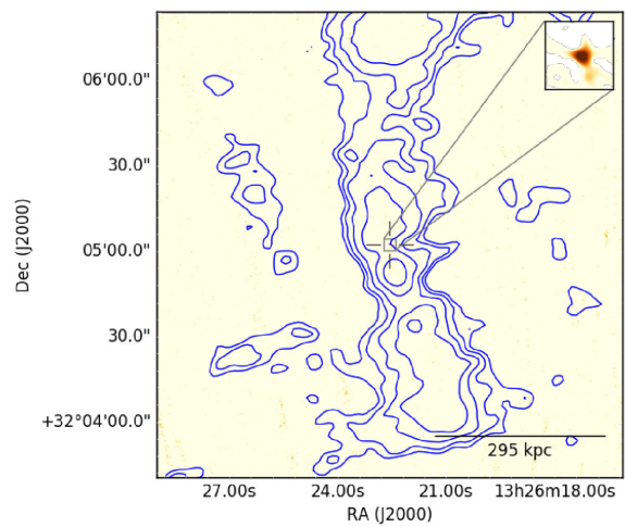
(ab) J132622.12+320512.1 †
