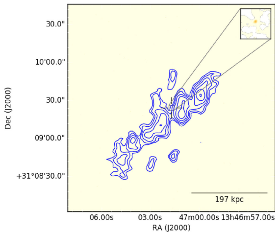
(ak) J134702.03+310913.3
