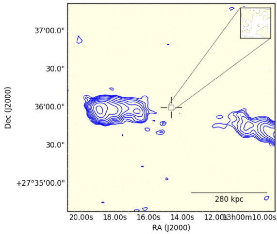
(g) J130013.55+273548.7
