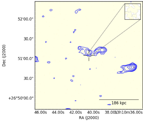
(s) J131039.92+265111.9
