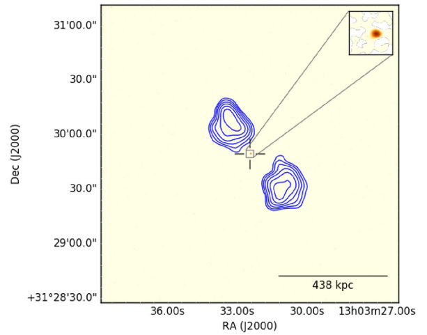
(h) J130332.38+312947.1
