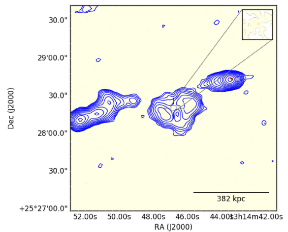
(v) J131446.57+252819.8
