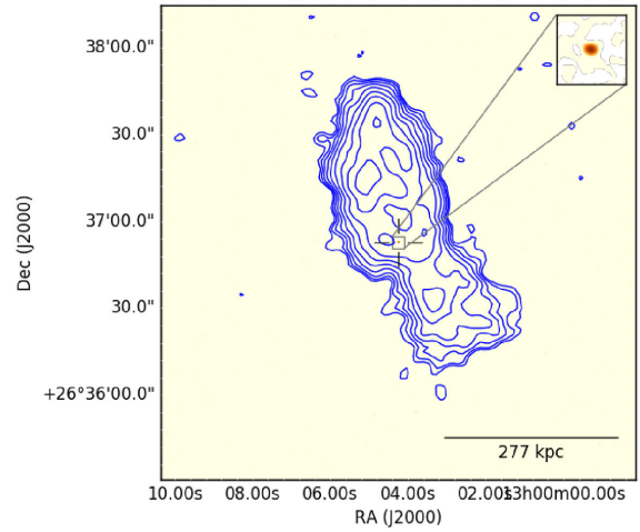
(f) J130003.72+263652.1
