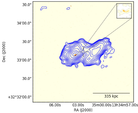
(ai) J133502.36+323312.8
