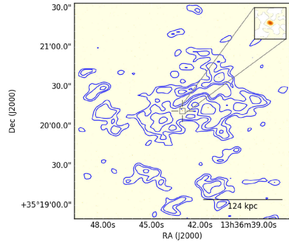
(aj) J133642.53+352009.9
