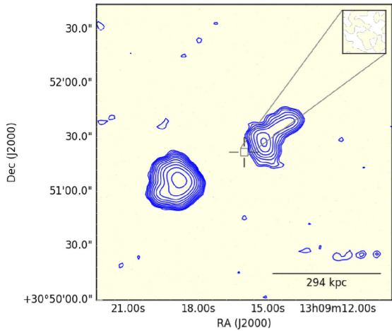
(o) J130916.85+305118.3
