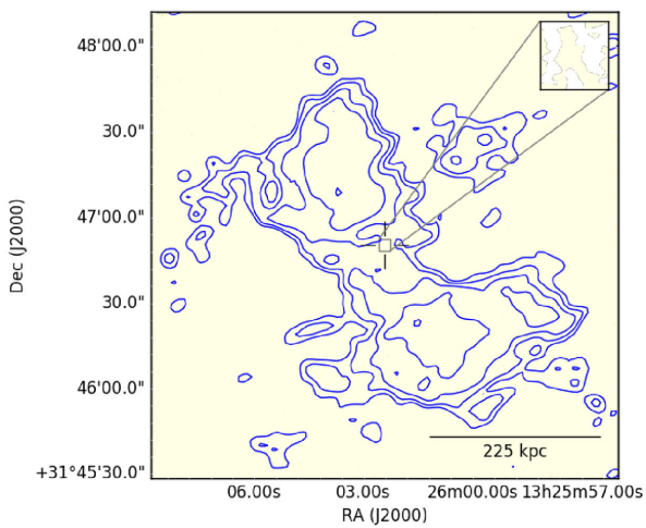
(aa) J132602.06+314645.6 †
