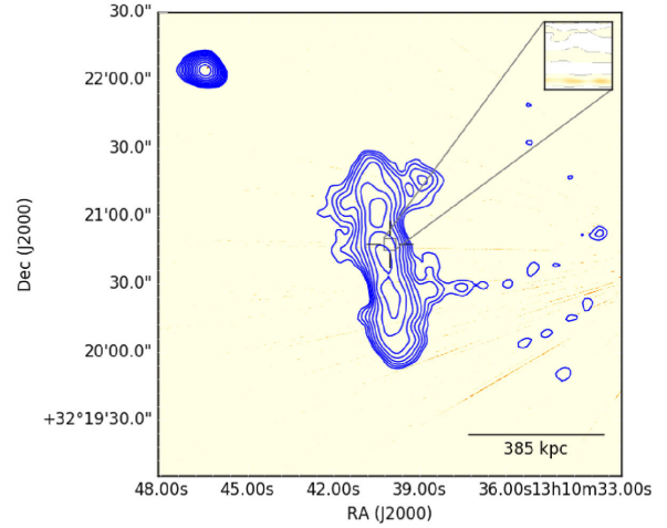
(r) J131040.25+322044.1
