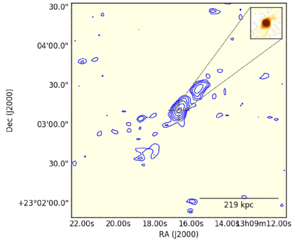
(p) J130915.61+230309.5
