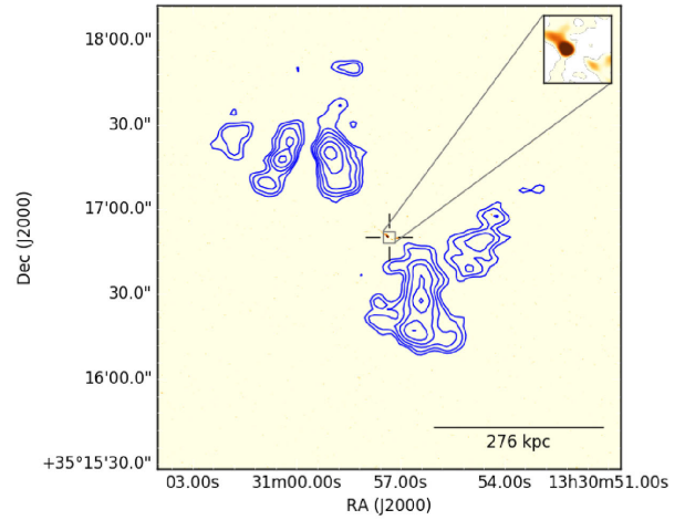
(af) J133058.91+351658.9
