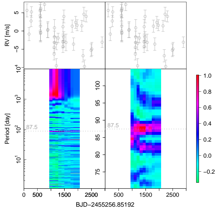
Figure 20. Moving periodogram for HIP 71135 b. The window size is 2000 days and the number of steps is 10. The annual alias of 87.5 day also show excess power in the bottom right panel.
