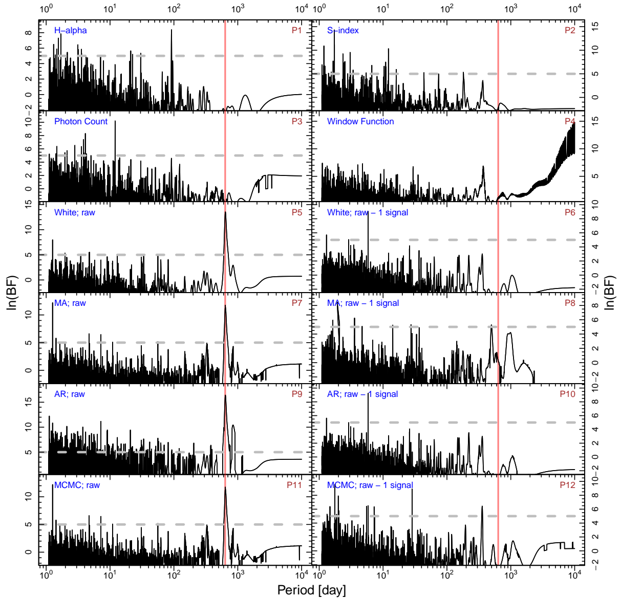
Figure 12. BFPs for HD 164604. The red line shows the signal at a period of 635 days.
