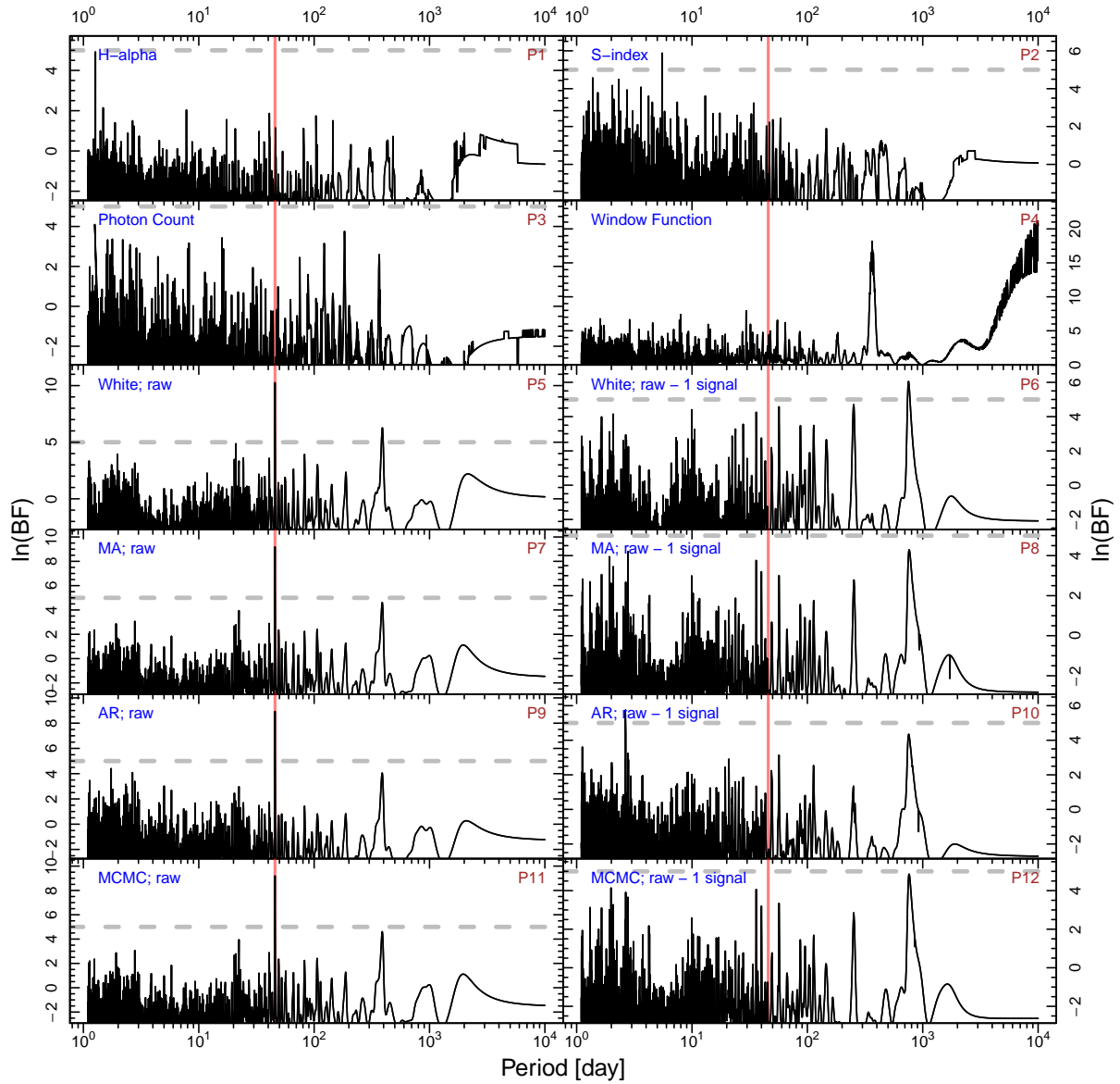
Figure 10. BFPs for HD 64114. The red line shows the signal at a period of 45.8 days.
