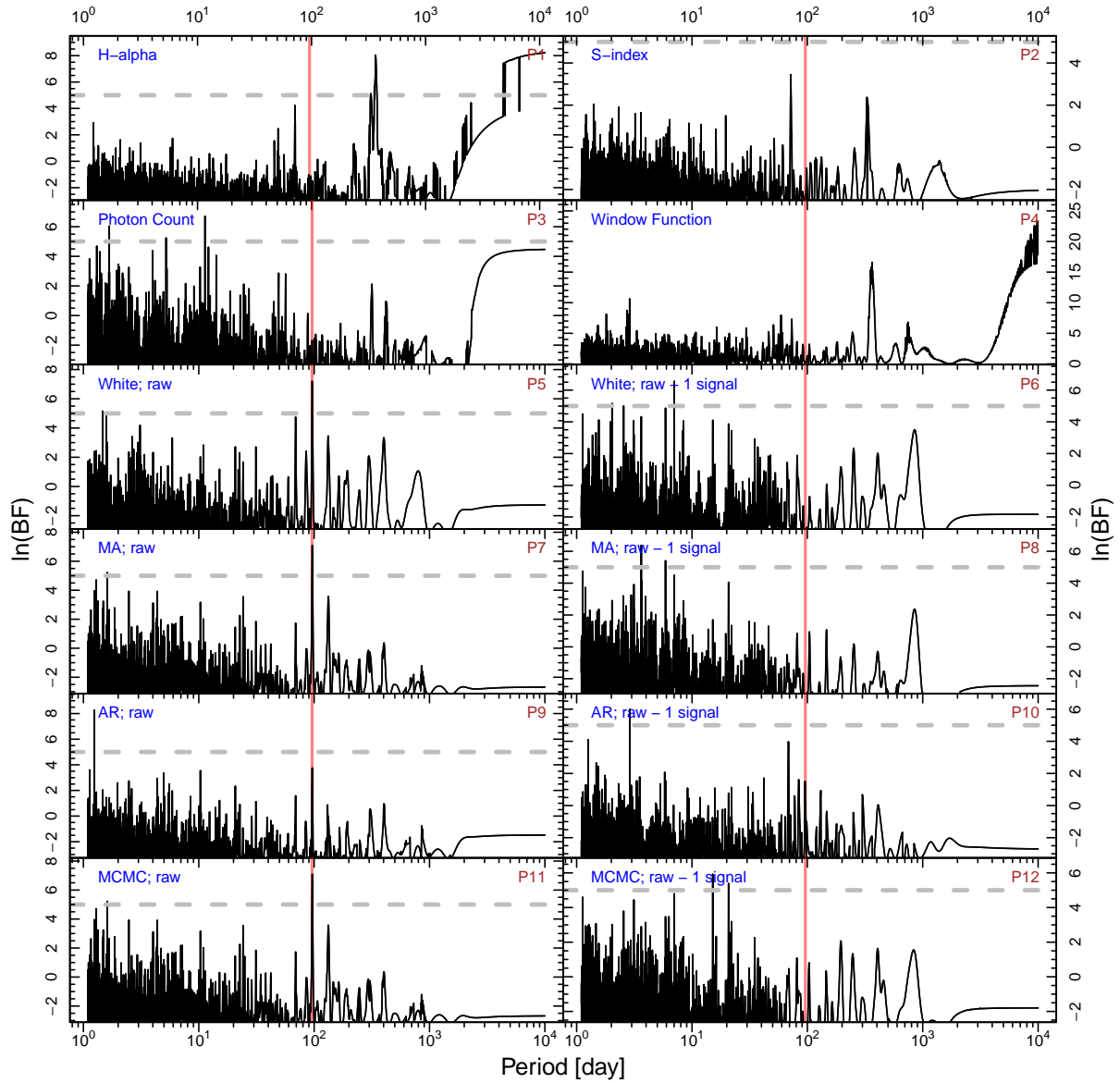
Figure 8. BFPs for HD 206255. The red line shows the signal at a period of 96.0 days.
