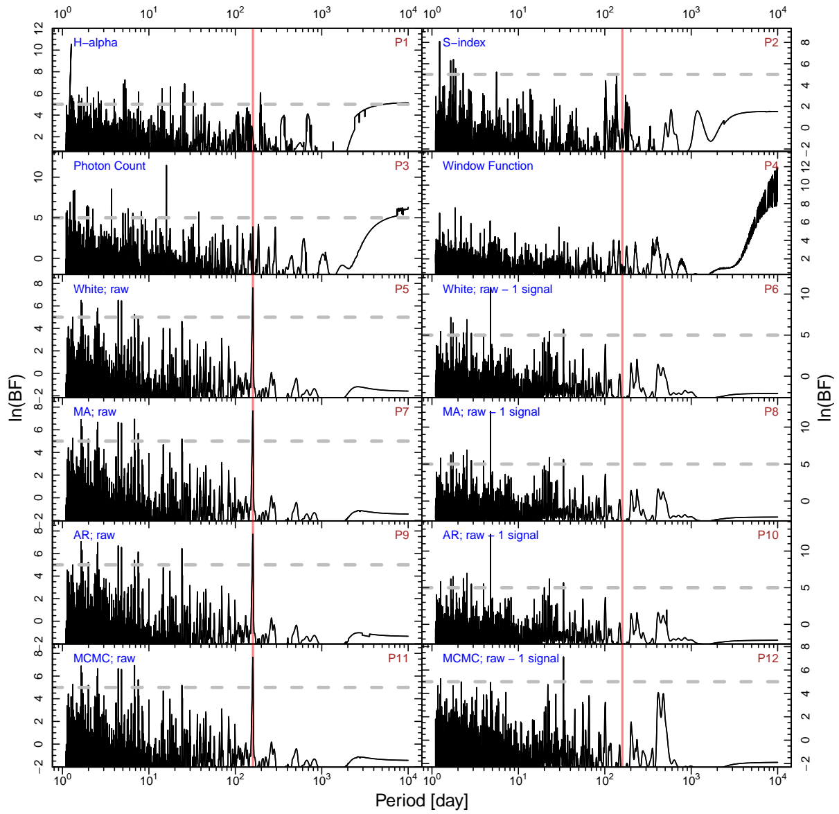
Figure 11. BFPs for HD 8326. The red line shows the signal at a period of 159 days.
