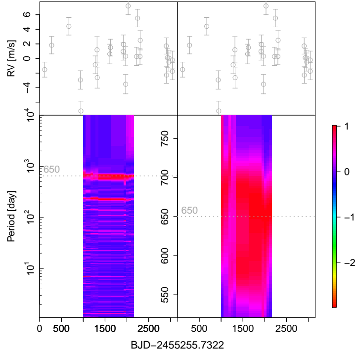
Figure 16. Moving periodogram for the PFS data for HD 210193. The top panels show RV data. The bottom right panel is a zoom-in version of the bottom left panel which shows the color-coded 2-dimensional BFP. The x axis is the BJD time relative to the first epoch. The periodogram power is normalized for each moving time window so that the BF does not depend on the number of RVs in each window. A global color coding is applied to these normalized BFs. The time span of each time window is 2036 days. The window move to cover the full data set within 20 steps. In the calculation of BFPs, we ignore the eccentricity of signals. This is not likely to change the time-consistency of MCMC signals although such assumption may alternate signal period and amplitude slightly.
