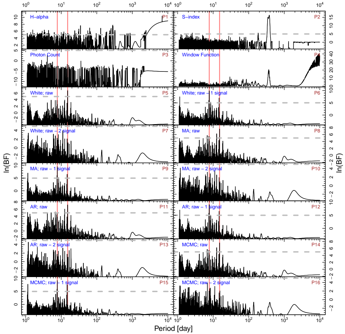
Figure 13. BFPs for HIP 54373. The red lines show the signals at periods of 15.1 and 7.76 days.
