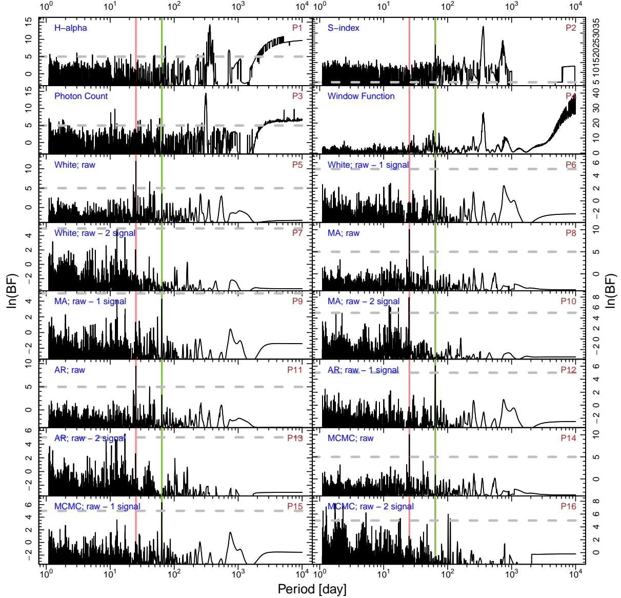
Figure 3. BFPs for HD 211970. The red line shows the Keplerian signal at a period of 25.2 days while the green line shows the 64.0 day activity signal.
