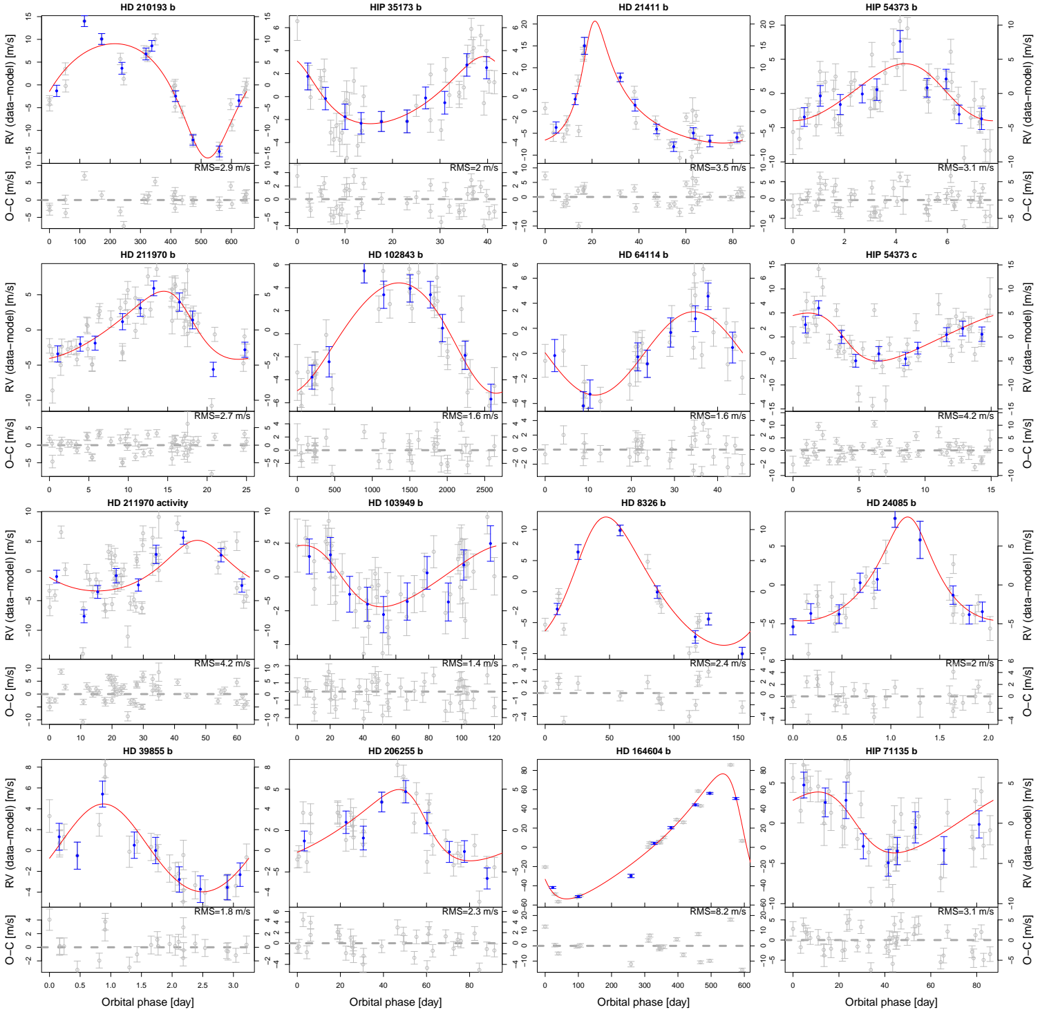
Figure 2. Phase curve and corresponding residuals for all planet candidates. The blue error bars show the error-weighted average RVs in 10 bins. The best orbital solution is determined by the MAP values of orbital parameters. The Root Mean Square (RMS) of the residual RVs is shown in each panel.
