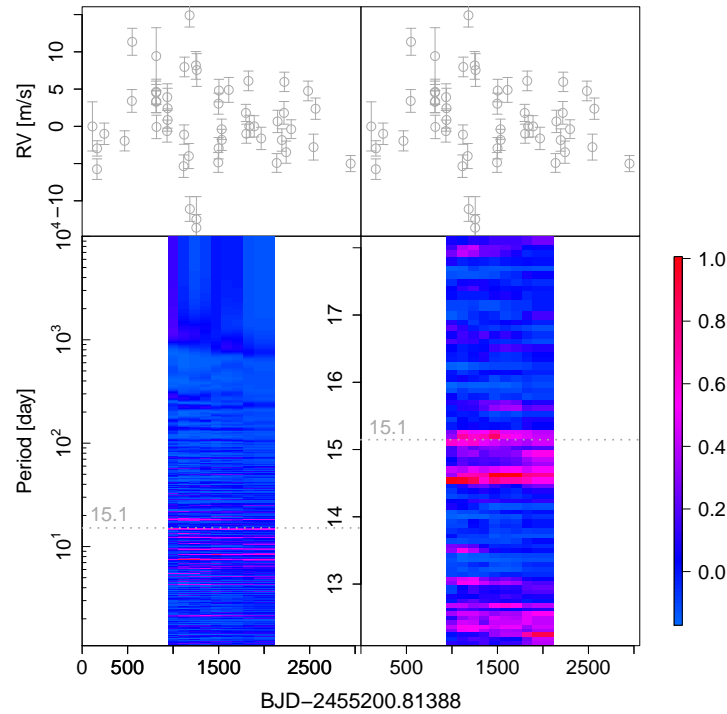
Figure 18. Moving periodogram for HIP 54373 c. The window size is 2000 days and the number of steps is 10. The signal near the 15.1 day signal is its annual alias.
