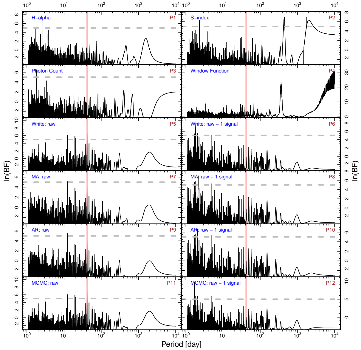
Figure 5. BFPs for HIP 35173. The red line shows the signal at a period of 41.5 days.
