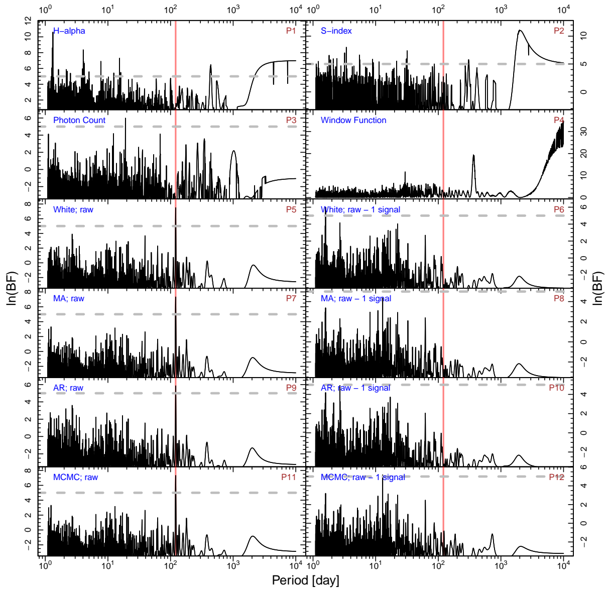
Figure 7. BFPs for HD 103949. The red line shows the signal at a period of 121 days.
