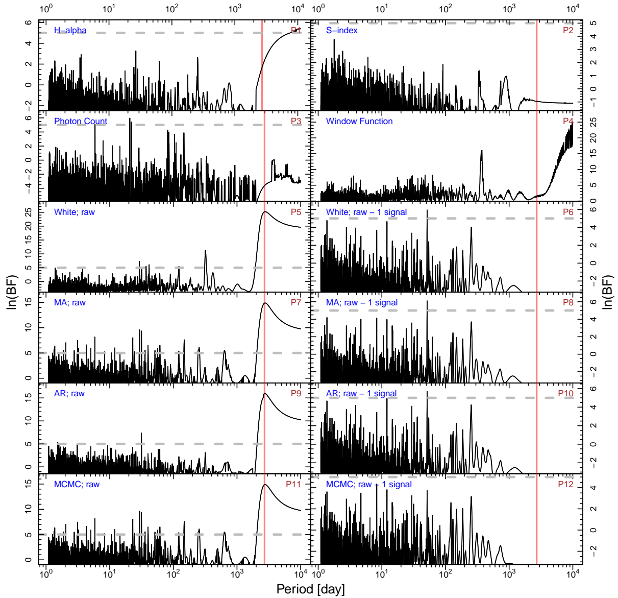
Figure 6. BFPs for HD 102843. The red line shows the signal at a period of about 3000 days.
