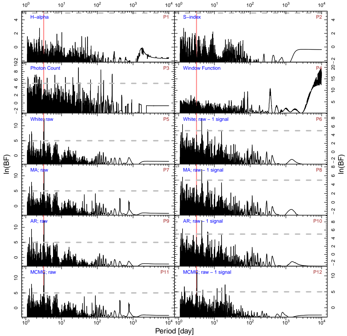
Figure 4. BFPs for HD 39855. The red line shows the signal at a period of 3.25 days.
