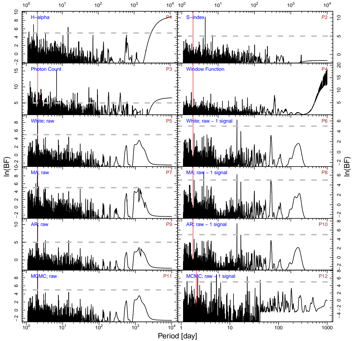
Figure 14. BFPs for HD 24085. The red line shows the signal at a period of 2.05 days.
