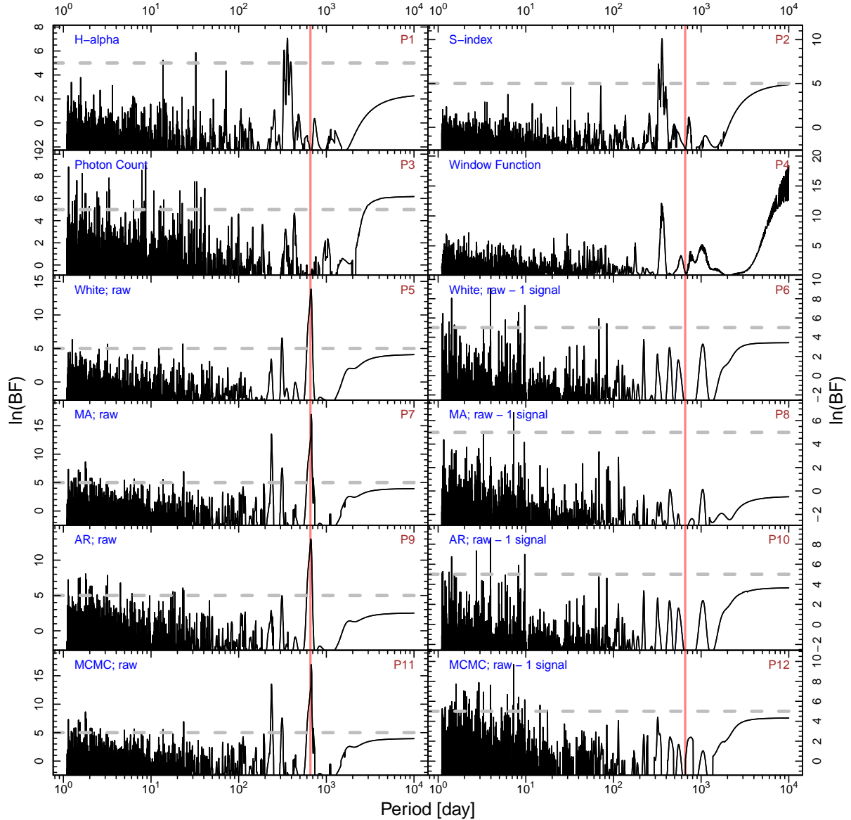
Figure 1. BFPs for HD 210193. The BFPs are calculated for the activity indices, and for the white noise model, MA(1), and AR(1) for the raw RV data and RVs with sinusoidal signals subtracted. The BFPs for activity indices are calculated using the MA(1) model. The window function is calculated using the Lomb-Scargle periodogram (Lomb 1976; Scargle 1982). The activity indices, window function, noise models and data sets are shown in the top left corners. Each panel is denoted by “Px” in the top right corner where “x” is a natural number. The RV signal at a period of 650 days is marked by the red vertical lines. The panels denoted by “MCMC” show the BFPs for the raw data subtracted by the best-fit Keplerian signals constrained by MCMC. The grey dashed line denotes the \ln(\text{BF})=5 criterion in each BFP. The elements in this figure are also applicable for the subsequent figures. The signals in the residual BFPs are either noise-model dependent or not identified as significant signals through MCMC sampling.
