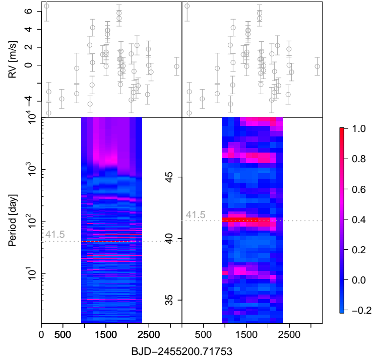
Figure 19. Moving periodogram for HIP 35173 b. The window size is 2000 days and the number of steps is 10. The other signals in the bottom right panel are the annual aliases of the 41.5 day signal.
