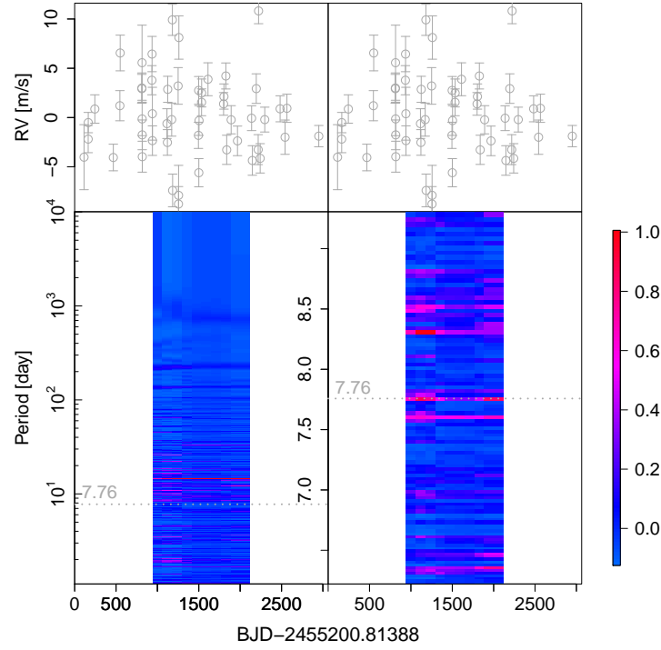
Figure 17. Moving periodogram for HIP 54373 b. The window size is 2000 days and the number of steps is 10. The signal near the 7.76 day signal is its annual alias.
