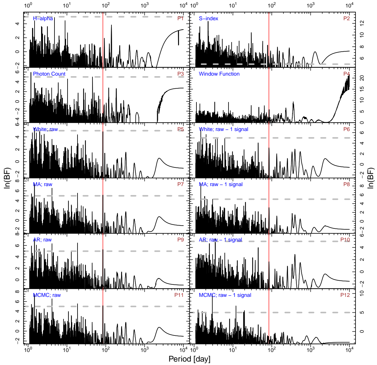
Figure 9. BFPs for HD 21411. The red line shows the signal at a period of 84.3 days.
