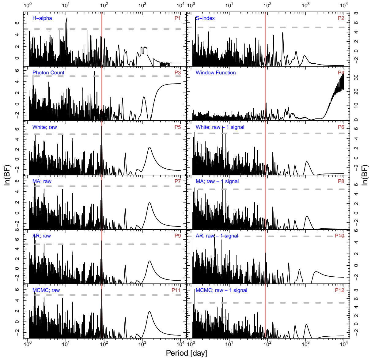
Figure 15. BFPs for HIP 71135. The red line shows the signal at a period of 87.2 days.
