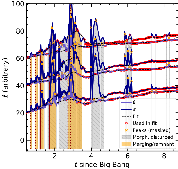
Figure 2. Plot illustrating our method for determining when an object is morphologically disturbed. Light and dark blue lines show the major and minor axes of the galaxy in 3 different projections (with arbitrary normalisation), red points show the points used to fit the continuum and the black line indicates the fit with the shaded region indicating the standard deviation of the residual. Yellow crosses show the detected peaks which were masked out from the fit and grey and orange shaded regions show the times that the galaxy is determined to be disturbed and disturbed as the result of a merger respectively.
