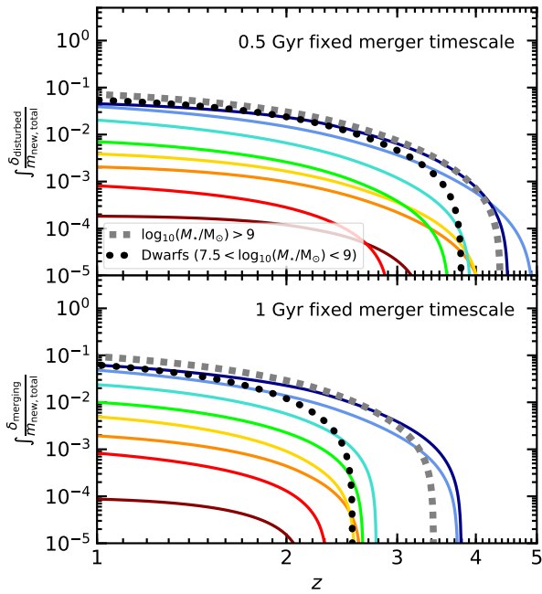
Figure C2. Version of Fig 12 using a fixed merger timescale of 0.5 Gyrs (top panel) and 1 Gyr (bottom panel).
