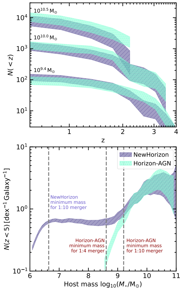
Figure A1. Top: Cumulative number of mergers occurring as a function of redshift for bins of stellar mass for the NEWHORIZON (blue) and Horizon-AGN (aquamarine) simulations. Shaded regions show the 1\sigma confidence interval for the cumulative number of mergers as a function of redshift and the centre of each 0.5 dex wide stellar mass bin is indicated above each region. Values on the y-axis are arbitrary and each bin is separated by an arbitrary amount Bottom: Total number of mergers undergone since z = 5 as a function of stellar mass of the primary at the time of the merger and normalised by the total number of galaxies in the stellar mass bin.
