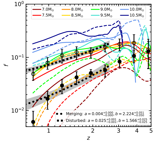
Figure 5. Fraction of galaxies that are morphologically disturbed at a given redshift (solid lines) and morphologically disturbed as the result of mergers with mass ratios greater than 1 : 10 . Colours indicate the z = 0.5 progenitor mass and thick dotted lines indicate the average fractions across all masses. Error bars with open and filled circles indicate average fractions for disturbed and merging fractions for the dwarf regime ( 7.5 < \log_{10}(M_{\star}/M_{\odot}) < 9 ), lines dotted with squares and circles indicate the best fitting parameters to the function f = a(1+z)^b using these data points and shaded regions indicate the 1\sigma uncertainty. Error bars and model uncertainties are both multiplied by 10 for legibility.
