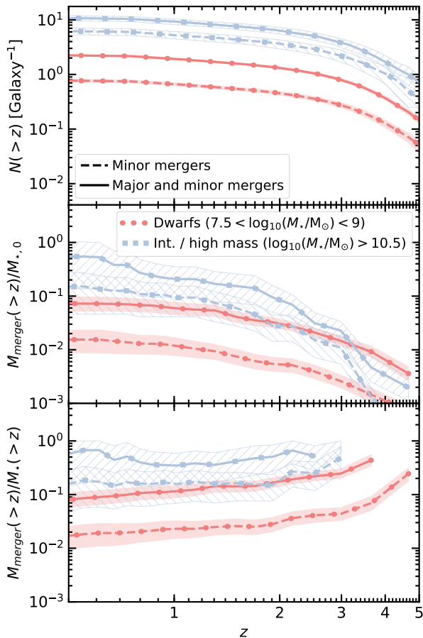
Figure 10. Top: cumulative number of minor (dashed line) and total number of mergers with mass ratios greater than 1 : 10 per galaxy for dwarfs (light red lines) and intermediate mass galaxies (light blue lines). Middle: cumulative mass accreted from minor and 1 : 10 or greater mass ratio mergers as a fraction of the total stellar mass at z = 0.5 . Bottom: ratio of the cumulative accreted mass and cumulative total stellar mass. Shaded regions and hatched regions show the 1\sigma uncertainties.
