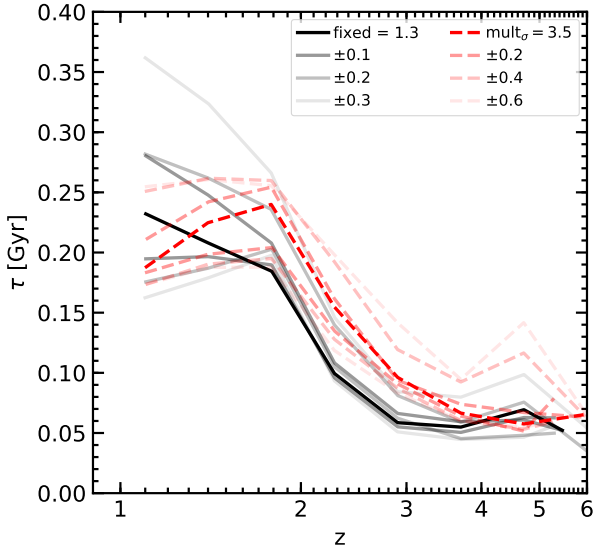
Figure C1. Evolution of median major merger durations as a function of redshift for different input parameters. Red dashed lines indicate merger timescales when we use a threshold based the multiple of \sigma_{\text{local}} that axis lengths are allowed to vary from the continuum fit before they are considered morphologically disturbed. Black solid lines indicate the same but using a fixed threshold rather than one that varies with \sigma_{\text{local}} . Lighter lines show how merger durations vary for small changes in the threshold.
