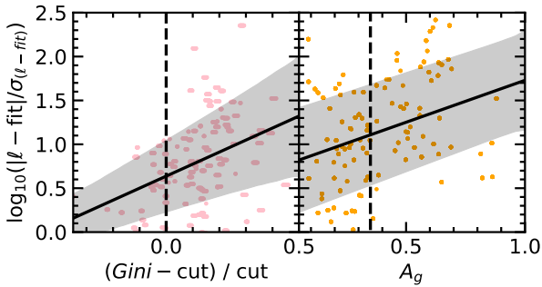
Figure B1. The residual between the smoothed continuum fit of the axis length and the actual evolution of the axis length as described in Section 2.4 vs the distance above the Gini-M_{20} cut (left) and shape asymmetry (right). The black lines show a first order polynomial fit to the data and the shaded region shows the standard deviation of the residual. The dashed lines indicate the threshold above which galaxies are considered to be merging.
