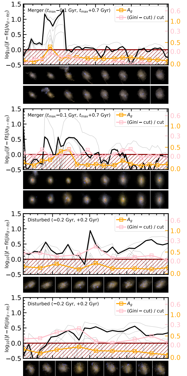
Figure 3. The top part of each panel shows the residual of the axis lengths and continuum for each axis and second highest value of the residual (thin and thick black lines respectively), A_g (yellow) and the distance of the Gini coefficient above the Gini-M_{20} cut (pink). y-axes are scaled so the red hatches enclose a region where the galaxy is relaxed according to our criteria, A_g and Gini-M_{20} . Bottom panels show u-r-z images in chronological order (top to bottom / left to right), the position of each image corresponds roughly to the time in the plot above. The top two panels show mergers between 100 Myr and 700 Myr before and after t_{\text{max}} . The bottom two panels show morphologically disturbed galaxies for \pm 200 Myr.
