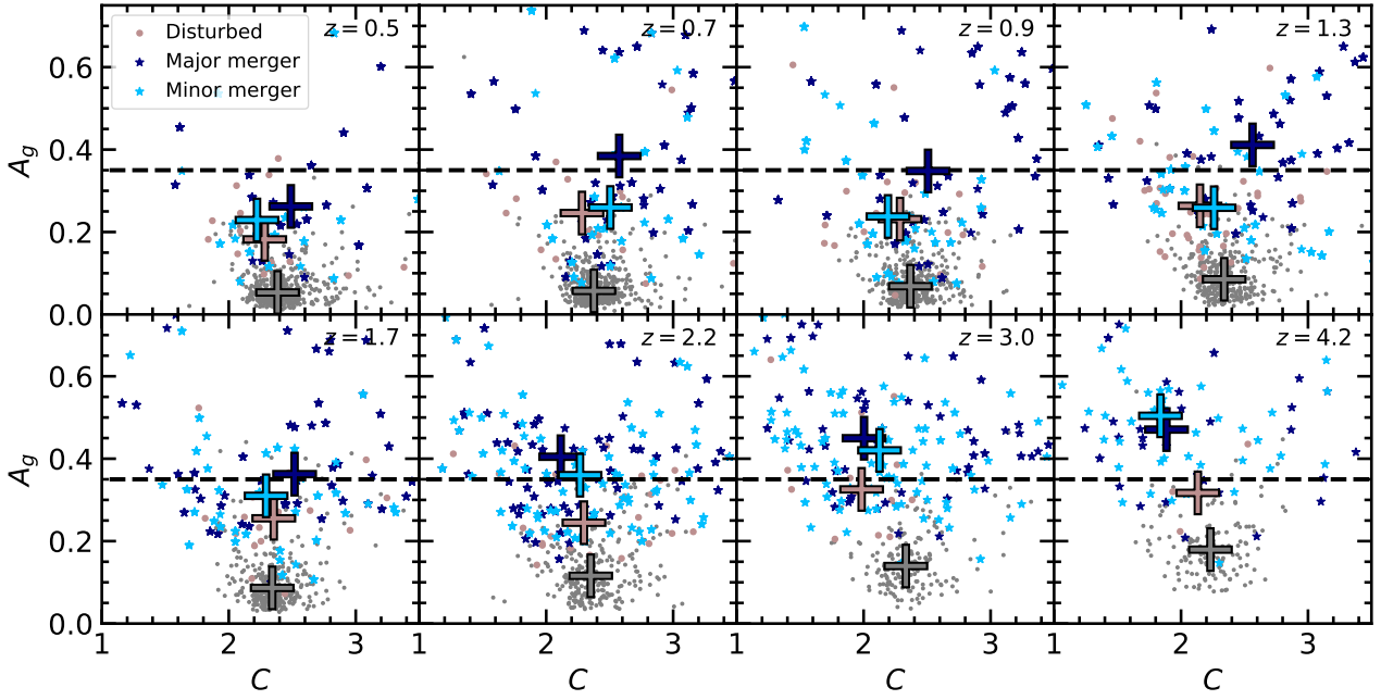
Figure B2. Shape asymmetry vs concentration for galaxies at different redshift snapshots. Dark blue and light blue stars indicate galaxies that undergoing either major or minor mergers, light red points indicate morphologically disturbed galaxies and grey points indicate galaxies that are neither merging or morphologically disturbed. Large coloured crosses indicate the mean position of each sample.
