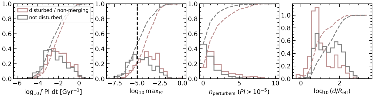
Figure A2. Histograms show the distribution of Left : the integrated perturbation index; Centre left : the largest instantaneous PI contributed by any individual galaxy; Centre right : the total number of galaxies that contribute a PI greater than \sim 10^{-5} ; Right : the minimum separation from another galaxy with a mass ratio of at least 1:10 for the disturbed and mass-matched non-disturbed samples. Light red histograms indicate the distribution of quantities of the non-merging disturbed sample and grey histograms indicate the distribution of quantities of the non-disturbed sample. Dotted lines indicate the cumulative distribution.
