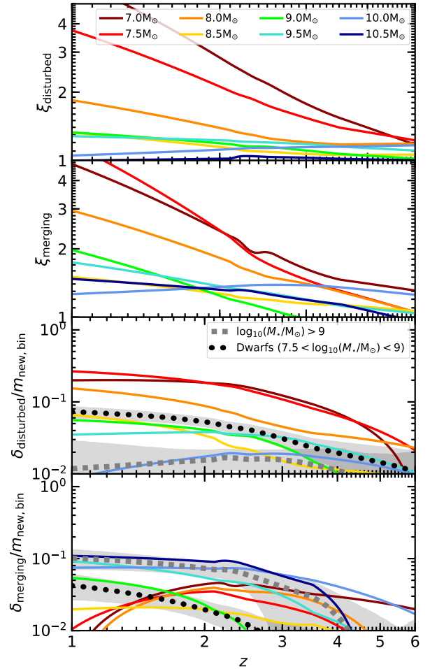
Figure 11. The first and second panels show the average fractional enhancement in sSFR for disturbed (interacting) galaxies and merging galaxies compared to the non-disturbed population in bins of progenitor stellar mass. The third and fourth panels show the fractional SFR excess due to interactions and mergers respectively. Coloured lines indicate the evolution of each quantity with redshift for different stellar masses and lines dotted with black circles and grey squares show the average excess due to interactions or mergers for dwarf masses and M_* > 10^9 M_{\odot} respectively weighted by the stellar mass formed in each bin.
