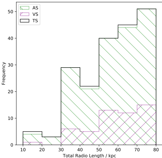
Figure 4. Distribution of total radio emission lengths for the TS, AS and VS.
