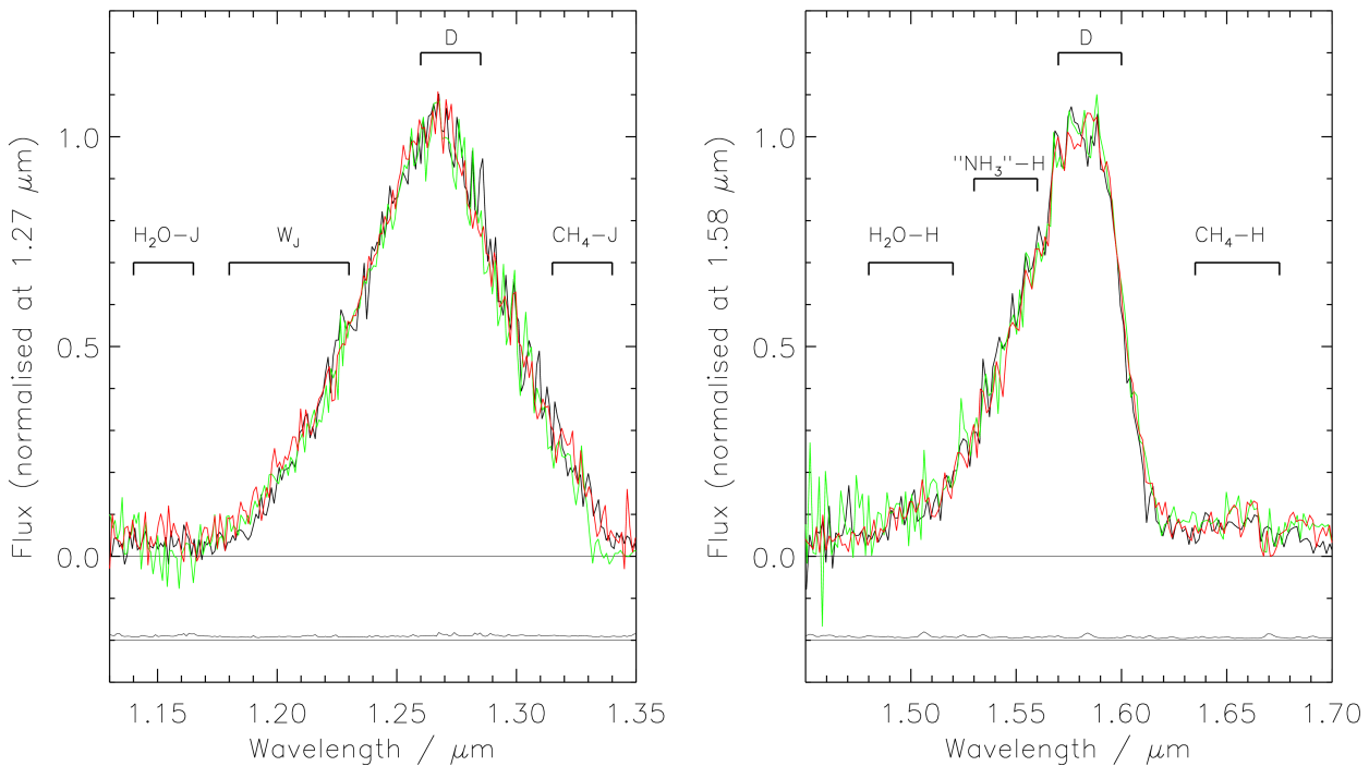
Figure 5. The J and H -band flux peaks of ULAS1335 (black line), ULAS0034 (T9, see text; green line) and CFBD50059 (T9, see text; red line). The black line that is plotted offset by -0.2 in the y-axis is the error spectrum for ULAS1335. Also indicated are the spectral regions integrated to form the numerator of the spectral indices discussed in the text. The region that forms the denominator is indicated with the letter “D”.
