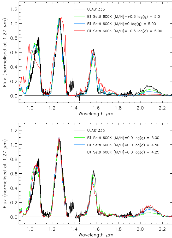
Figure 13. A comparison of model spectra with ULAS1335 for differing gravity and metallicity combinations at T_{\text{eff}} = 600\text{K} .
