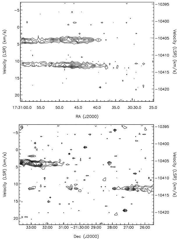
Figure 6. High-resolution ^{12}\text{CO} (J=2-1) spatial-velocity maps of the region surrounding Kepler's SNR. Top: R.A.-velocity map with contours starting at 0.04 K and incrementing by 0.03 K. Bottom: Dec.-velocity map with contours starting at 0.07 K and incrementing by 0.03 K.
