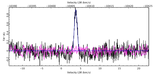
Figure 7. ^{12}\text{CO} (J=2-1) high-resolution spectra (black) observed at the location listed in Table 1 over the velocity range -14 < v < 23 \text{ km s}^{-1} . The corresponding ^{13}\text{CO} (J=2-1) spectra are shown in purple. The peak CO emission is < 1 with velocity widths \Delta v < 1 \text{ km s}^{-1} .
