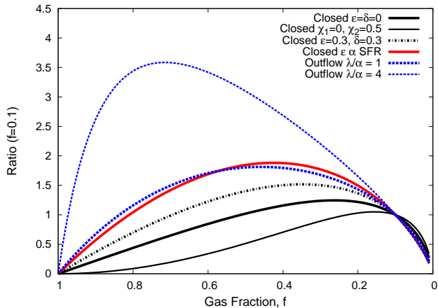
Figure 24. Ratio ( R ) of dust mass at gas fraction f to that at f = 0.1 (today). The models are (i) a closed box with no gas entering/leaving the system with dust from both supernovae \chi_1 = 0.1 and LIMS stars \chi_2 = 0.5 (thick solid; black); (ii) with dust from LIMS only \chi_1 = 0 , \chi_2 = 0.5 (thin solid; black); (iii) including mantle growth (dot-dashed; black); (iv) A model with mantle growth proportional to the SFR (solid; red). (v) and (vi) A model which has outflow with gas lost at a rate proportional to one or four times the SFR ( \lambda/\alpha = 1 (dotted; blue)). It is worth noting that for higher returned fraction from stars to the ISM (i.e. \alpha = 0.5 ), the ratio decreases for all models ( R < 3 for the extreme outflow).
