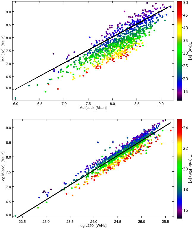
Figure 6. Top: Comparison of dust masses from the DCE08 model ( M_{\text{sed}} ) versus the dust mass obtained by using the isothermal grey body fit ( M_{\text{iso}} ) using Eq. 3. Points are colour-coded by the isothermal temperature. The one-to-one line is shown in black. There is a large difference between the two mass estimates which is a strong function of fitted isothermal temperature. Bottom: Comparison of M_{\text{sed}} to L_{250} showing a reasonably tight and linear correlation. The best fit relationship (Eq. 4) is over-plotted. The scatter in this relationship is driven by the diffuse ISM dust temperature, which is used to colour-code the points.
