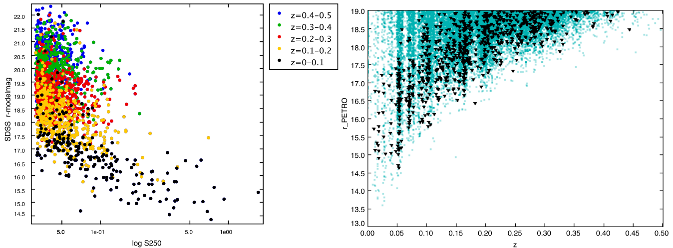
Figure 2. Left: SDSS r -modelmag as a function of 250\mu\text{m} flux. There is no strong correlation apart from at the brightest fluxes. Only 4 galaxies lie within 0.4 mag of the flux limit used for IDs ( r < 22.4 ) at z < 0.5 and so we consider that optical incompleteness is not a serious problem for this sample. Right: r -mag versus redshift for all sources in GAMA-9 (pale blue squares) and SPIRE IDs with R \geq 0.8 (black triangles). Herschel sources tend to be larger mass optical galaxies and so the SDSS flux-limit does not affect our ability to optically identify H-ATLAS sources until z \sim 0.5 . Note that the right panel uses the brighter limit of r < 19 appropriate for the GAMA redshift survey.
