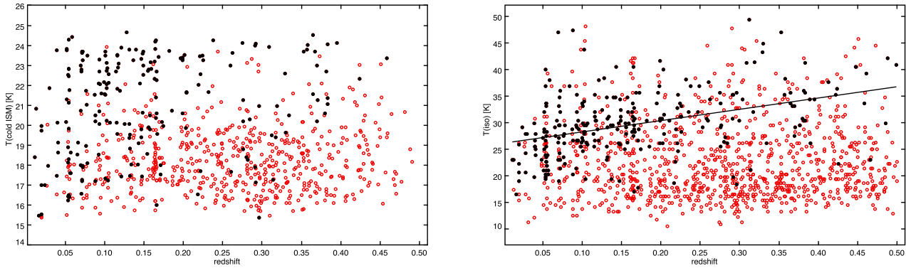
Figure 11. Left: Cold ISM temperature from the DCE08 fits versus redshift for sources with PACS detections (black filled) and which have 350\mu\text{m} fluxes above 3\sigma in additions to the 5\sigma 250\mu\text{m} flux (red open). Right: Same but for the isothermal temperature. Here there is a correlation between T_{\text{iso}} and redshift for the PACS detections ( r = 0.4 ).
