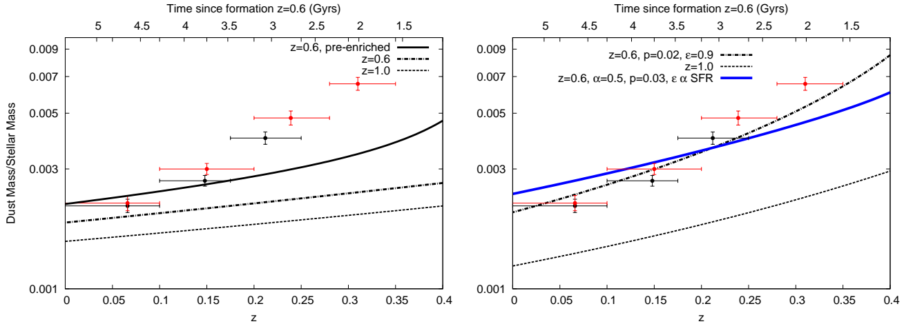
Figure 23. Left: The dust-to-stellar mass ratio as a function of redshift. Stellar and dust masses are derived from the SED fits using the models of DCE08 and are discussed in detail in Section 3 and Smith et al. (2011b). Black points show those sources with spectroscopic redshifts, while red points include photometric redshifts. Each sample is limited in redshift to the point where the optical flux limit is not biasing the selection to low dust-to-mass ratios. The model lines for the dust model (Section. 6.1) corresponding to the Milky Way including mantle growth and destruction are over-plotted with formation redshifts of z = 0.6 (dot-dashed) and z = 1 (dotted). A model including pre-enrichment of Z_i \sim 0.1Z_\odot with formation timescale at z = 0.6 is also shown (solid; black). Right: Same as left including pre-enrichment, but models are now tuned to match the data for the z = 0.6 formation time. With pre-enrichment, we require \chi_1 = 0.1 , \chi_2 = 0.5 , p = 0.02 , \epsilon = 0.9 and SF efficiency k = 1.5 \text{ Gyr}^{-1} to ‘fit’ the data points (black dot-dashed) or \chi_1 = \chi_2 = \epsilon = 0.5 , p = 0.02 (not shown). Also shown is a model with mantle growth varying with SFR and a top-heavy IMF described by \alpha = 0.5 , p = 0.03 (solid; blue). Adding outflow or destruction rates which vary with SFR would make the decline in M_d/M_* more pronounced at lower redshifts (later evolutionary times).
