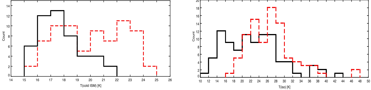
Figure 10. Left: Cold ISM temperature from the DCE08 fits for the lowest redshift bin which has 41 percent PACS detections. The sources with PACS detections are shown by the red dashed line while those without PACS detections but which do have a 350\mu\text{m} flux above 3\sigma in addition to the 5\sigma 250\mu\text{m} point are shown in black. Right: Same but for the isothermal temperature
