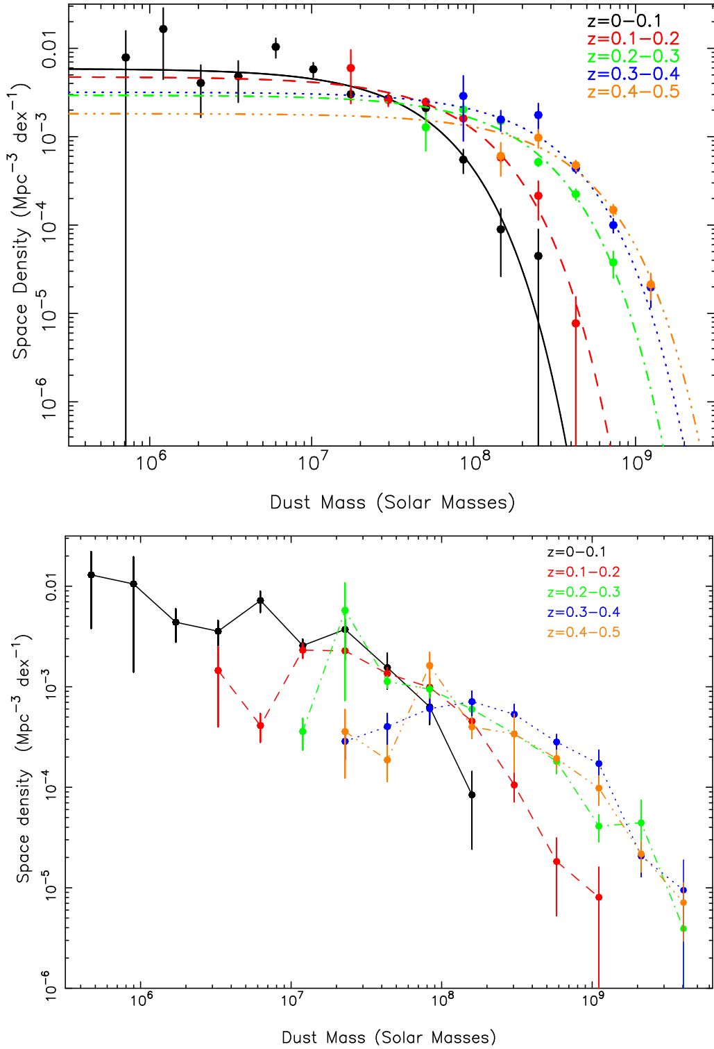
Figure 9. Dust mass functions using the modified PC00 estimator calculated in 5 redshift slices of \Delta z = 0.1 . Top SED based dust masses. Bottom Isothermal dust masses. The relation between dust mass and L_{250} has some scatter due to variation in the temperature of the cold ISM dust, which results in down-turns in the lowest mass bins in each redshift slice. The broader error on M_d acts to convolve the true DMF with a Gaussian of width approximately 0.2 dex. Schechter functions are plotted in the top panel with the faint-end slope fixed to that which fits best in the z < 0.1 slice. Parameters for the fits are given in Table 3.
