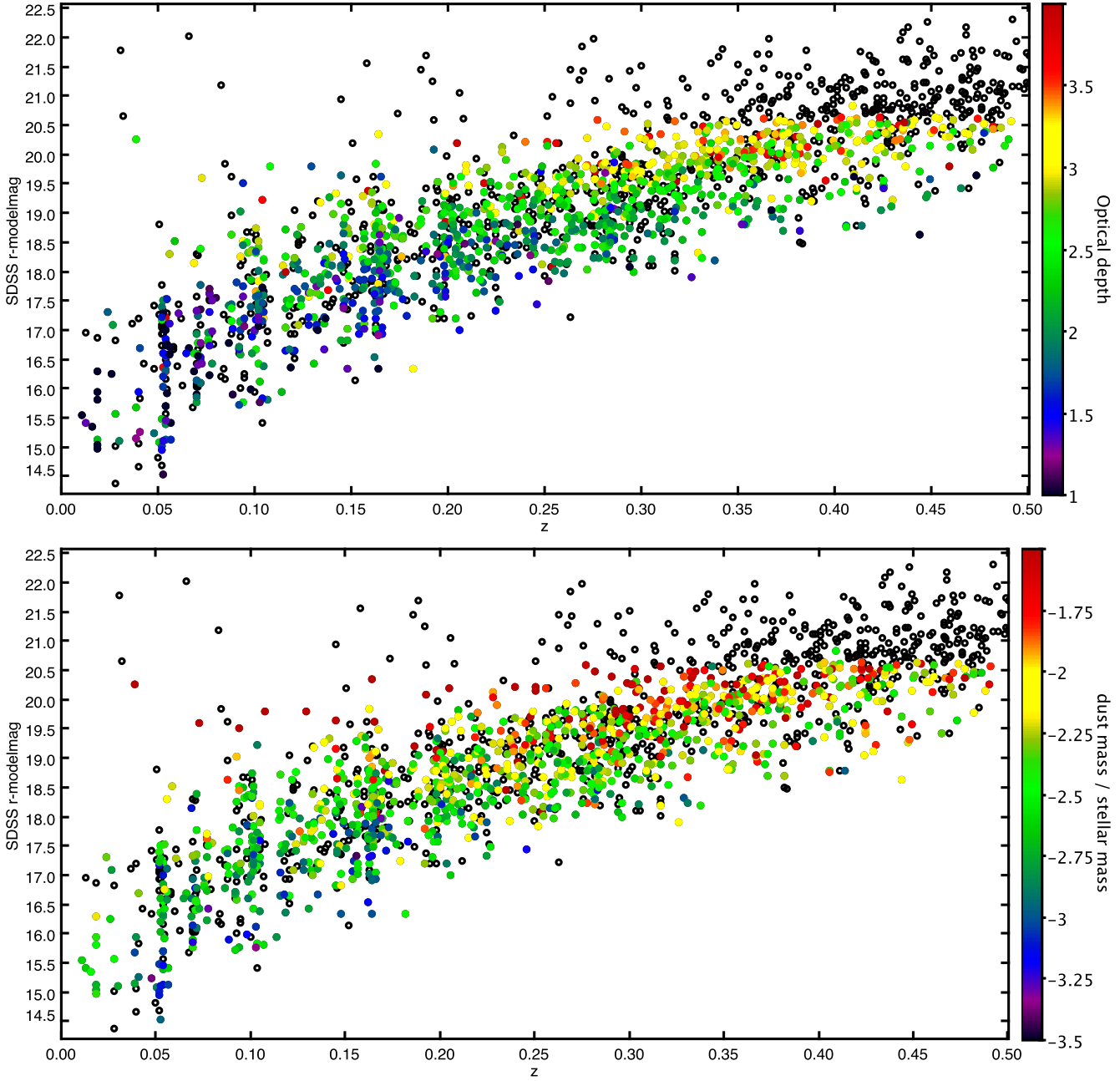
Figure 19. r -mag versus redshift for the H-ATLAS sources. Black open circles represent H-ATLAS sources which are too faint for an SED fit using the DCE08 model at the current time, or which were not in the region covered by GAMA photometric catalogues. Coloured points denote the values of either V-band optical depth ( top ) or dust-to-stellar mass ratio ( bottom ) from the DCE08 fits. The limit of reasonable completeness in the optical for the SED fits is z \sim 0.35 . Beyond this redshift, averaged values of optical depth or dust-to-stellar mass ratio will be biased low because only the brightest optical galaxies in that redshift bin will have SED fits (and these tend to have less obscuration).
