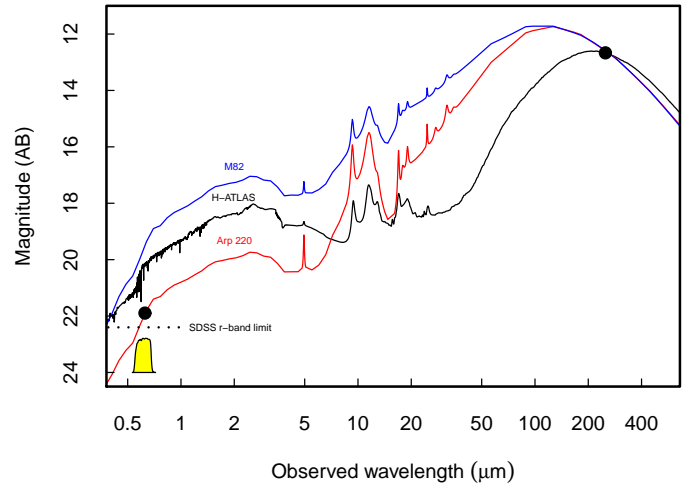
Figure 1. Templates for three galaxies showing the range of optical fluxes expected for galaxies which are at the SPIRE flux limit of S_{250} = 32 \text{ mJy} at z = 0.5 ; the limit of our study. The templates are for M82 (a typical starburst), a Herschel -ATLAS template derived from our survey data by Smith et al. in prep and Arp 220, a highly obscured local ULIRG. The SDSS limit of r = 22.4 is shown as a horizontal dotted line and even a galaxy as obscured as Arp 220 is still visible as an ID to our optical limit at z = 0.5 . The yellow shape represent the SDSS- r band filter which was used to compute the optical flux
