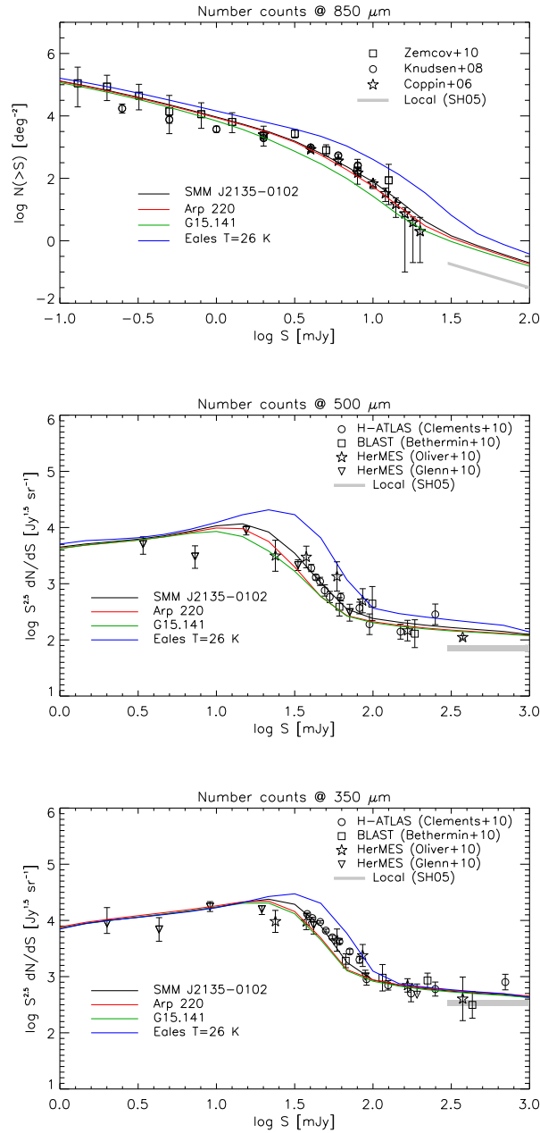
Figure 17. Constraints on the SED of high- z galaxies from multi-wavelength source counts. We have determined the luminosity functions at different redshifts > 1 using our reference sample and the SEDs of Arp220 and G15.141, in addition to SMM J2135-0102, and used them to compute the number counts at several wavelengths, adding the contributions of (lower- z ) spiral and starburst galaxies as given by the Negrello et al. (2007) model. In all cases we recover a good fit at 250 \mu\text{m} , essentially by construction since this is the main selection wavelength. At longer wavelengths, however, while the counts obtained using the SMM J2135-0102 SED are still nicely consistent with the data, the other SEDs do not yield good fits. The counts given by the luminosity functions estimated by Eales et al. (2010), K-corrected with their SED, are also shown for comparison. In this case too the observed 250 \mu\text{m} counts are accurately reproduced.
