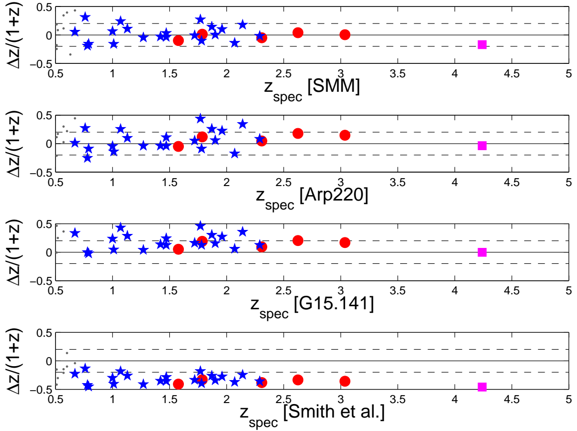
Figure 3. Photometric redshift estimates based on the SEDs of (from top to bottom) SMM J2135-0102, Arp220, G15.141, and the average low- z SED from Smith et al. (2011) compared in terms of the quantity \Delta z/(1+z) \equiv (z_{\text{phot}} - z_{\text{spec}})/(1+z_{\text{spec}}) with spectroscopic measurements for the strongly lensed galaxies of Negrello et al. (2010; red filled circles) and Cox et al. (2011; purple filled square), and for the H -ATLAS SDP galaxies with z > 0.5 of Bonfield et al. (2011; blue asterisks) and Smith et al. (2010; black dots). The dashed lines correspond to a 20% difference.
