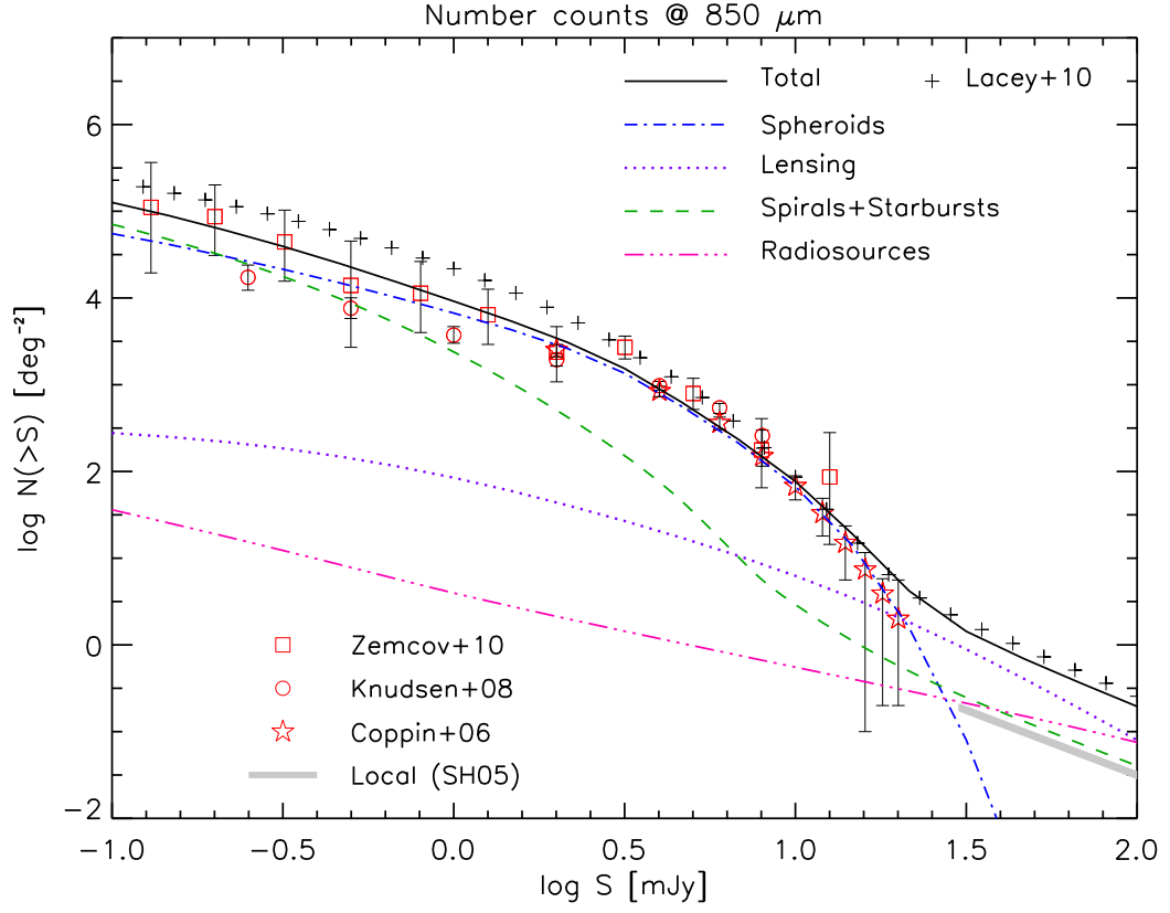
Figure 13. Comparison of the observed integral counts at 850\mu\text{m} (Zemcov et al. 2010; Knudsen et al. 2008; Coppin et al. 2006) with the predictions of our full model (solid line) and of the semi-analytic model of Lacey et al. (2010; crosses). The lines have the same meaning as in Fig. 10.
