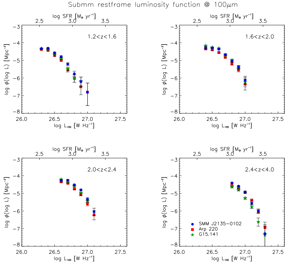
Figure 6. Comparison of the luminosity functions at 100\mu\text{m} computed using different SED templates – SMM J2135-0102 (blue circles), Arp220 (red squares), and G15.141 (green stars) – after correcting for the median offsets in the redshift estimates highlighted by Fig. 3. To ease the comparison, only statistical uncertainties are reported.
