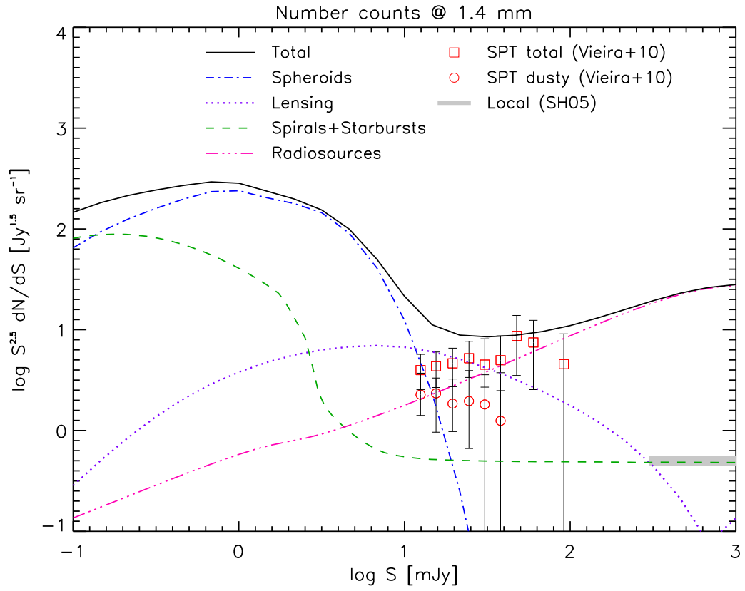
Figure 15. Comparison of the observed Euclidean normalized counts at 1.4 mm (Vieira et al. 2010) with the predictions of our full model (solid line). The lines have the same meaning as in Fig. 10.
