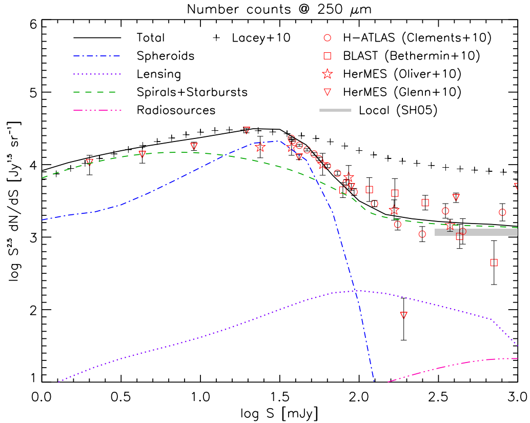
Figure 10. Comparison of the observed Euclidean normalized counts at 250 \mu\text{m} (Clements et al. 2010; Oliver et al. 2010; Glenn et al. 2010; Bethérmin et al. 2010) with the predictions of our full model (solid line) and of the semi-analytic model of Lacey et al. (2010; crosses). The different lines show the contributions to the counts of the various populations included in our full model: unlensed (blue dot-dashed line) and strongly lensed (purple dotted line) proto-spheroidal galaxies (host halo masses are within the range 2.5 \times 10^{11} M_{\odot} \lesssim M_H \lesssim 3 \times 10^{13} M_{\odot} ), normal late-type plus starburst galaxies (green dashed line), radio sources (magenta triple-dot-dashed line). The radio source counts are from the De Zotti et al. (2005) model. The grey shaded area shows the counts of local galaxies estimated by Serjeant & Harrison (2005; SH05).
