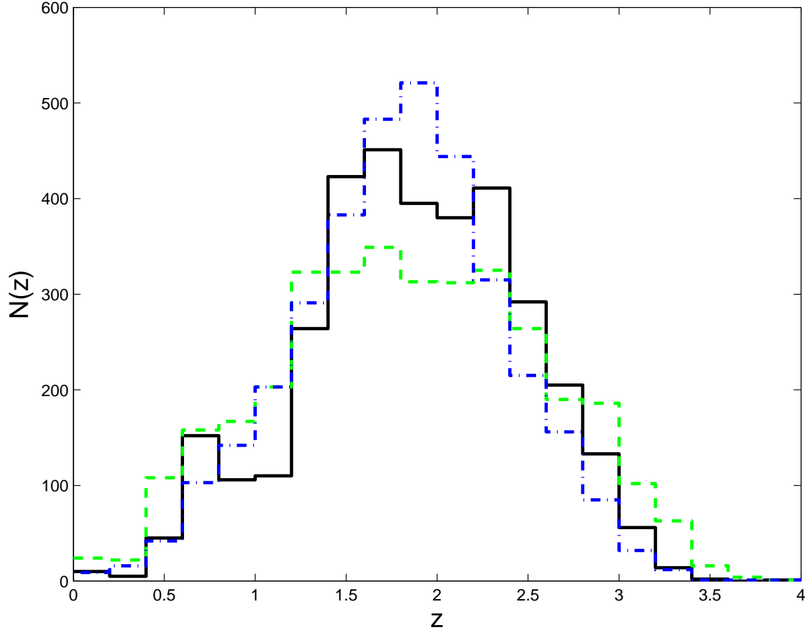
Figure 4. Comparison of the redshift distributions of sources in our reference sample ( S_{250\mu\text{m}} > 35 \text{ mJy} , S_{350\mu\text{m}} > 3\sigma , and no R > 0.8 optical identifications; 3469 sources, i.e. \approx 50\% of the 6876 H-ATLAS SDP galaxies; the selection has mostly excluded the z < 0.5 sources, and in fact there is another peak in the redshift distribution of the total SDP sample at z < 0.5 , see Smith et al. 2011a) estimated using the SEDs of Arp 220 (green dashed line), G15.141 (blue dot-dashed line), and of SMM J2135-0102 (black solid line), correcting for the offsets estimated from Fig. 3. For our preferred SED, the one of SMM J2135-0102, 3093 are estimated to be at z > 1 . Correcting for the contamination by cold low- z galaxies with genuine r < 22.4 counterparts not identified with R > 0.8 (see §5), we estimate that the fraction of SDP galaxies with S_{250\mu\text{m}} \geq 35 \text{ mJy} (6100 in total) that are at z > 1 is of \approx 45\% .
