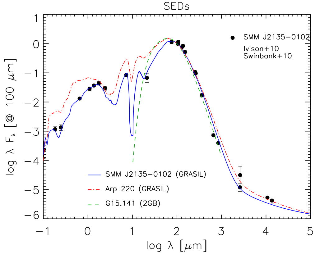
Figure 2. The SED of SMM J2135-0102 (“The Cosmic Eyelash”) as modeled by GRASIL (blue solid line); data are from Ivison et al. (2010) and Swinbank et al. (2010). The SED of Arp220 (red dot-dashed line) as modeled by GRASIL, and that of G15.141 modeled as a double-temperature grey-body (green dashed line; see text for details) are also shown for comparison. All SEDs are in the rest-frame and are normalized at 100 \mu\text{m} .
