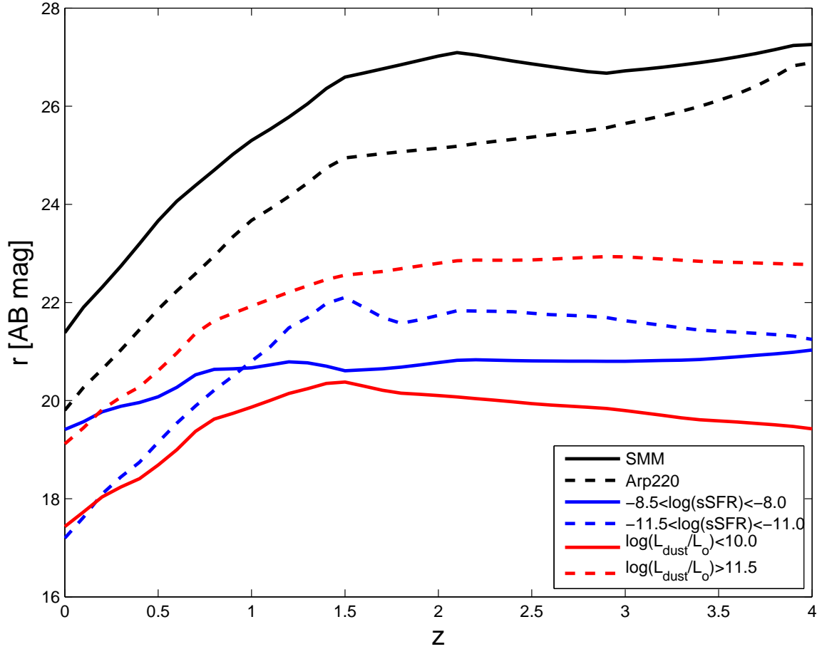
Figure 1. Optical (SDSS r -band) magnitudes as a function of redshift for several SEDs, normalized to S_{250\mu\text{m}} = 33.5 \text{ mJy} , the 5\sigma detection limit for H -ATLAS SDP galaxies. The red curves refer to the mean SEDs of optically identified z < 0.5 SDP galaxies in the lowest [ 9.5 < \log(L_{\text{dust}}/L_{\odot}) < 10 ; solid line] and in the highest [ 11.5 < \log(L_{\text{dust}}/L_{\odot}) < 12 ; dashed line] luminosity bins of Smith et al. (2011b). The blue curves refer to the same sample by Smith et al. (2011b) but for the lowest [ -11.5 < \log(\text{sSFR}) < -11 ; dashed] and for the highest [ -8.5 < \log(\text{sSFR}) < -8 ; solid] specific star formation rate (in \text{yr}^{-1} ) bins. The dashed black line refers to the SED of Arp220 (a local ULIRG) and the black solid line to that of SMM J2135-0102 (‘The Cosmic Eyelash’ at z \approx 2.3 ). As explained in § 2, the figure is meant to illustrate that the high- z H -ATLAS sources must have global SEDs different from the low- z ones. The latter are relatively cool and unobscured, while the high- z population is dominated by more obscured objects with higher star-formation rates and warmer dust temperatures.
