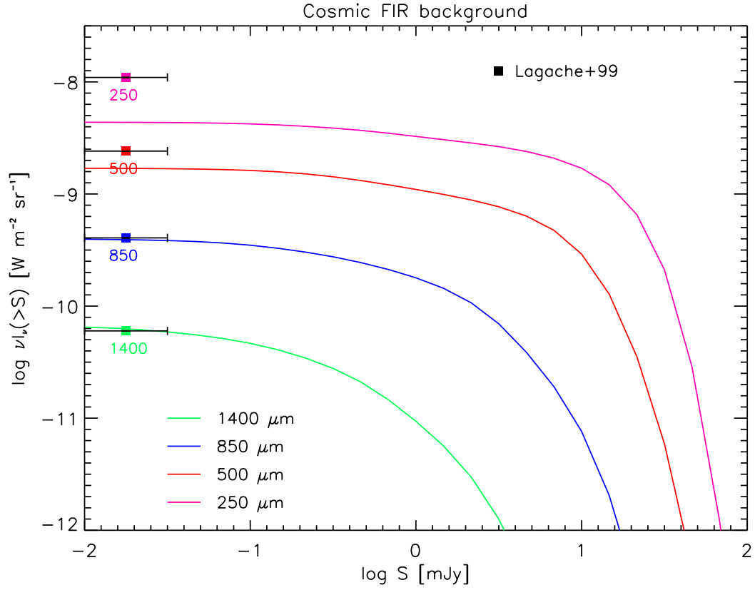
Figure 19. Contributions of high- z proto-spheroidal galaxies to the (sub-)mm extragalactic background, according to our model, compared with the observational estimates of the total background intensity (Lagache et al. 1999). ETGs account almost entirely for the background at \lambda \gtrsim 850 \mu\text{m} . Contributions from lower redshift ( z \lesssim 1 - 1.5 ) late type, normal and starburst galaxies become increasingly important at shorter wavelengths.
