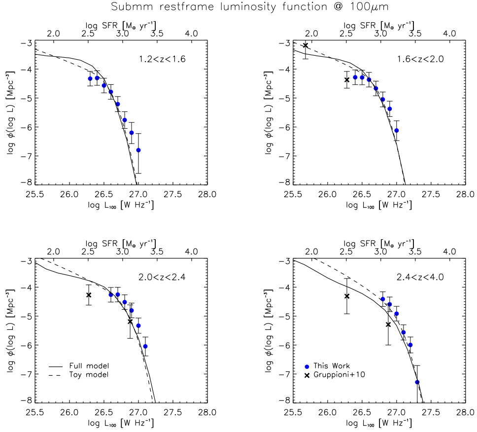
Figure 5. Luminosity functions at 100\mu\text{m} in four redshift intervals compared with models described in the text (solid line: full model; dashed line: toy model). The flattening of the LFs at the lowest luminosities may be, at least in part, due to the overestimate of the accessible volume yielded by the 1/V_{\text{max}} estimator for objects near to the flux limit (Page & Carrera 2000). The 90\mu\text{m} LFs (crosses) estimated by Gruppioni et al. (2010) using PACS data are also shown for comparison.
