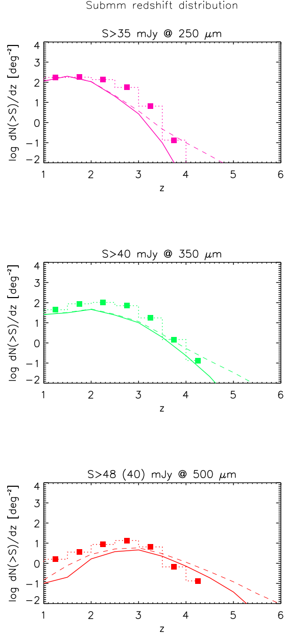
Figure 18. Comparison between the estimated redshift distributions (histograms) of proto-spheroidal galaxies at 250\mu\text{m} ( S_{250\mu\text{m}} \geq 35 \text{ mJy} ), 350\mu\text{m} ( S_{350\mu\text{m}} \geq 40 \text{ mJy} ), and 500\mu\text{m} ( S_{500\mu\text{m}} \geq 48 \text{ mJy} ), and the predictions of our full model, using the same parameters as in Lapi et al. (2006); solid lines refer to unlensed, while dashed lines also include the contribution of lensed, proto-spheroids. Because of the flux boosting due to confusion, the catalogued 500\mu\text{m} flux densities have to be scaled down by the factors given by Clements et al. (2010). For example, the 500\mu\text{m} flux density limit of 48 \text{ mJy} for catalogued sources corresponds to a boosting corrected flux limit of 40 \text{ mJy} . As discussed in the text (see also the caption to Fig. 4), we estimate that \approx 55\% of SDP galaxies with S_{250\mu\text{m}} > 35 \text{ mJy} are at z < 1 . Such galaxies belong to a different population comprising late-type normal and starburst galaxies.
