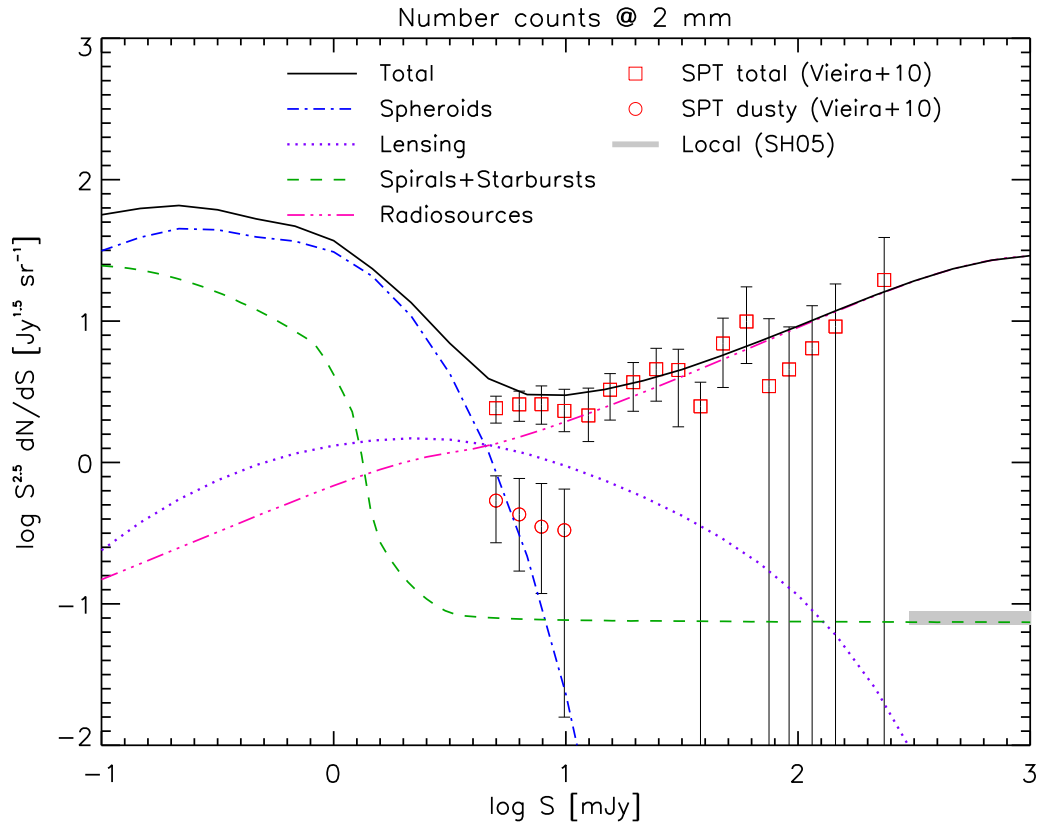
Figure 16. Comparison of the observed Euclidean normalized counts at 2 mm (Vieira et al. 2010) with the predictions of our full model (solid line). The lines have the same meaning as in Fig. 10.
