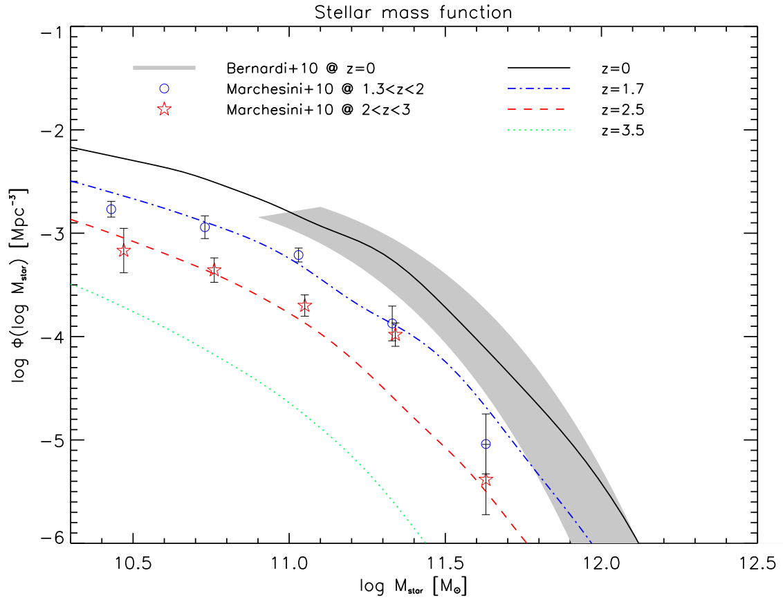
Figure 9. Stellar mass functions of ETGs at different redshift predicted by the toy model compared with observational determinations.
