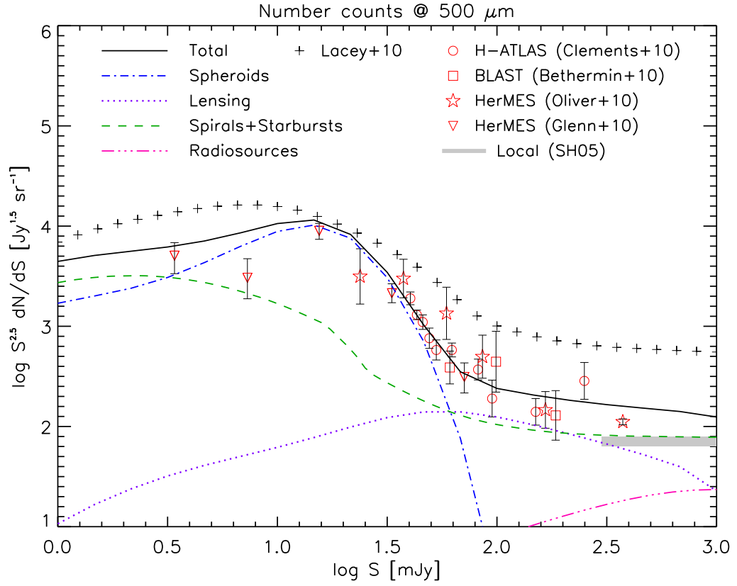
Figure 12. Same as in Fig. 10 but at 500 \mu\text{m} . Note that the flux densities in the Table 1 of Clements et al. (2010) must be multiplied by the correction factors given in the same table to produce the correct flux densities; the lowest corrected 500 micron flux density is 40 mJy.
