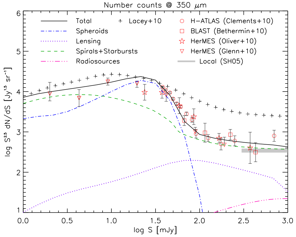
Figure 11. Same as in Fig. 10 but at 350 \mu\text{m} .
