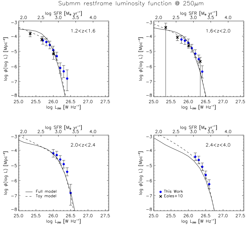
Figure 7. Luminosity functions at 250\mu\text{m} in four redshift intervals based on our reference sample, compared with the predictions of the models discussed in the text (solid line: full model; dashed line: toy model) and with the estimates by Eales et al. (2010b), after applying the K -corrections based on the SMM J2135-0102 SED, for common redshift ranges.
