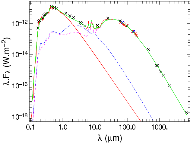
Fig. 2. Best fit with MCFOST to the observed data. Shown is the photometry obtained from the literature (black), Spitzer IRS spectrum (red), PACS photometric observations (blue crosses), and PACS continua derived from the spectroscopic observations (red crosses). The green line represents the best MCFOST model, in red the atmosphere model. The blue dot-dashed and pink dashed lines are the contributions (scattered light and thermal emission) from the inner and outer disc, respectively.
