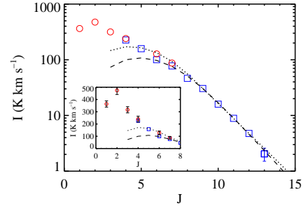
Fig. 4. Comparing the highest likelihood model (dotted line) with our CO line intensities. The model shown by a dashed line was obtained by using only J \geq 7-6 CO lines. The W03 data are shown by open circles. The inset highlights the deviations from models at the lower J end.
