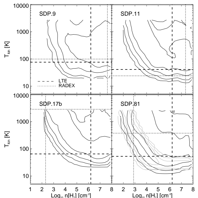
Figure 11. Contour plots of the (T_{kin}, n[\text{H}_2]) 2D marginal likelihood distributions, generated by a MCMC sampling of the parameter space for RADEX models. The contours are in n\sigma -equivalent steps, enclosing 68.3%, 95.4%, 99.7%, and 99.99% of the probability, respectively. The dashed lines correspond to parameters that reproduce the LTE solution, and the dotted lines indicate the parameters corresponding to the RADEX 4D maximum likelihood solution. Note that the 2D marginal distributions will not necessarily have the same maximum as the 4D distribution. The kinetic temperature is limited to < 3000 \text{ K} , where collisional dissociation of CO becomes important. In the SDP.81 panel, the lighter contours show the probability levels for a model including the CO(1–0) from Frayer et al. (2011). The parameters for this model are listed as model SDP.81* in Table 5.
