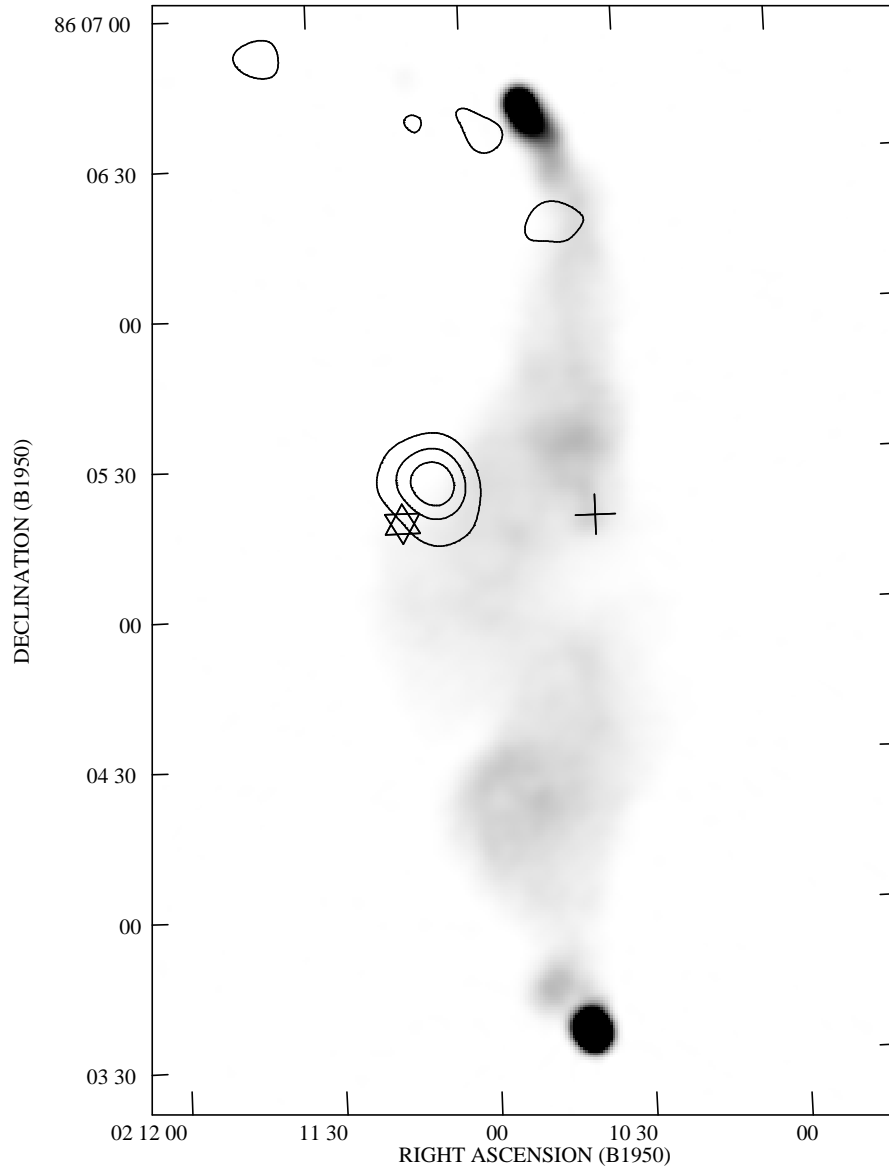
Figure 1. 3C 61.1 in radio and X-ray. The greyscale is a 1.5-GHz radio map (Leahy & Perley 1991) taken from Leahy, Bridle & Strom (1998); the resolution is 3.7 arcseconds and black represents 100 \text{ mJy beam}^{-1} . Contours show the X-ray image smoothed with a \sigma = 4 arcsec Gaussian, and are at (6.1 \times 10^{-3}) \times (1, 2, 4 \dots) HRI counts \text{arcsec}^{-2} . The lowest contour corresponds to the 3\sigma level, calculated as described by Hardcastle et al. (1998c). The cross corresponds to the position of the 2.7-GHz radio core (Laing & Riley, in prep.) and the star to the position on DSS plates of the background object discussed in the text. The offset between the X-ray position and the position of the radio core is too large to be introduced by ROSAT pointing inaccuracies.
