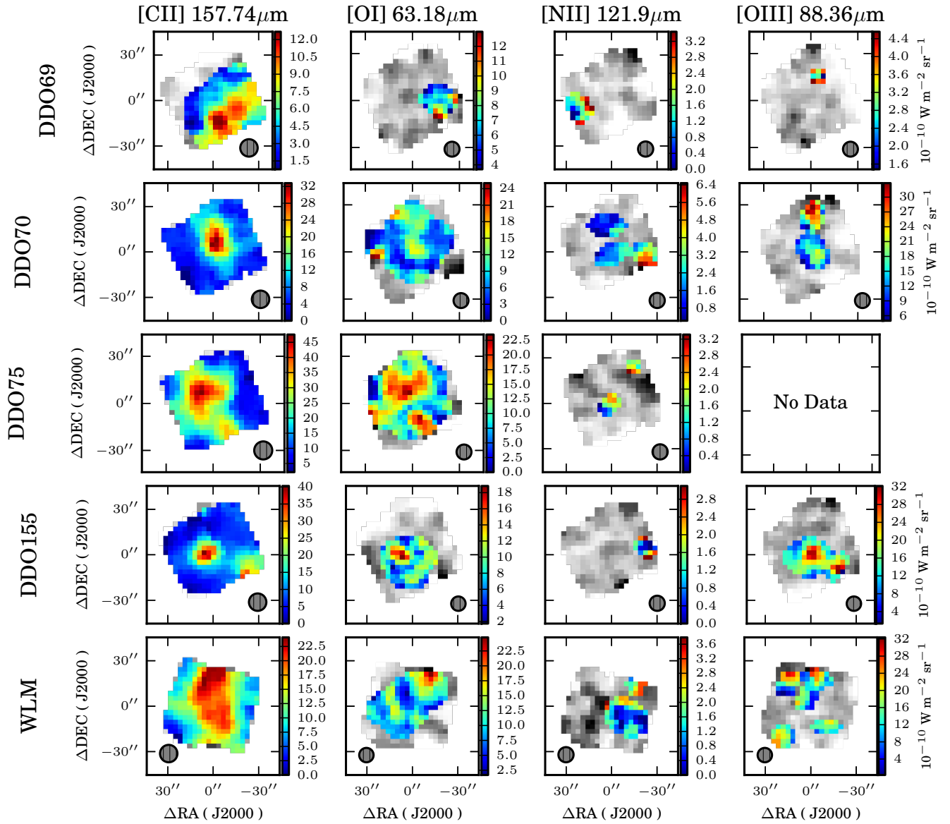
FIG. 7.— PACSman brightness maps of the four observed lines in each of our five galaxies. Fluxes in the regions that registered detections ( S/N > 3 ) are shown in color, while fluxes from areas of non-detections are shown in grayscale. The flux (color) scale is different for each map. The mask regions are the same as those detailed in Figure 5 and § 3.3: for [C II] and [O I], S/N values are determined from the moving integration kernel maps, while S/N regions for [O III] and [N II] were determined by manual inspection of the spectral data cubes. The hatched circle at the bottom of each map shows the PACS beam size of the given line.
