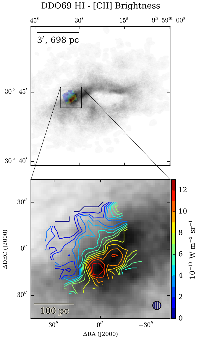
FIG. 1.— Overlay of Herschel [C II] contours onto HI in DDO 69. Darker gray corresponds to increased HI emission. The [C II] beam is shown in the lower frame. Overlays of the other galaxies can be found in Figure 2.
