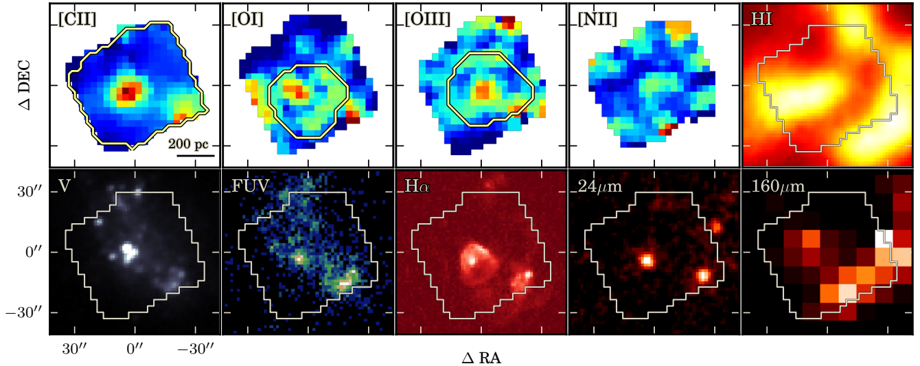
FIG. 10.— Spatial comparison of emission in the Herschel PACSman maps with other observations at several wavelengths. DDO 155 appears here, with the other galaxies presented in Figures 11 and 12. Each image scaling is independent, to enhance dynamic range and draw out faint features. Brightness (yellow) in the H I colormap now corresponds to higher column density (as opposed to darkness in the grayscale of Figures 1 and 2). The Herschel maps have overlaid contours showing regions where S/N > 3 for the flux contained within regions spanning a minimum of 2 beam widths, as described in § 3.3. Since our signal is typically weak (except for [C II]), and since we are interested in detections aggregated from regions the size of one beam or larger, we do not look at S/N values of single re-gridded pixels. In the other maps, the white outlines indicate the footprint of the [C II] map. Here, H I is from Hunter et al. (2012), V-band from HE06, FUV from Dale et al. (2009), H\alpha from HE04, 24\mu\text{m} & 160\mu\text{m} from Dale et al. (2009).
