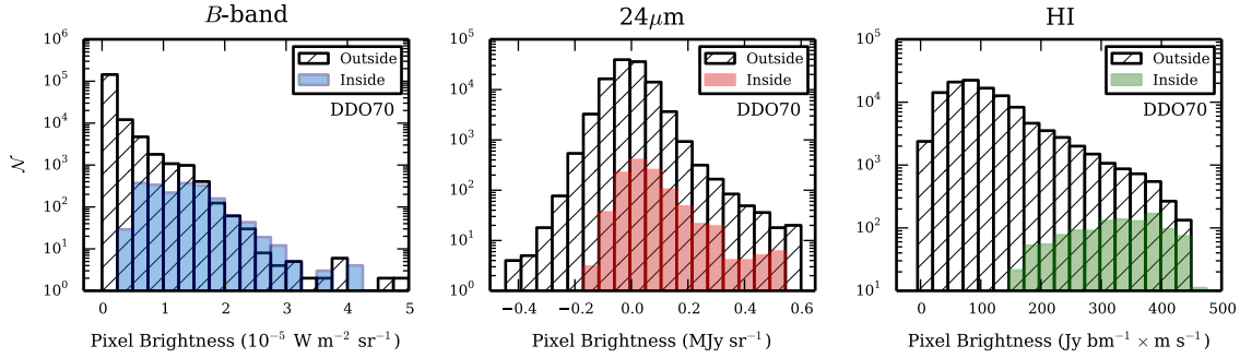
FIG. 3.— Pixel brightness histograms for the B -band, 24\mu\text{m} , and H I maps of DDO 70. The values inside the observed Herschel footprint are shown in color, while those outside of the footprint are shown in black and white. The “inside” distributions of the B -band and 24\mu\text{m} maps are representative of the majority of the “outside” distributions. H I is quite extended in our galaxies, with low column densities at the outer edges (c.f. Figures 1 & 2). Even though the H I distributions are not equivalent, we sample the brighter non-edge emission in the galaxy fairly well. The histograms for the other four galaxies in our sample show similar behavior to those presented here for DDO 70.
