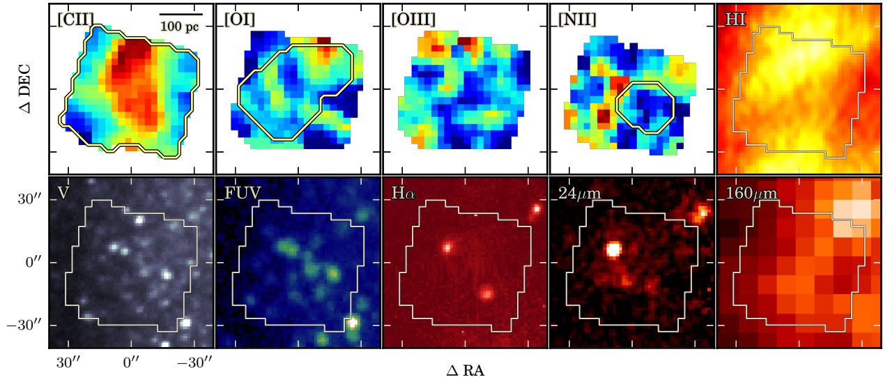
FIG. 12.— Comparison of emission in the Herschel maps with other observations at several wavelengths. H I is from Hunter et al. (2012), V-band from HE06, FUV from Hunter et al. (2010), H \alpha from HE04, 24 \mu m & 160 \mu m from Dale et al. (2009). We note that, in general, [C II] emission correlates well with H I emission, and bright knots in the bands that trace star formation are often near [C II] peaks.
