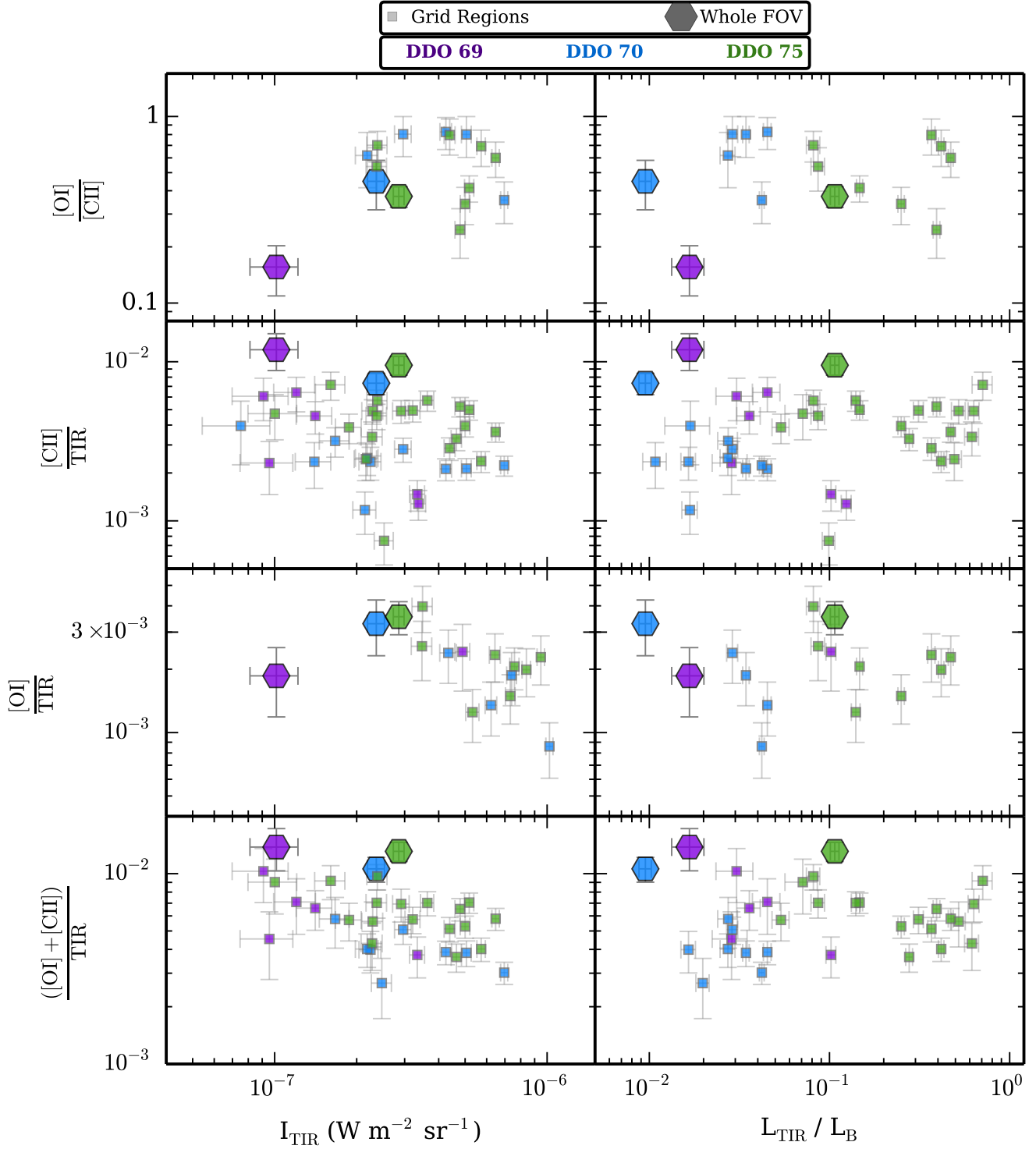
FIG. 15.— Herschel line ratio comparison for resolved regions and beam-by-beam grids as described in § 5.3. Each resolved data point (square symbols) represents the fluxes contained within a single [C II] beam width. Only detections ( 3\sigma ) are shown. We only consider TIR derived from PACS 100\mu\text{m} maps (DDO 69, DDO 70, DDO 75; squares) for trends on these scales, since these regions are much smaller than the limiting MIPS 160\mu\text{m} beam size for the Spitzer -based TIR. The global line ratios for TIR calculated from PACS (hexagons) are plotted for reference.
