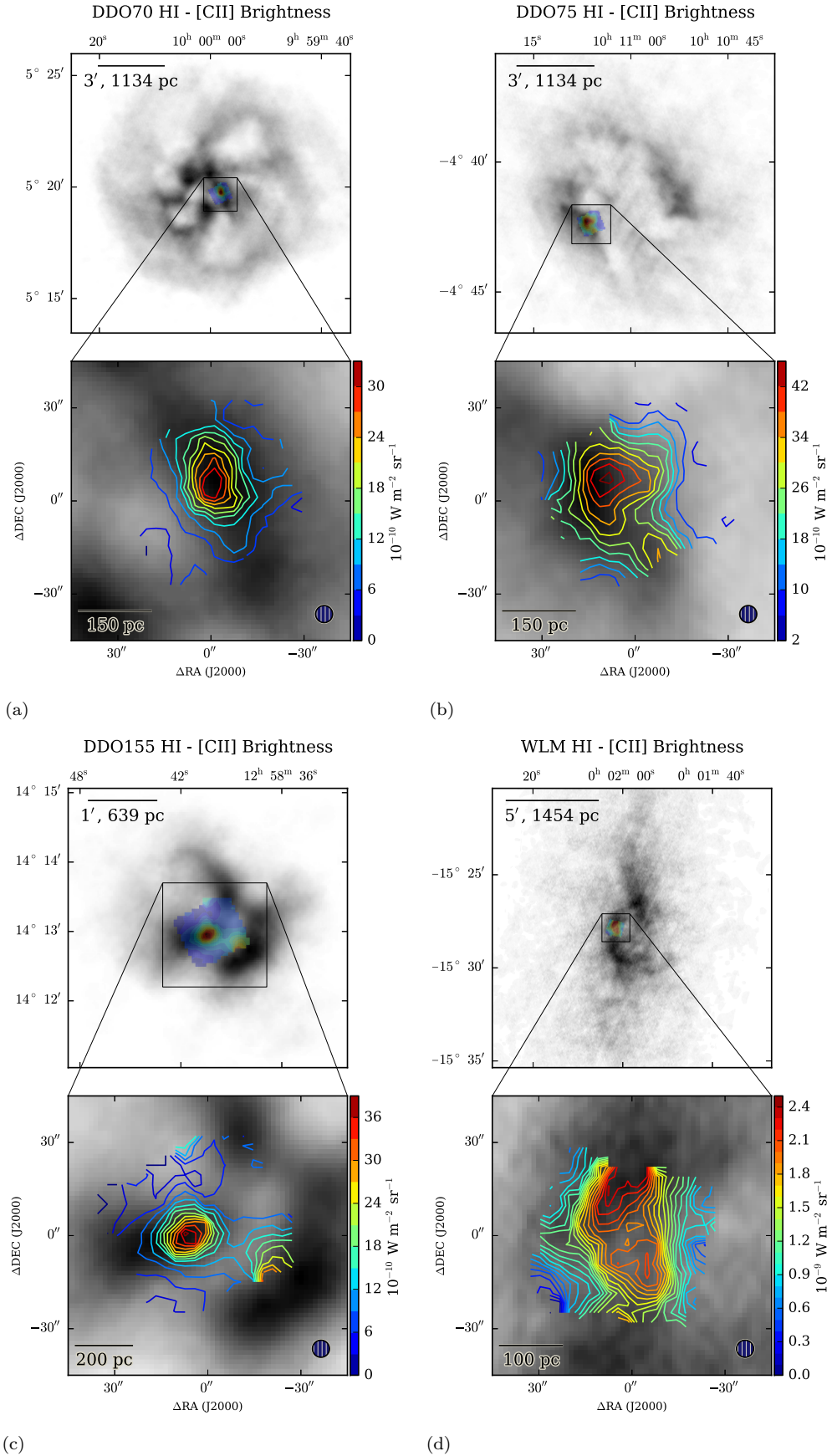
FIG. 2.— Overlays of Herschel [C II] contours onto H I maps from Hunter et al. (2012). Each PACS footprint covers 51'' \times 51'' on a side. Darkness in the grayscale corresponds to increased H I emission. The contour levels and linear scales are different for each target.
