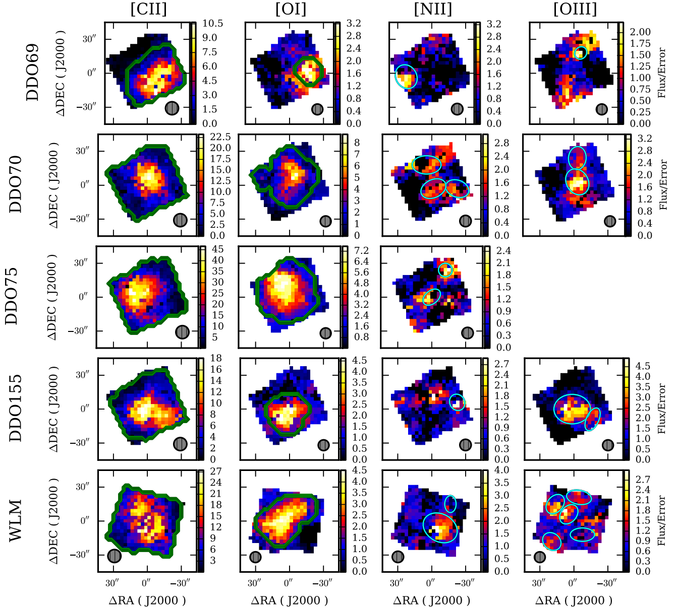
FIG. 5.— Maps of signal to noise (fitted flux over fitted error) for our galaxies, with regions indicated for combining spectra. Colorscale values indicate the significance ( \sigma ) level of the fits for spectra summed from a region centered on that pixel, with a diameter of two beam widths. The green contours, used for the broadly detected [C II] and [O I] emission, outline the contiguous region in each map where S/N > 3 (based on the 2-beam-width integration kernel). The cyan ellipses in the [O III] and [N II] maps are the regions used for spectrum aggregation, based on signal found by manual inspection of the 3D spectral cubes: apertures of varying sizes and shapes that contain S/N \sim 3 profiles, based on the brightest regions in the moving-integration maps. Note that the cyan ellipses do not exactly follow S/N peaks - that is, some regions of manually-identified signal do not overlap exactly with the bright spots from the integrated flux maps. This is especially true for [N II], where the emission is particularly faint.
