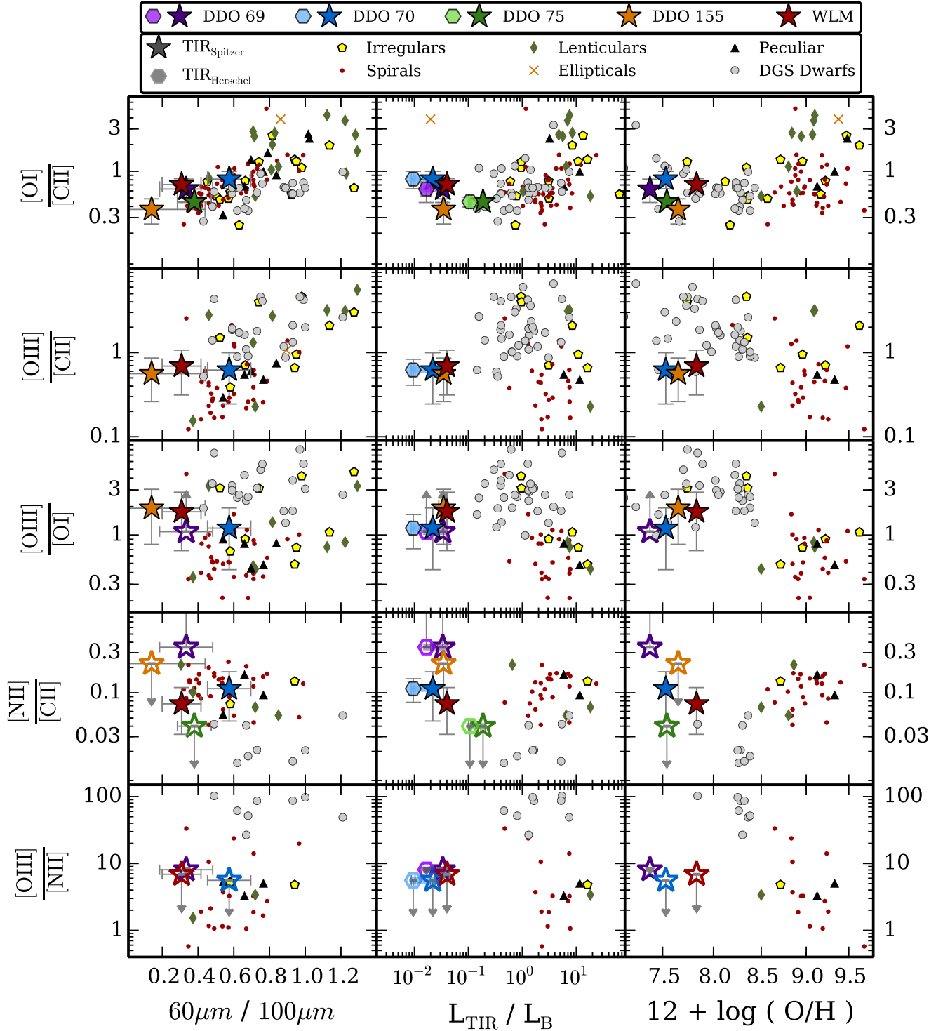
FIG. 8.— Herschel far infrared line ratios. Line fluxes were integrated over the regions shown in Figure 5. The fluxes for each ratio were integrated over identical apertures, according to the selection order: [N II], [O III], [O I]. IRAS data for additional LITTLE THINGS galaxies come from Hunter et al. (1989) and ISO data from Hunter et al. (2001). Spiral, elliptical, and irregular † galaxy data points from Brauher et al. (2008) are given for comparison with the 60\mu\text{m}/100\mu\text{m} ratios, TIR/B ratios, and metallicities, complemented by dwarfs from the DGS sample (Cormier et al. 2015). We only plot detections for the comparison sample data, omitting upper limits from B+08. TIR for that sample are computed from the 25, 60, and 100\mu\text{m} flux densities: \text{TIR}_{\text{IRAS}} = 2.403(\nu f_{\nu})_{25} - 0.245(\nu f_{\nu})_{60} + 1.638(\nu f_{\nu})_{100} . Metallicities for the reference sample were determined from the Luminosity-Metallicity relation described by Lamareille et al. (2004). For our measurements, detections are denoted by solid filled stars. TIR derived from Herschel photometry is also shown by the hexagon symbols for galaxies with PACS 100\mu\text{m} data: DDO 69, DDO 70, and DDO 75. Upper and lower limits ( 3\sigma ) for our data appear as empty symbols with arrows.
