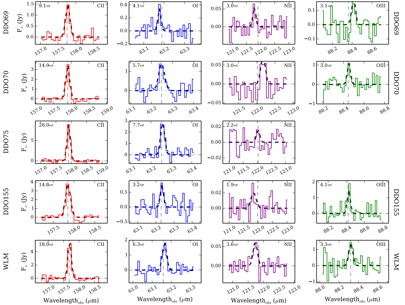
FIG. 6.— Spectra from the regions described in Figure 5 are combined to give a global measure of all observed flux. The vertical dashed grey line indicates the expected line center location, based on the local H I velocity of each galaxy.
