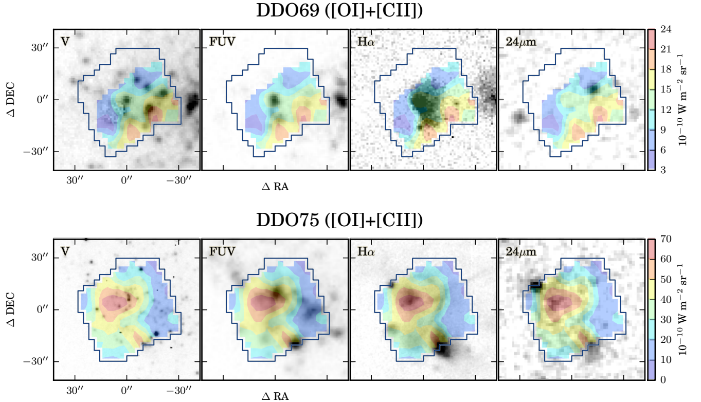
FIG. 14.— ([O I] + [C II]) intensity overlaid onto V, FUV, H\alpha , and 24\mu\text{m} maps in grayscale (dark = brighter emission) for DDO 69 and DDO 75. The filled Herschel contours are the same across each row. In DDO 69, the ([O I] + [C II]) emission is concentrated at the edge of the H\alpha region - a nice example of a PDR. Agreement is good for H\alpha in DDO 75, but slight offsets are apparent for FUV.
