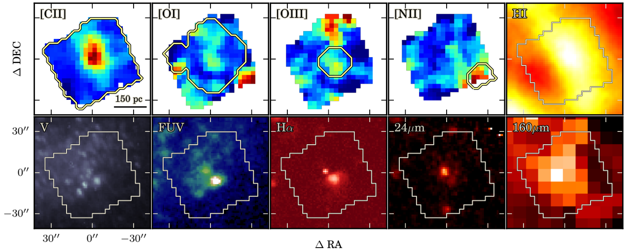
FIG. 11.— Comparison of emission in the Herschel PACSman maps with other observations at several wavelengths. H I is from Hunter et al. (2012), V-band from HE06, FUV from Hunter et al. (2010), H \alpha from HE04, 24 \mu m & 160 \mu m from Dale et al. (2009). We note that, in general, [C II] emission correlates well with H I emission, and bright knots in the bands that trace star formation are often near [C II] peaks.
