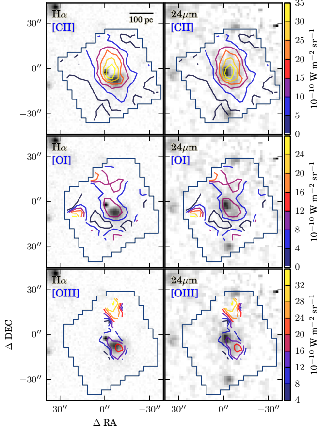
FIG. 13.— [C II], [O I], and [O III] intensity maps overlaid onto H\alpha and 24\mu\text{m} grayscales (dark = brighter emission) for DDO 70. The Herschel contours are the same in each row. In this galaxy, the [C II] emission is offset from the H\alpha peaks, while the [O III] emission is more closely aligned to H\alpha . It is interesting to note that the H\alpha and 24\mu\text{m} peaks are slightly offset.
