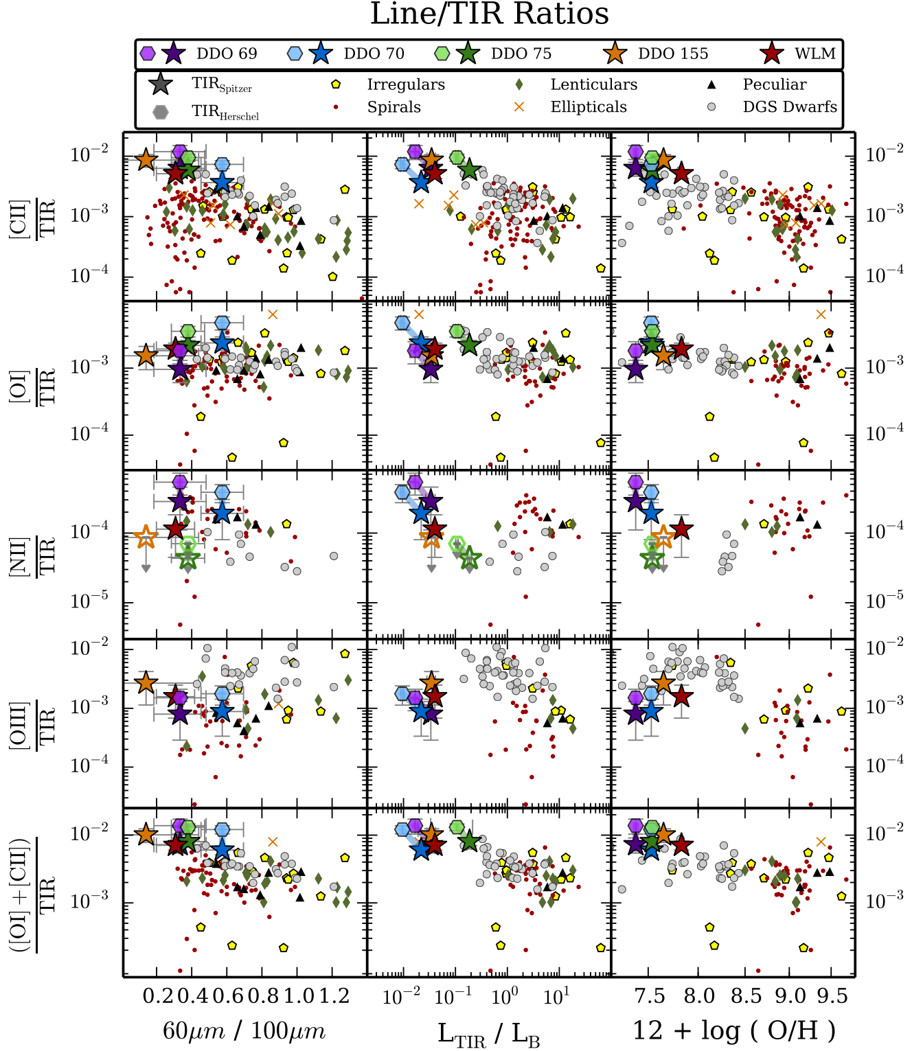
FIG. 9.— PACS and Spitzer TIR line ratios. Line fluxes were integrated over the regions shown in Figure 5: the majority of the footprints for [C II] and [O I], and smaller manually-identified regions for [O III] and [N II]. The [N II] and [O III] error bars each have an additional 50% uncertainty added in quadrature, to account for potential biases from the aperture selection. The reference sample dwarf, spiral, elliptical, and irregular galaxy markers are the same as those described in Figure 8. Again, we only plot those data points from Brauhar et al. (2008) with published detections, and TIR for that sample is calculated from 25, 60, and 100 \mu\text{m} data. Our detections, using TIR calculated from Spitzer maps, are represented by solid stars. The hexagons represent TIR determined from PACS 100 \mu\text{m} , where available, and colored lines linking to the Spitzer points (stars) emphasize the differences. Upper limits ( 3\sigma ) appear as empty symbols.
