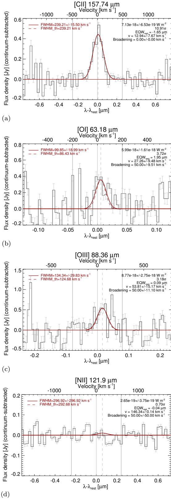
FIG. 4.— Sample continuum-subtracted spectra from single rasters of the central spaxel in the PACSman fit procedure for DDO 155. We detect [C II], [O I], and some [O III] emission, but there is no cospatial [N II] signal in this particular region. Line fit values are noted within each plot. The line center velocity is denoted as v . \text{FWHM}_{\text{th}} is the spectral resolution line width, due to the thermal properties of the instrument. Broadening is the excess line width beyond \text{FWHM}_{\text{th}} in the fit, when added in quadrature. That is, \text{FWHM}^2 = \text{FWHM}_{\text{th}}^2 + \text{Broadening}^2 . This broadening is not likely physical. \text{EQW}_{\text{rest}} is the width in wavelength units for which a box defined from zero flux to the continuum level, and centered at the rest wavelength, has an area equal to that of the integrated flux.
