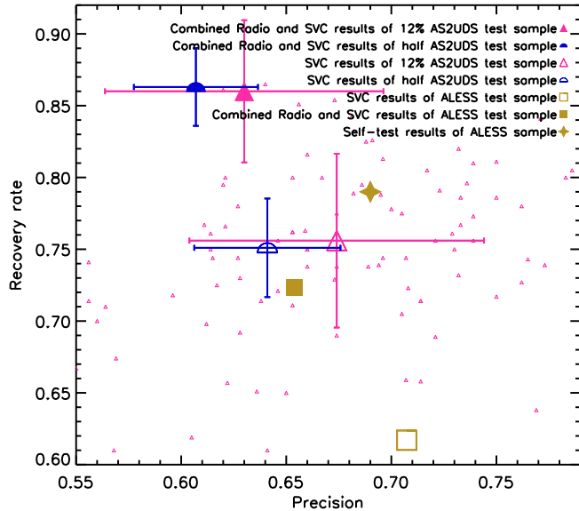
Figure 6. The results of applying the support vector machine-learning method to the independent samples from the AS2UDS and ALESS surveys. The blue open half circle shows the media precision ( 64 \pm 3 percent) and recovery rate ( 75 \pm 3 percent) of our machine-learning method for the “half-half” test – this involves constructing a training set from the galaxies in half of the ALMA maps in AS2UDS and testing the method on an independent sample from the other half of the ALMA maps. The filled half circle shows the results of the combined radio and machine-learning method for the “half-half” test. We show error bars estimated from the variation in the derived precision and recovery rate based on 100 bootstrap simulated “half-half” tests. We also apply our combined radio and machine-learning method, trained on the AS2UDS sample, to the independent ALESS sample in the ECDFS field and plot this as a filled square. We recover 72 percent of ALESS SMGs with a precision of 65 percent, which can be compared to the success rate indicated by a “self-test” on the ALESS sample (filled star). To investigate the variation in recovery rate and precision as a function of sample size, we also randomly select sub-samples of 88 AS2UDS ALMA maps (12 percent of AS2UDS sample) matching the number of ALMA maps in ALESS. We show the results of recovery rate ( 86 \pm 5 percent) and precision ( 63 \pm 7 percent) of the combined radio and machine-learning method for this “12 percent” test sample by filled triangle, and for just the machine-learning as a large open triangle. The small open triangles represent the results of machine-learning method for 100 individual sub-tests. Four of these “12 percent” tests have a recovery rate as low as that seen for the ALESS test sample, while the median recovery rate of these 100 tests is same to the “self-test” of AS2UDS. These results illustrate the success rate of our combined radio and machine-learning method and the expected scatter in the recovery and precision when applied to smaller samples, including those selected from different fields from those used for the training set.
