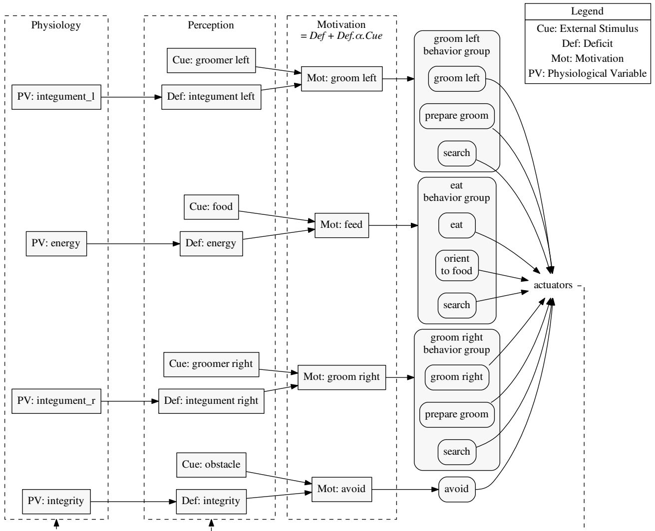
Figure 2. An overview of the action selection mechanism for our robot. Rounded boxes represent individual (potentially nested) behaviors, while square-cornered boxes represent other internal components. The actions of the actuators result in changes in the environment and the robot’s physiology, which is fed back to the robot’s perceptions. Motivations are updated and new behaviors selected every action selection loop (10Hz).
