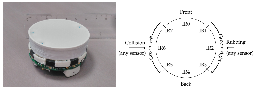
Figure 3. Left: An Elisa-3 robot, viewed from the front/left. Right: A diagram of the Elisa-3's infrared distance sensors (top view). Arrows indicate how the sensors are used to detect grooming and damage from collisions and sustained rubbing.
