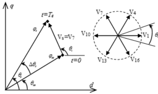
Figure 3. Flux deviation in a DTC control scheme
