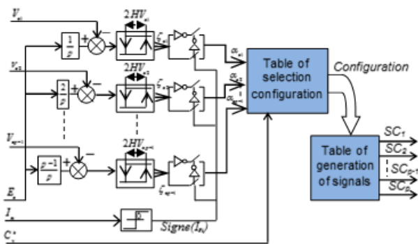
Figure 8. Selection of the hysteresis balancing procedure for phase capacitor voltages
