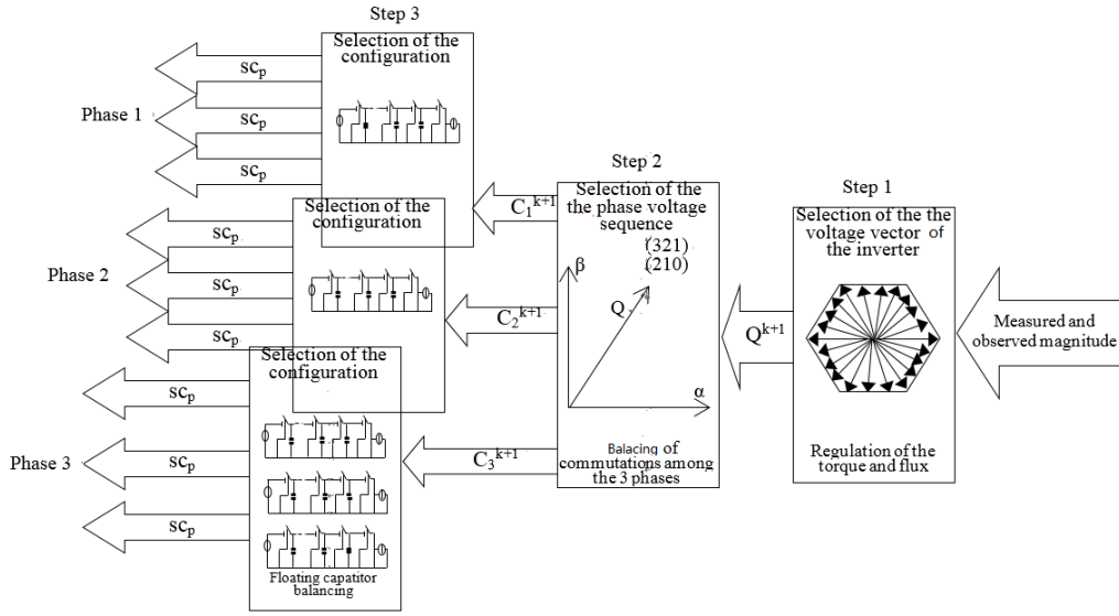
Figure 5. The three steps principle of ISFDTC applied to the torque of the asynchronous machine fed by a multilevel inverter
