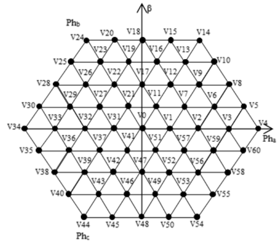
Figure 2. Voltages that can be supplied by the inverter with five voltage levels
