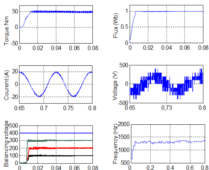
Figure 10. Response of ISFDTC torque, flux, stator current, voltage, evolution of voltages at floating capacitor terminals, and average switching frequency per cell
