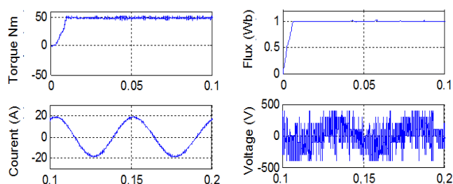
Figure 9. Response of conventional DTC: torque, flux, stator current, voltage
