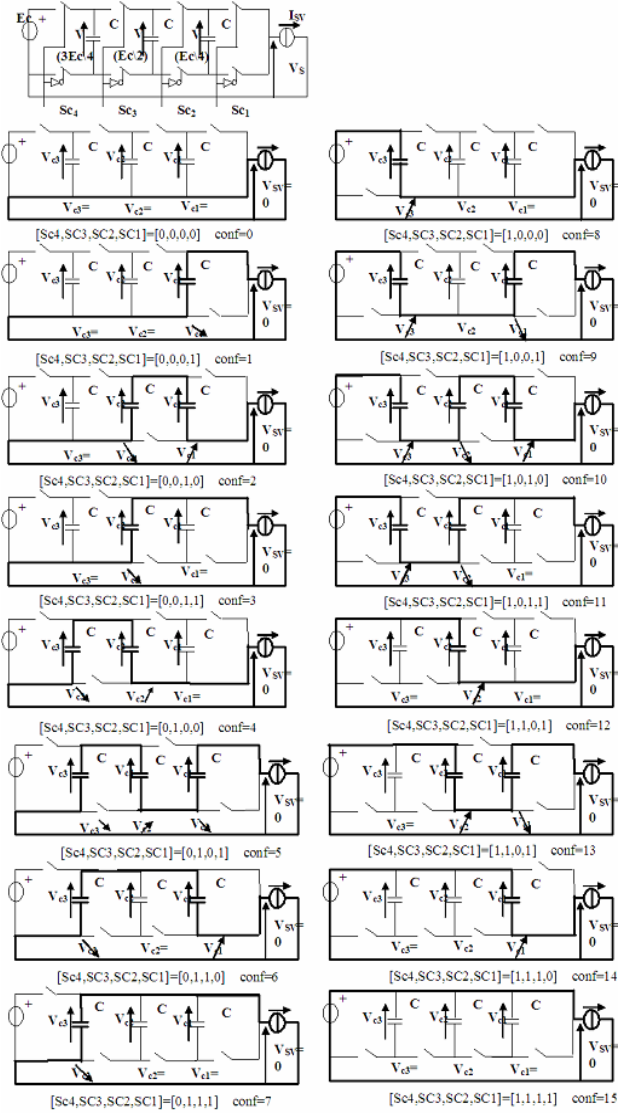
Figure 7. Possible configuration of a flying capacitors inverter arm with N = 4 , p = 3
