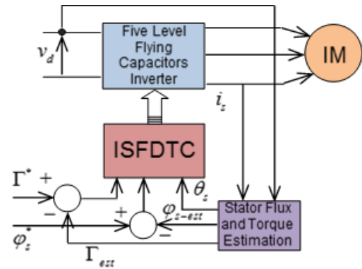
Figure 4. Block diagram of ISFDTC.
