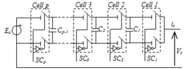
Figure 1. Flying capacitors inverter arm with N-levels (p = N-1 cell)
