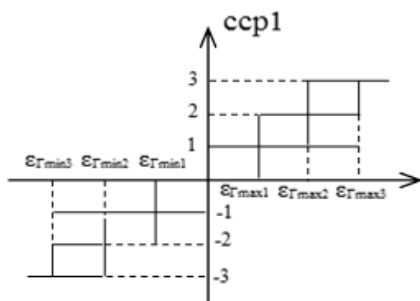
Figure 6. Hysteresis control regions of the torque.
