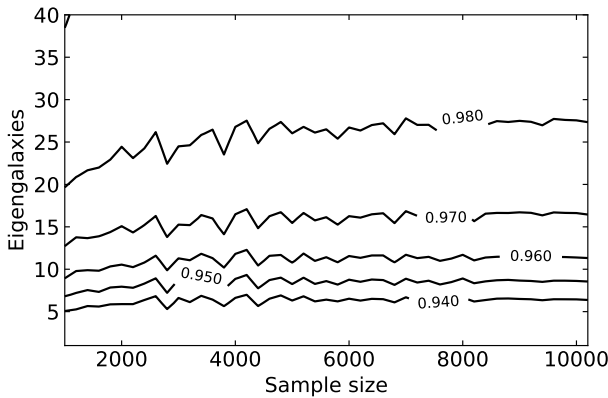
Figure 6. Contour plot of explained variance corresponding to the required number of eigengalaxies versus sample size. Higher explained variances tend to require proportionally more eigengalaxies as sample size increases, however at 12 eigengalaxies explained variance is asymptotic to a constant.
