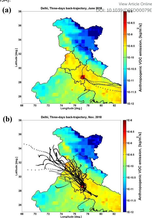
Figure 1. Three-day air mass back-trajectory for Delhi, for the selected days in June (a) and November (b). The back-trajectories for 00:00 and 12:00 UTC on each day are calculated based on the high-resolution meteorology field from WRF model. The background colors indicate the anthropogenic VOC emissions from EDGAR-HTAP 2010 dataset ( https://edgar.jrc.ec.europa.eu/ ). The data of the boundaries of administrative areas are sourced from https://gadm.org/ .
