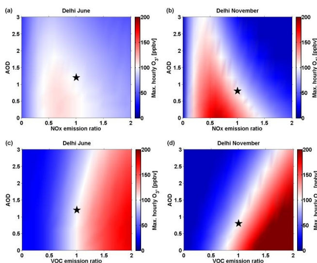
Figure 4. The impact of AOD on the non-linear VOC-NO x -ozone relationship in Delhi. (a) Impact on relationship between NO x and ozone in summer (June), (b) between NO x and ozone in winter (November), (c) between VOC and ozone in summer, and (d) between VOC and ozone in winter. Current conditions are marked by a black star.
