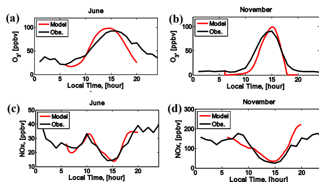
Figure 2. Observed and simulated ozone and NO x diurnal variations. (a) Ozone in June; (b) ozone in November, (c) NO x in June, and (d) NO x in November. The black line indicates observations and the red line indicates NCAR-MM model results.
