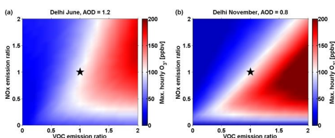
Figure 3. Daily maximum hourly ozone in Delhi as a function of NO x and VOC emissions in (a) summer (June) and (b) winter (November). Current conditions are marked by a black star.
