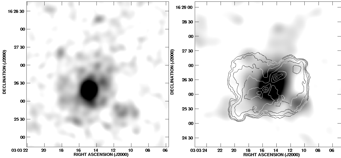
Figure 4. The X-ray environment of 3C 76.1. Images made from the combined MOS1, MOS2 and pn events lists in the 0.5 - 5.0 keV energy range, with exposure correction to correct for chip gaps but not vignetting, as described in the text. Left: image smoothed with a Gaussian of FWHM 5.2 arcsec; right: smoothed with a Gaussian of FWHM 10.4 arcsec and with 1.4-GHz radio contours overlaid.
