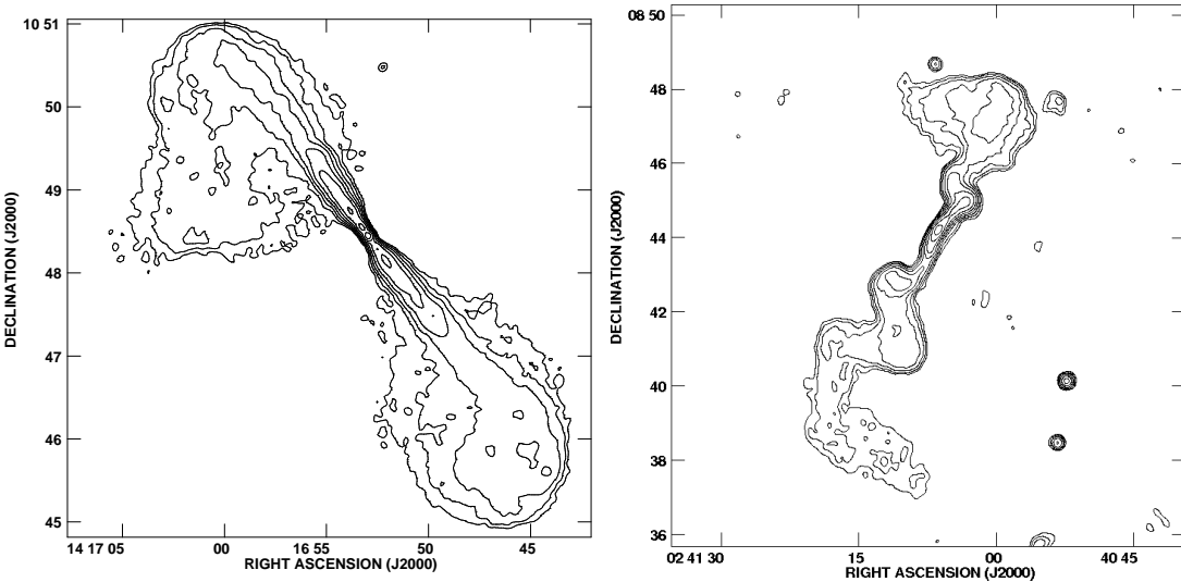
Figure 9. Examples of the two morphological classes of FRI radio galaxies, as described in the text. L: a typical “bridged” source, 3C 296, in which the lobe material is primarily between the nucleus and the end of the collimated jet; R: a typical “plumed” source, NGC 1044, in which the lobe material is primarily beyond the end of the collimated jet.
