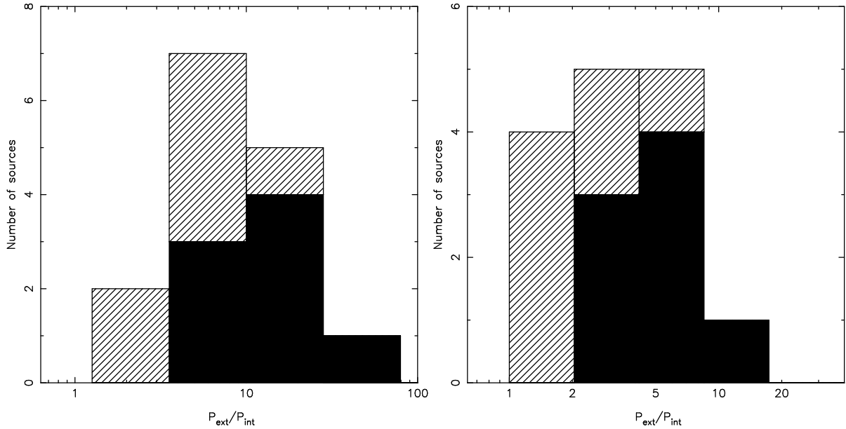
Figure 12. Histograms of the P_{ext}/P_{int} , the ratio of external to internal (equipartition) pressure for the full sample. The left panel is for pressures at the midpoint of the radio lobe and the right panel for pressures at the outermost of edge of the radio lobe. The sample is subdivided into bridged (hatched) and plumed (solid black) lobes. For all except NGC 6251 and NGC 315, both lobes are plotted.
