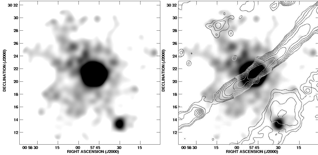
Figure 1. The X-ray environment of NGC 315. Images made from the combined MOS1, MOS2 and pn events lists in the 0.5 - 5.0 keV energy range, with exposure correction to correct for chip gaps but not vignetting, as described in the text. Left: smoothed with a Gaussian of FWHM 33 arcsec to show the group-scale emission. Right: with 1.4-GHz radio contours (Laing et al. 2006) overlaid.
