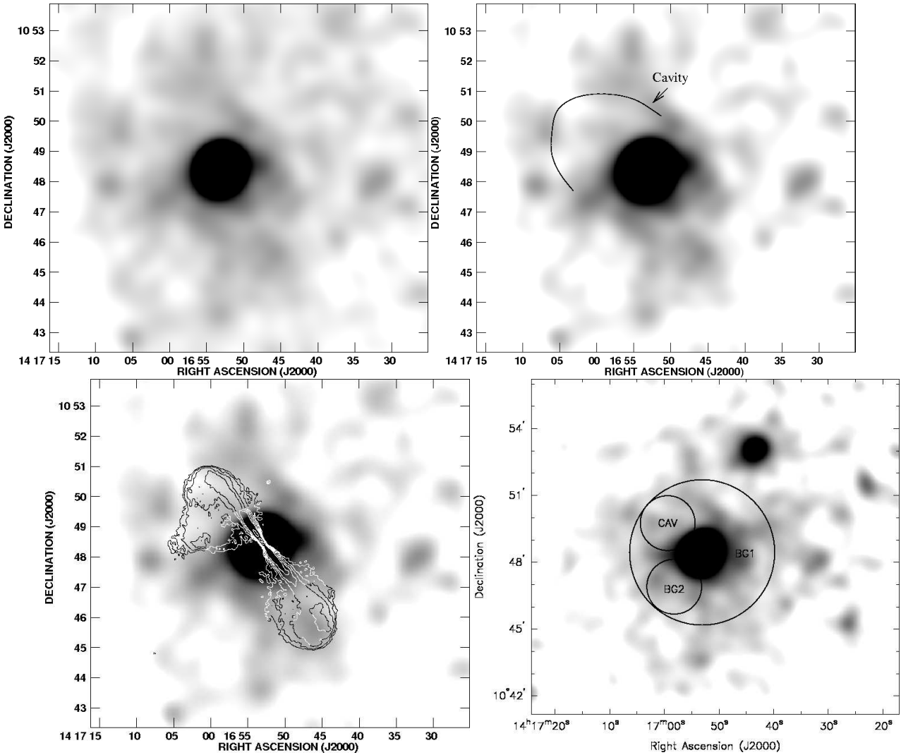
Figure 6. The X-ray environment of 3C 296. Images made from the combined MOS1, MOS2 and pn events lists in the 0.5 - 5.0 keV energy range, with exposure correction to correct for chip gaps but not vignetting, as described in the text. Images are smoothed with a Gaussian of FWHM 19 arcsec. Top left: group emission; top right: cavity to the NE highlighted; bottom left: with 20-cm radio contours overlaid illustrating that the northern lobe fills the cavity seen in the top right panel; bottom right: regions used to investigate significance of cavity detection.
