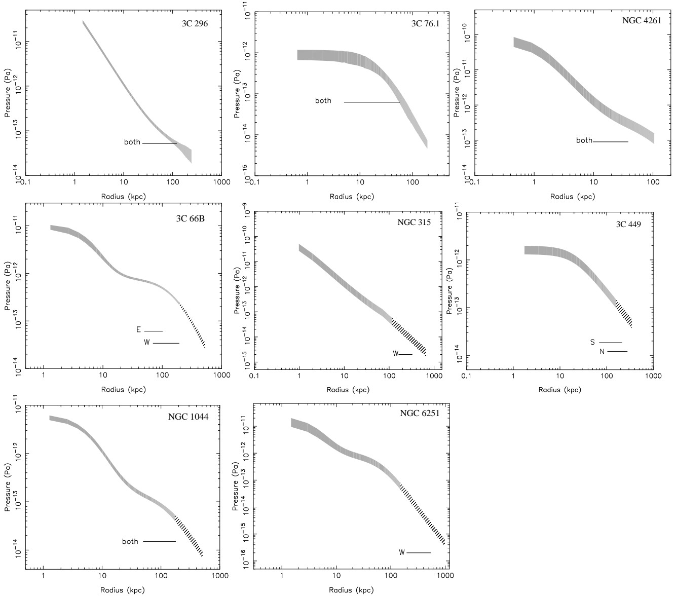
Figure 8. Pressure profiles for the XMM-observed radio-galaxy environments. The grey shaded area indicates the 1\sigma uncertainty, which takes into account uncertainties in all the model parameters and in the temperature measurement. Hatched regions indicate an extrapolation of the pressure profile model beyond the region covered by the data. Horizontal lines indicate internal pressures of radio lobes. Top row (l-r): the bridged sources 3C 296, 3C 76.1, NGC 4261; middle row: the plumed sources 3C 66B, NGC 315, and 3C 449; bottom row: NGC 1044, and NGC 6251.
