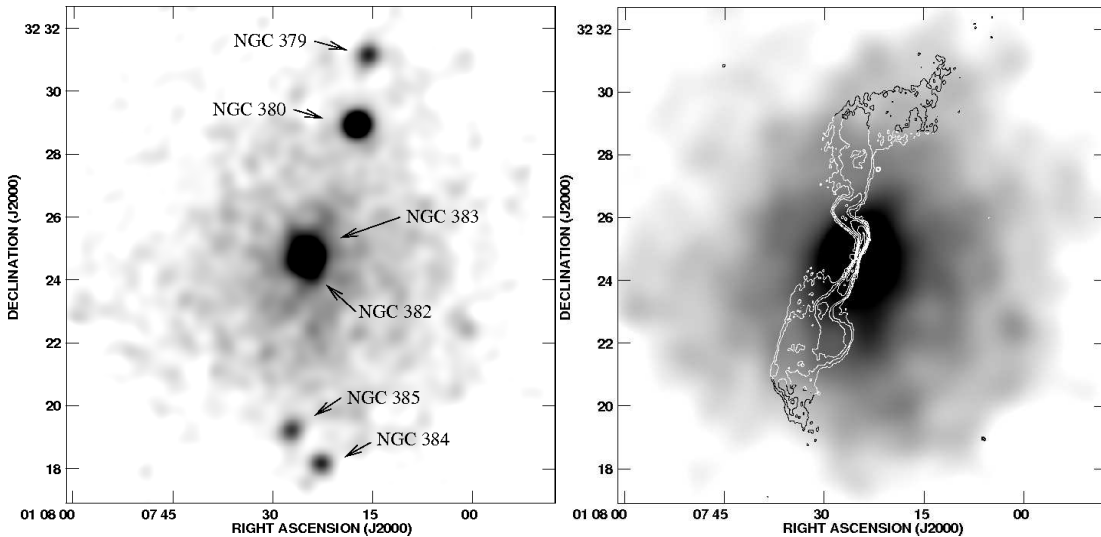
Figure 2. The X-ray environment of 3C 31. Images made from the combined MOS1, MOS2 and pn events lists in the 0.5 - 5.0 keV energy range, with exposure correction to correct for chip gaps but not vignetting, as described in the text. Left: smoothed with a Gaussian of FWHM 13 arcsec to highlight the emission associated with several of the NGC 383 group galaxies. The central galaxy is NGC 383, with a slight elongation to the south west due to emission from its companion galaxy NGC 382; right: smoothed with a Gaussian of FWHM 26 arcsec to highlight the group-scale emission, and with galaxy emission removed, overlaid with 1.6-GHz radio contours (Laing et al. 2008).
