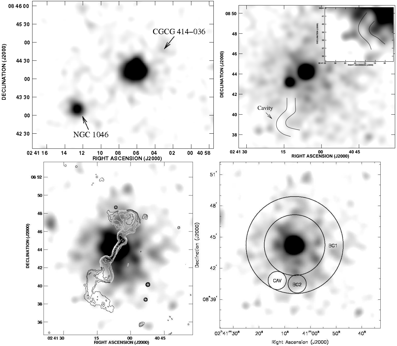
Figure 3. The X-ray environment of NGC 1044. Images made from the combined MOS1, MOS2 and pn events lists in the 0.5 - 5.0 keV energy range, with exposure correction to correct for chip gaps but not vignetting, as described in the text. Top left: smoothed with a Gaussian of FWHM 13 arcsec to highlight the emission associated with several of the NGC 1044 group galaxies; top right: the same image smoothed with a Gaussian of FWHM 20 arcsec and with galaxy emission removed to show the group-scale emission and cavity to the S; an inset shows a close-up of the cavity region from an image smoothed with a Gaussian of FWHM 26 arcsec; bottom left: image smoothed with a Gaussian of FWHM 26 arcsec to highlight the group emission, with 1.4-GHz radio contours overlaid illustrating that the southern radio plume fills the cavity shown in the middle panel; bottom right: regions used to investigate significance of cavity detection.
