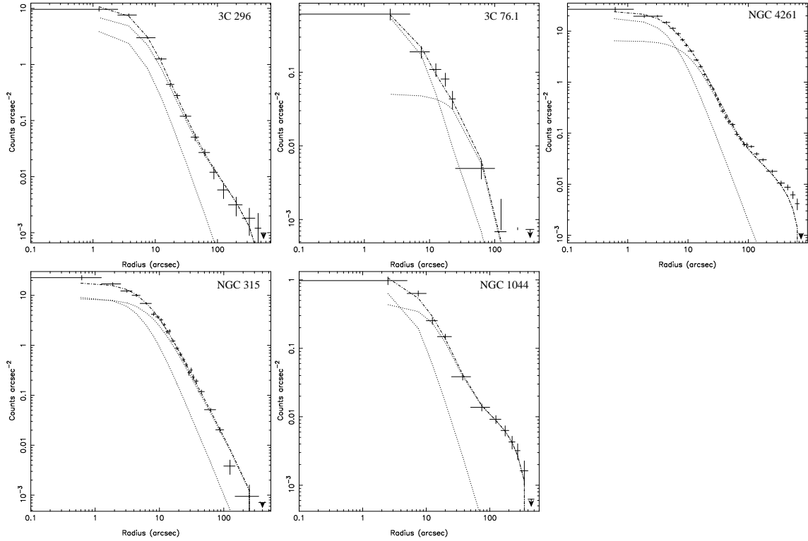
Figure 7. EPIC pn surface brightness profile with best-fitting point source plus \beta model or projb model, as discussed in the text, for the newly observed galaxies. Top row (l-r): the bridged sources 3C 296, 3C 76.1, NGC 4261; bottom row: the plumed sources NGC 315 and NGC 1044. (The somewhat poor fit in the outer regions for NGC 4261 is because the model is from the best joint fit, rather than the best fit to the pn profile alone).
