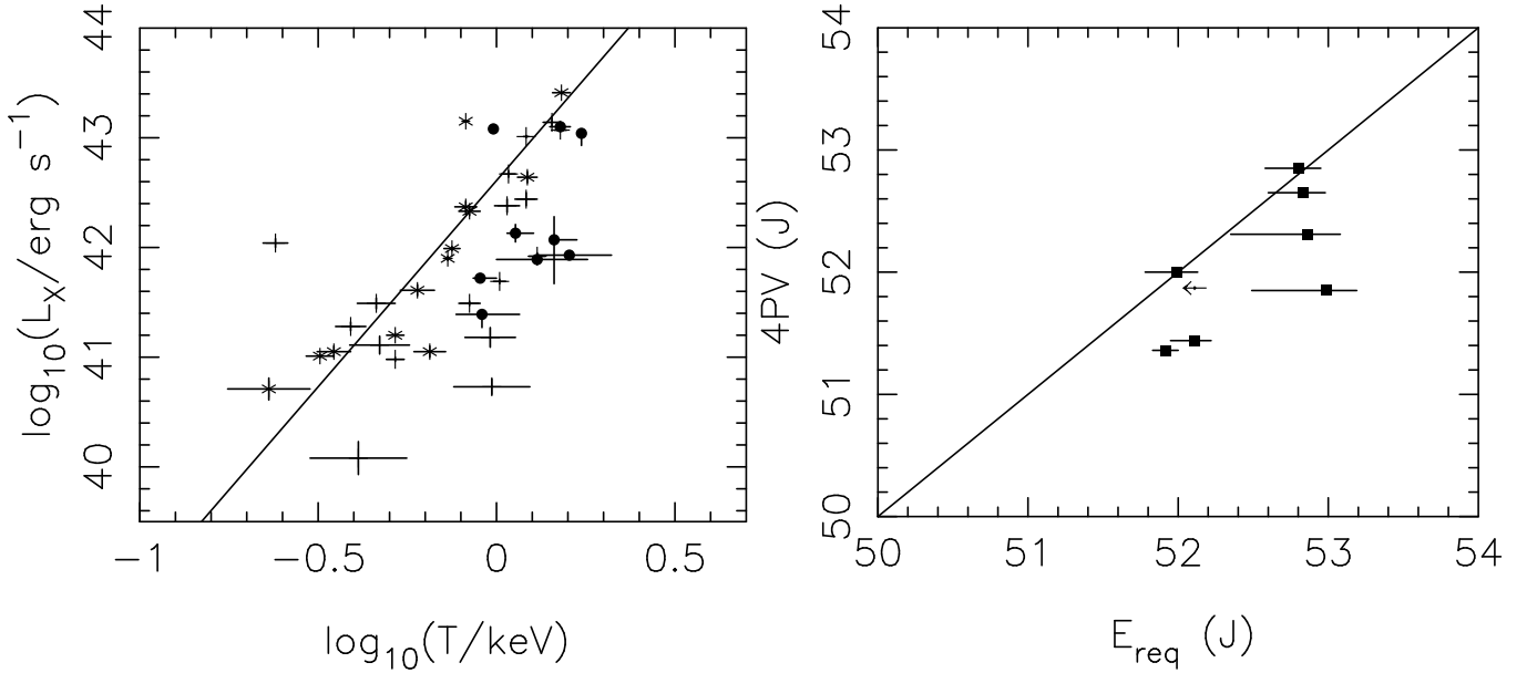
Figure 13. Left: The L_X/T_X relation for the XMM-Newton radio-galaxy environments sample (filled circles) compared with the radio-quiet (x symbols) and radio-loud (+ symbols) samples of Croston et al. (2005a). Solid line indicates the best-fitting relation for radio-quiet groups. Right: The energy required to produce the observed temperature offsets ( C\Delta T ) vs. energy available from the current radio source ( 4PV ). Solid line is the line of equality.
