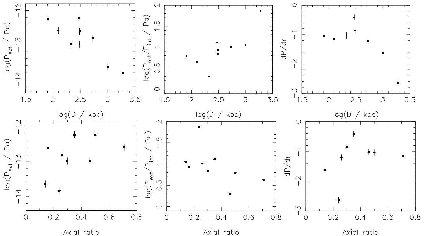
Figure 10. Correlations between radio structure and group gas properties. Top: Size vs. external pressure (left), pressure ratio ( P_{ext}/P_{int} ) (middle), and pressure gradient (right); bottom: Axial ratio vs. external pressure (left), pressure ratio ( P_{ext}/P_{int} ) (middle), and pressure gradient (right).
