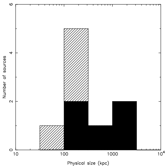
Figure 11. Histograms of radio-source size for the bridged (hatched) and plumed (solid black) sources, showing a statistically significant difference in their distributions.
