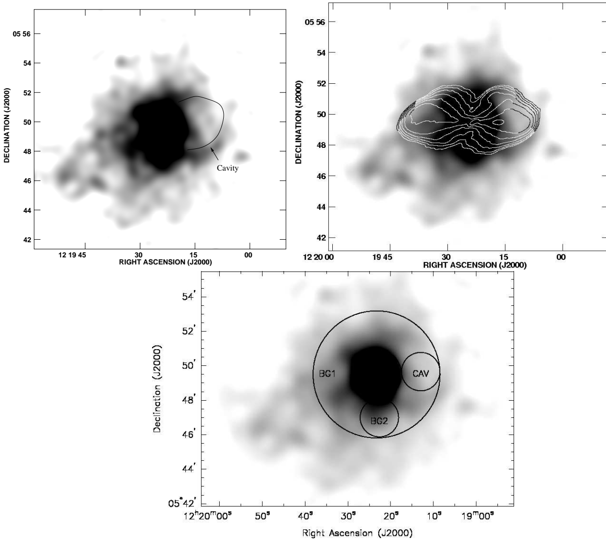
Figure 5. The X-ray environment of NGC 4261. Images made from the combined MOS1, MOS2 and pn events lists in the 0.5 - 5.0 keV energy range, with exposure correction to correct for chip gaps but not vignetting, as described in the text. Top left: smoothed with a Gaussian of FWHM 26 arcsec and with galaxy emission removed to show the group-scale emission and cavity to the W; top right: smoothed with a Gaussian of 33 arcsec and with 1.4-GHz radio contours overlaid illustrating that the W lobe coincides with the cavity in the group-scale gas; bottom: regions used to investigate significance of cavity detection.
