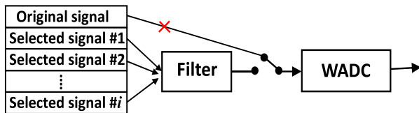
FIGURE 5. WADC with filter.
