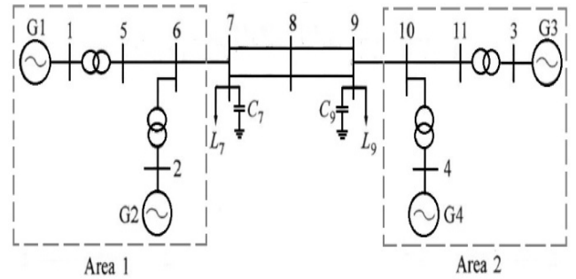
FIGURE 6. Two-area system.
