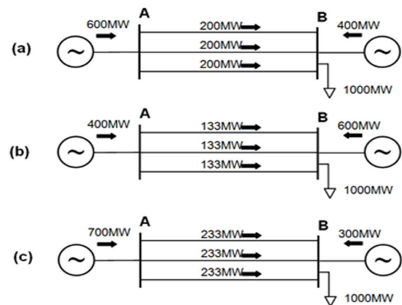
FIGURE 1. Two-Bus power system. (a) Unsecured operation (i.e. pure economic dispatch). (b) Operation under the N-1 security rule (i.e. security-constrained dispatch). (c) Security constrained dispatch when the capacity of each line is increased to 350 MW.
