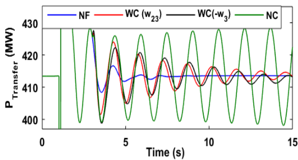
FIGURE 10. Responses when \Delta\omega_1 is lost and \Delta\omega_{23} or -\Delta\omega_3 is used as input.
