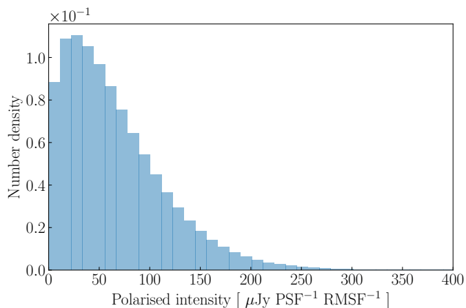
Fig. 6. Histogram of polarised intensity of the mosaic at Faraday depth \Phi = -50 \text{rad m}^{-2} (Fig. 7). The width of this distribution, approximated by the standard deviation multiplied by \sqrt{2} , gives an estimate of the noise level in the mosaic, 71 \mu\text{Jy PSF}^{-1} \text{RMSF}^{-1} , while its mean gives the polarisation bias, 66 \mu\text{Jy PSF}^{-1} \text{RMSF}^{-1} .
