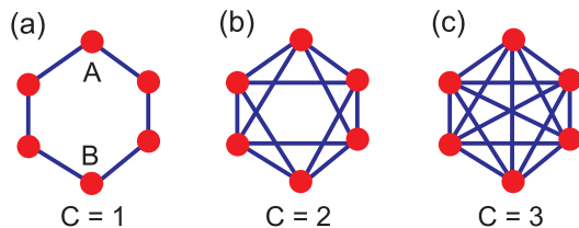
FIG. 1: (Color online) A circulant spin network can be used to transfer quantum states from A to B. In a network of N = 6 spins there are three possible configurations with connectivity (a) C = 1 , (b) C = 2 , and (c) C = 3 , as shown. Network (b) is a 3-cross polytope graph (CPG).
