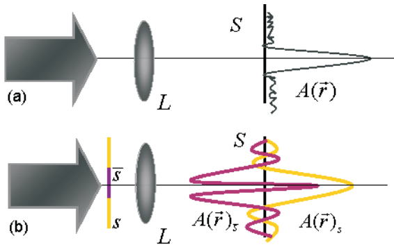
FIG. 3: (Color online) Illustration of Babinet's principle in an optical set up with Fraunhofer conditions. (a) An unobstructed plane wave is focused by a lens L and produces a diffraction pattern of amplitude A(\vec{r}) on the screen S . (b) Diffraction patterns resulting from complementary screens s and \bar{s} , whose opaque and transparent areas are swapped. At any point downstream from s and \bar{s} , the sum of the two diffracted amplitudes, A_s(\vec{r}) + A_{\bar{s}}(\vec{r}) , equals the amplitude diffracted from the unobstructed plane wave A(\vec{r}) . Away from the central spike, this amplitude is zero and therefore A_s(\vec{r}) = -A_{\bar{s}}(\vec{r}) , which leads to Babinet's prediction of identical diffracted light fields for complementary apertures. Complementary apertures play the role of complementary graphs describing quantum spin networks. Increasing \vec{r} corresponds to increasing the number of nodes N .
