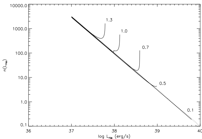
FIG. 3.—Computed models of H II region LFs with constant gas-to-dust ratio. Each solid curve corresponds to a value of integrated dust optical depth (at the H \alpha wavelength) for a region with emitted H \alpha luminosity of \log L_{\text{H}\alpha} = 38 ( L_{\text{H}\alpha} in ergs per second). The dotted curve represents the unextinguished LF.
