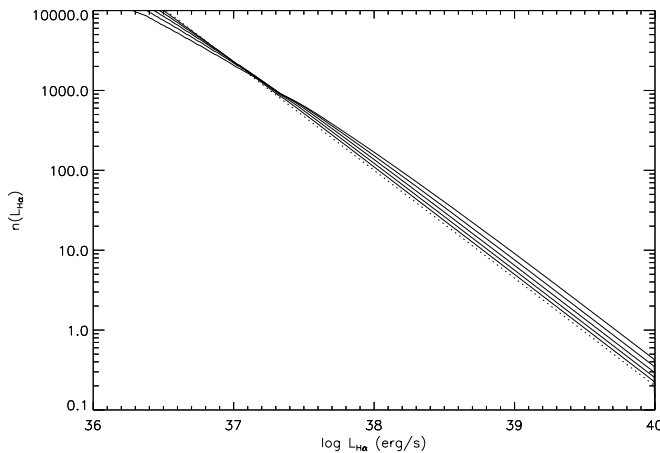
FIG. 4.—Models of the LF in H \alpha in which increasing degrees of overlapping and absorption take place between H II regions (see text for details). Although we place little stress on the quantitative results, we can see qualitatively that the effect of assimilating regions within others is to reduce the LF slope at high L_{\text{H}\alpha} , not to increase the slope as observed.
