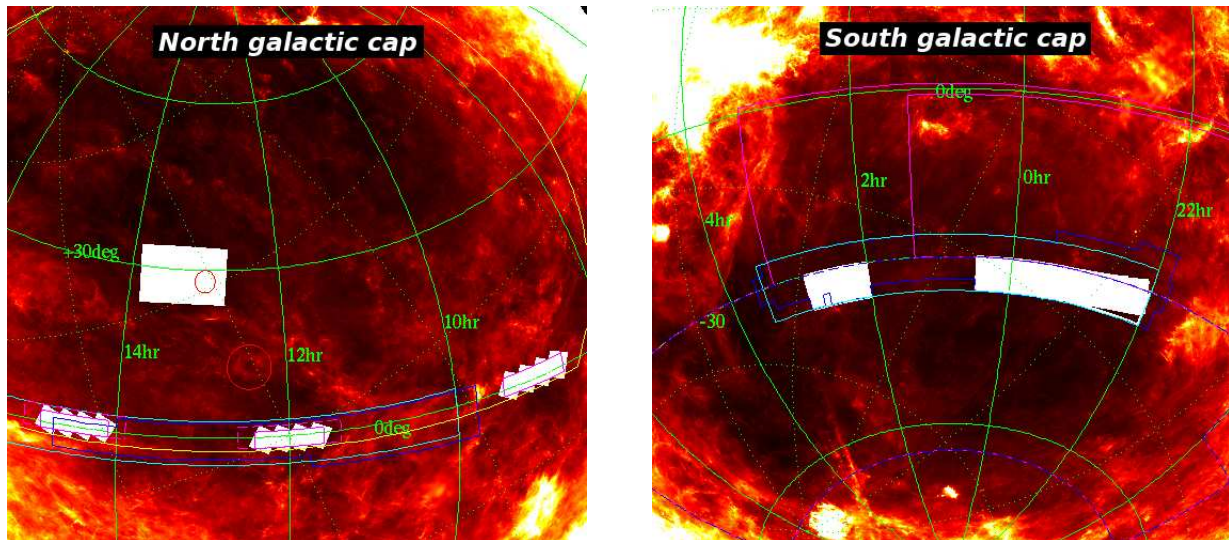
FIG. 2.— The positions of the ATLAS field, shown as white blocks, superimposed on the IRAS 100\ \mu\text{m} map of the sky, which traces the distribution of galactic dust. Figure 2(a) shows the northern galactic cap and Figure 2(b) shows the southern galactic cap. The colour coding for the lines is as follows: solid green lines—RA and dec; dotted green lines—ecliptic latitude and longitude; cyan—KIDS/VIKING area; yellow—SDSS area; blue—2dFGRS area; magenta—area of the Dark Energy Survey; magenta/blue dashed—area covered by the South Pole Telescope.
