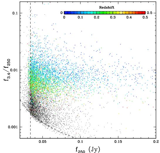
FIG. 2.— Distribution of the 3.4 - 250\ \mu\text{m} flux density ratio as a function of 250\ \mu\text{m} flux density for H-ATLAS sources with WISE 3.4\ \mu\text{m} IDs. Colored points have spectroscopic redshifts from the GAMA survey and sources without measured redshifts are indicated by black points. Dashed lines indicate the approximate limits of the H-ATLAS and WISE surveys. The majority of sources with spectroscopic redshifts ( z \lesssim 19.4 ) are well detected by WISE , while the no-redshift sources have small flux density ratios that are inconsistent with “normal” low-redshift galaxies.
