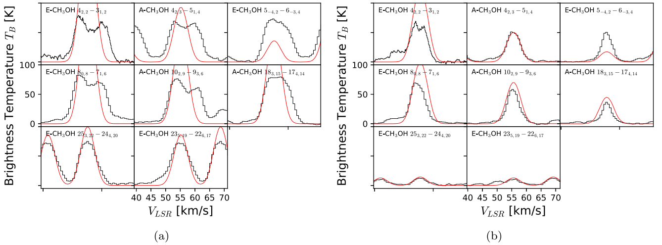
Figure 8. Spectra of the CH 3 OH lines toward a pair of selected pixels just outside of the central e2e core. (a) is 0''55 and (b) is 1''33 from e2e. The red curves show the LTE model fitted from a rotational diagram as shown in Figure 7. The model is not a fit to the data shown, but is instead a single-component LTE model fit to the integrated intensity of the lines shown. As such, the fit is not convincing, and it is evident that a single-temperature, single-velocity model does not explain the observed lines. Nonetheless, a component with the modeled temperature is likely to be present in addition to a cooler component responsible for the self-absorption in the low-J lines. (a) shows a pixel close to the center of e2e, which is probably optically thick in most of the shown transitions, while (b) shows a better case where the highest- A_{ij} (highest critical density) lines are overpredicted but many of the others are well-fit.
