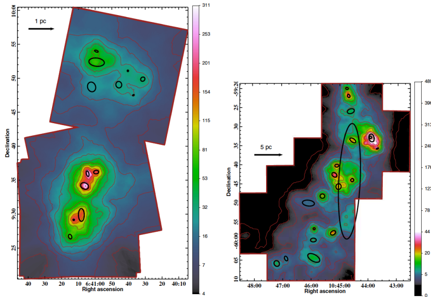
Fig. 2 The smoothed projected stellar surface density from the Massive Young Star-Forming Complex Study in Infrared and X-ray (MYStIX, Feigelson et al., 2013) is shown with a color bar in units of observed stars \text{pc}^{-2} . The brown contours show the increase in surface density by factors of 1.5. The ellipses mark the core regions of the isothermal ellipsoids. To identify the subclusters and to estimate the model parameters of the young stars a finite mixture model with a maximum likelihood estimation was used. The left panel shows NGC 2264 while the right panel shows the Carina star-forming region. This figure was published as part of Fig. 2 in Kuhn et al. (2014).
