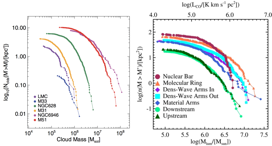
Fig. 6 Cumulative GMC mass spectra normalised by the observed area for different galaxies (left; from Hughes et al. 2016) and for different regions of the spiral galaxy M51 (right; from Colombo et al. 2014). The differences in slopes and maximum masses in different galaxies and for different kinematic environments of a given galaxy suggest an environmental dependence of the GMC mass distribution.
