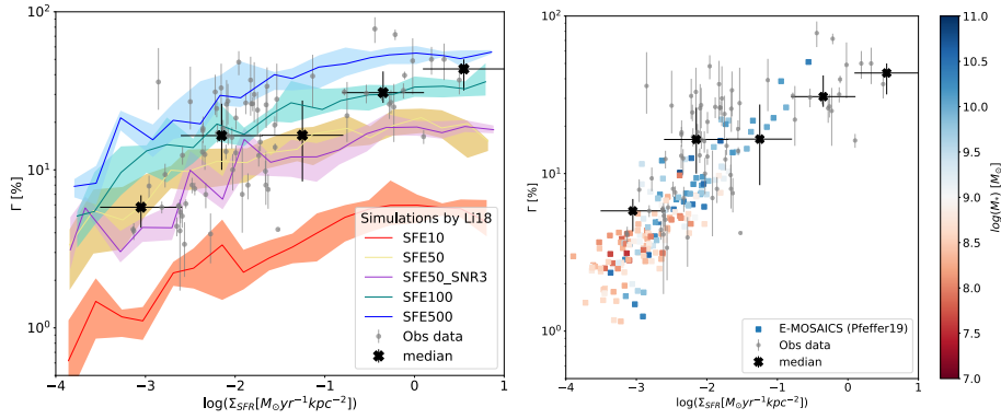
Fig. 9 \Gamma vs. \Sigma_{\text{SFR}} plane. We combine the observed data available in the literature (filled grey symbols), i.e. the data are not separated by age ranges used to estimate \Gamma (see Section 7 and Figure 8 for description of the observed data). We also include median and 25 and 75 % quartiles of the observed data (filled black symbols) estimated in \Sigma_{\text{SFR}} bins, of size indicated by the horizontal bars. Left : We include the resulting \Gamma vs. \Sigma_{\text{SFR}} extracted from the simulation sets by Li et al. (2018). The curves show the median and quartiles of different sets of simulations using different feedback prescriptions. Right : We include the extracted \Gamma and \Sigma_{\text{SFR}} for the E-MOSAICS simulations (filled square symbols) by Pfeffer et al. (2019b). The values have been extracted from galaxies at redshift 0 and are plotted color-coded by the galaxy stellar mass in the same snapshot.
