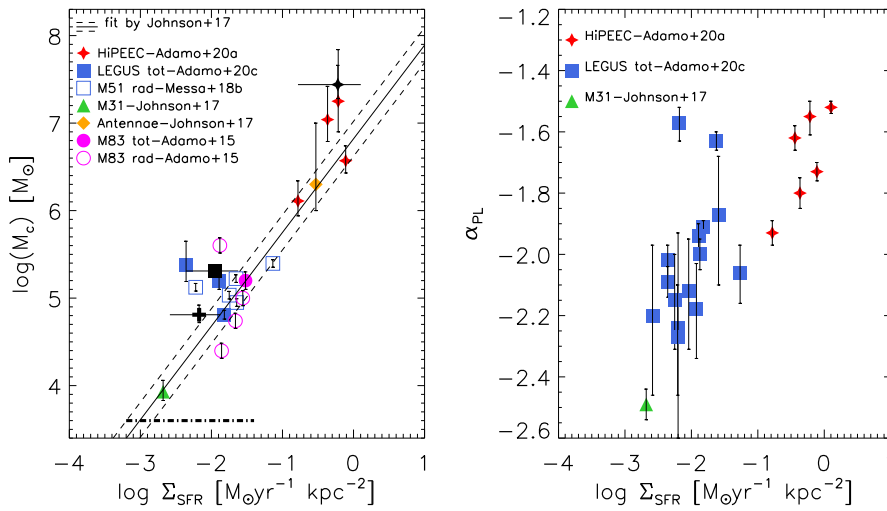
Fig. 10 Left: Truncation mass, M_c , vs. the star formation rate density plane. To the initial data points used by Johnson et al. (2017), we have added literature data (Messa et al., 2018a) and newly determined M_c in single galaxies from the LEGUS (blue filled squares, Adamo et al, 2020c to be subm.) and HIPEEC (red filled diamonds, Adamo et al 2020a to be subm.) sample. Only statistically significant determinations of M_c are reported. Black symbols are the recovered M_c reported in Table 2 and obtained by combining the cluster catalogues of 8 LEGUS spiral galaxies with \text{SFR} < 0.5 M_{\odot} \text{yr}^{-1} ( lowSFR spirals, black cross), 6 spiral galaxies with \text{SFR} > 0.5 M_{\odot} \text{yr}^{-1} ( highSFR spirals, black square), 6 merger systems belonging to the HiPEEC sample ( \text{SFR} > 10 M_{\odot} \text{yr}^{-1} , black diamond). The horizontal bar associated with each black symbol shows the \Sigma_{\text{SFR}} interval that each sample spans (see main text). The range of \Sigma_{\text{SFR}} of the dwarf sample is plotted as a dot-dashed horizontal line. Right: Power-law slope of the cluster mass function vs. star formation rate surface density. Values plotted in this plot are reported by Johnson et al. (2017), and Adamo et al (2020a, c, to be subm.).
