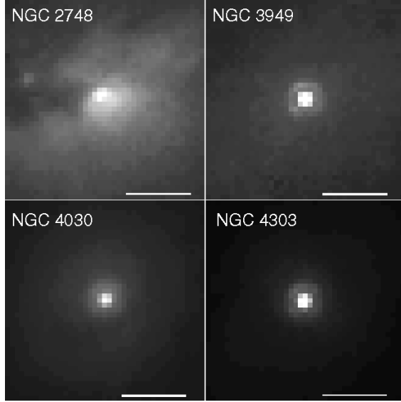
Fig. 5.— The archival NICMOS f160w images for the 4 central source candidates. Cut levels have been adjusted to highlight the nuclei. The white bar shows a scale of 1". The image for NGC 2748 shows that the presence of significant amounts of dust is the likely cause of the inflexion in the surface brightness profile. The central sources in the other galaxies are not much different to the size of the NICMOS PSF (see also figure 6), as can be seen by the presence of Airy rings
