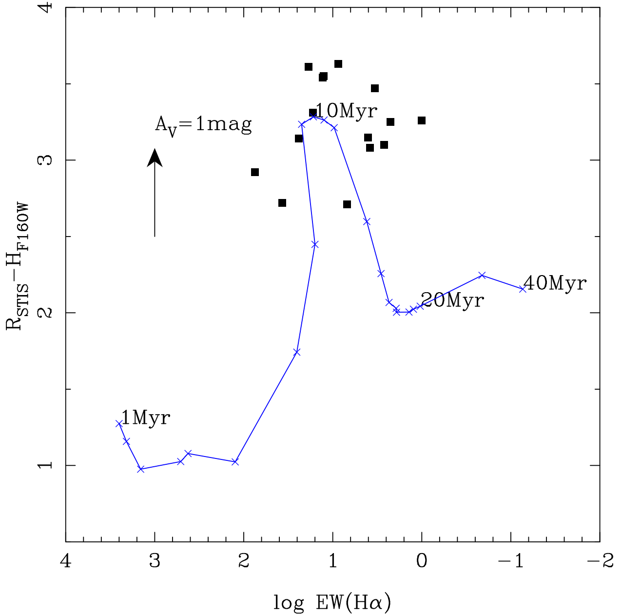
Fig. 8.— The R-H color index against H\alpha equivalent width for 100 pc apertures placed on the on-nucleus spectra. The model population is the same as in figure 7. This is much more useful than the plot in figure 7 as it suggests the age range of the central stellar populations is \sim 10 -20 Myr. The points correspond to those galaxies where both color and H\alpha spectral information was available and not just those with obvious central sources apparent in their surface brightness profiles.
