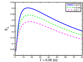
FIG. 5: System's response for a chain of N = 4 qubits with J/\Omega = 1.5 as quantified by the dynamical measure \mathcal{S}_4 = \langle \sum_{i=1}^4 \sigma_x^i / 4 \rangle as a function of the noise strength \Gamma J_i/\Omega_i = 1.5 and \Gamma_i/\Omega_i = 1 , and for different values of the external temperature.
