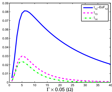
FIG. 3: System's response for a chain of N = 4 qubits at T = 0 with J_i/\Omega_i = 1.5 , ( i = 1 \dots 4 ) as quantified by an information theoretic measure, the quantum mutual information. Under the evolution given by H_{\text{eff}} , entanglement is restricted to nearest neighbours only and E_{F_{13}} = E_{F_{14}} = 0 .
