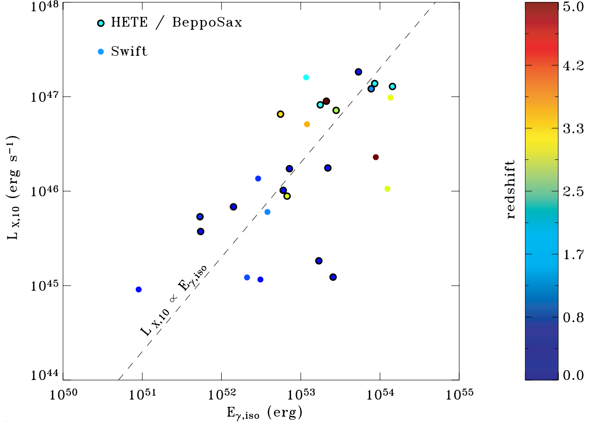
Fig. 6.— Distribution of L_{X,10} (2 – 10 keV) versus E_{\gamma, \text{iso}} (20 – 2000 keV) for all Swift GRBs with established redshifts (from Table 1) plotted together with selected earlier events observed with HETE-II and BeppoSAX (Berger et al. 2003; Bloom et al. 2003).
