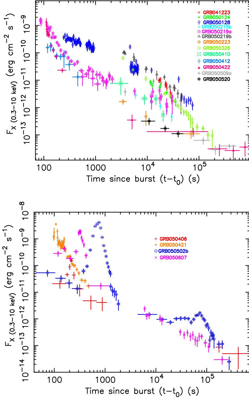
Fig. 2.— The X-ray flux (0.3 – 10 keV in the observer frame) as a function of the observed time, for all Swift GRBs without known redshifts, with ( lower panel ) and without ( upper panel ) X-ray flares.
