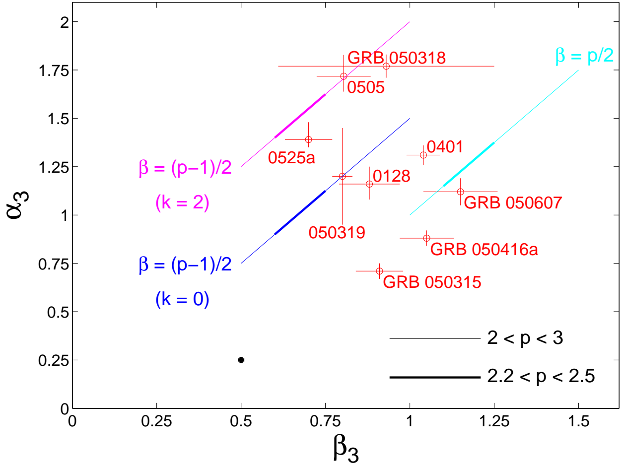
Fig. 9.— The values of \alpha_3 and \beta_3 for the GRBs in our sample for which t_{\text{break},2} could be determined. Other symbols as in Fig 8.
