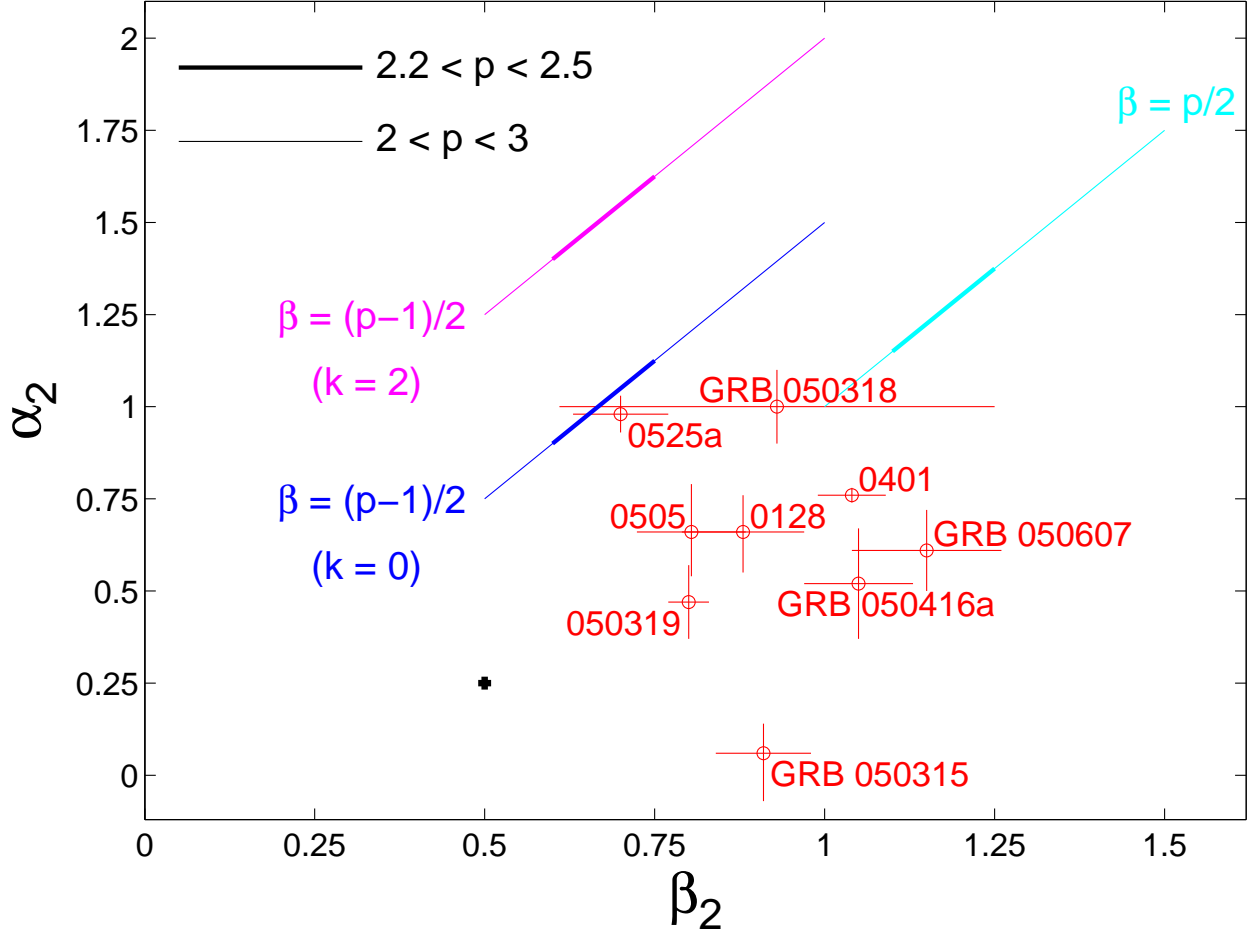
Fig. 8.— The values of \alpha_2 and \beta_2 for the GRBs in our sample for which t_{\text{break},2} could be determined, as well as the values expected for an adiabatic evolution of a spherical afterglow shock (Sari, Piran & Narayan 1998; Granot & Sari 2002). In most relevant power law segments of the spectrum both \alpha and \beta depend on p , and therefore we drew a thick (thin) line corresponding to the range 2.2 < p < 2.5 ( 2 < p < 3 ) which is both typically inferred from GRB afterglows, and is preferred on theoretical grounds. The cross at \alpha_2 = 1/4 and \beta_2 = 1/2 corresponds to the fast cooling power law segment of the spectrum, \nu_c < \nu < \nu_m , where both \alpha and \beta are independent of p and k .
