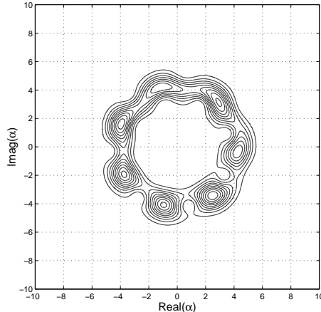
Fig. 6. Q -function for the dynamical evolution of the system at 1 \times 10^{-2} s.
