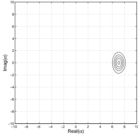
Fig. 2. Q -function for a Bose condensed gas in the Thomas-Fermi approximation.
