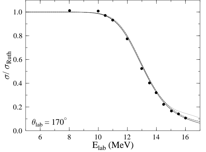
FIG. 10. Excitation function of ^{92}\text{Mo}(\alpha,\alpha)^{92}\text{Mo} scattering at \vartheta_{\text{lab}} = 170^\circ normalized to the Rutherford cross section. The experimental data are taken from Ref. [49]. The dotted (dashed, full) curves have been calculated from potentials which were adjusted to the 13 (16, 19) MeV angular distributions.
