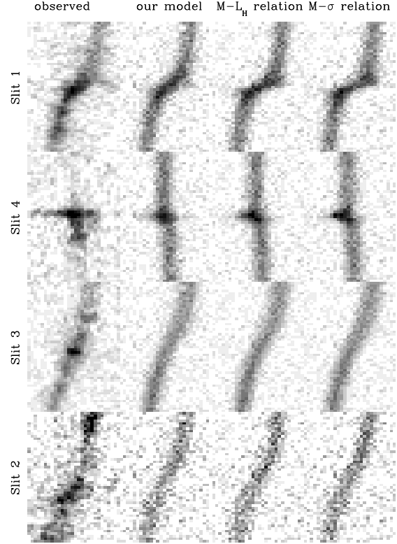
Figure 14. Comparison between the observed two-dimensional spectra ( left panels ) and the two-dimensional synthetic spectra for (i) the best-fitting model, (ii) a model with M_{\bullet} = 4 \cdot 10^7 M_{\odot} as predicted by the near-infrared M_{\bullet}-L_{bulge} relation, and (iii) a model with M_{\bullet} = 5 \cdot 10^7 M_{\odot} as predicted by the M_{\bullet}-\sigma_c relation for the different slit positions. In the models we added a random noise in order to mimic the actual S/N ratio of the observed spectra. Each box is 15 \text{ \AA} \times 2.6 \text{ arcsec} .
