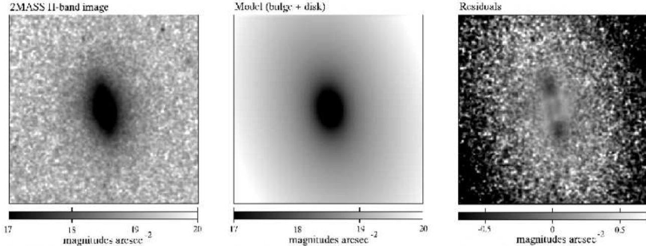
Figure 13. Two-dimensional photometric decomposition of the surface-brightness distribution of NGC 4435. Left panel: Background- and star-subtracted H -band image of NGC 4435 from the 2MASS archive. Central panel: Galaxy model as derived from the photometric decomposition. The bulge is modeled with a Sérsic law ( n = 2.39 , R_e = 11''.14 , \mu_e = 16.10 mag arcsec ^{-1} and b/a = 0.64 ) the disc is modeled with an exponential law ( h = 104''.41 , \mu_0 = 18.15 mag arcsec ^{-1} and b/a = 0.60 ). Right panel: Residuals of the model. Images are 3 arcmin \times 3 arcmin.
