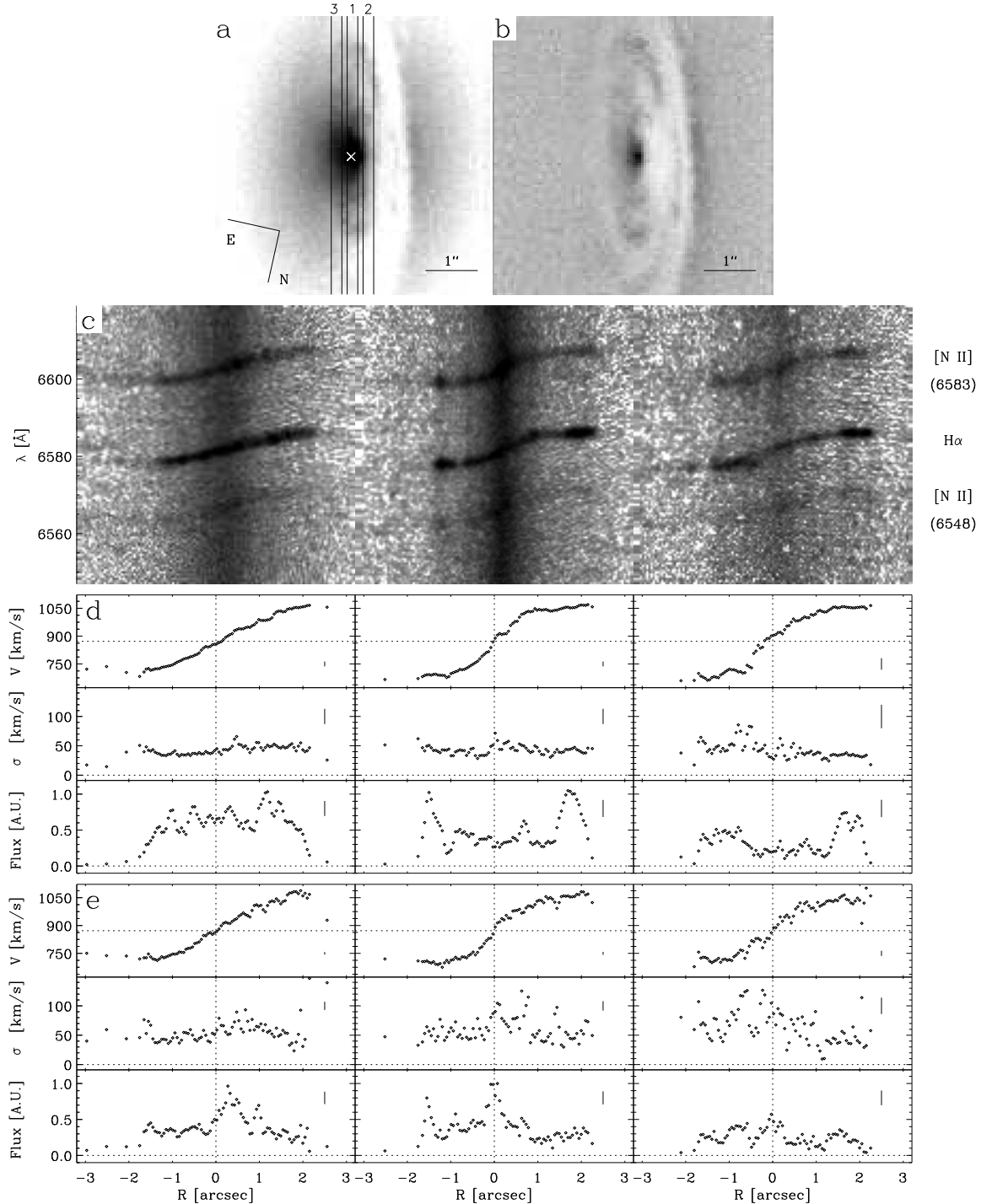
Figure 1. a) HST STIS/F28X20LP acquisition image of NGC 4435. The image has been rotated to the STIS instrumental frame. Orientation and scale are given. The white cross is the position of the nucleus from STIS acquisition procedure. The rectangles overlotted on the image show the actual locations of the slit during the spectroscopic observations. Table 1 lists the offsets of slit position 1, 2, and 3 with respect to the location of the nucleus. b) Unsharp-masking of the acquisition image of NGC 4435. c) Portions of the bidimensional STIS spectra of NGC 4435 obtained in position 1 ( central panel ), 2 ( right panel ) and 3 ( left panel ). The spectral region centered on the H \alpha emission line is shown after wavelength calibration, flux calibration and geometrical rectification. The spatial axis is horizontal and ranges between -3.2 and +3.2 arcsec, while the wavelength axis is vertical and ranges from 6547 to 6619 Å. Individual emission lines are identified using a key, such that [N II] (6548), H \alpha , and [N II] (6583) correspond to [N II] \lambda 6548, H \alpha , and [N II] \lambda 6583, respectively. d) H \alpha kinematics from the spectra of NGC 4435 obtained in position 1 ( central panels ), 2 ( right panels ) and 3 ( left panels ). For each slit position the line-of-sight velocity curve ( top panel ), the radial profile of the line-of-sight velocity dispersion (uncorrected for instrumental velocity dispersion, middle panel ), and the radial profile of line flux in arbitrary units ( bottom panel ) are given. Errorbars are not plotted for clarity, but the typical errors are shown on the right side of each plot. e) Same as in d) , but for the [N II] \lambda 6583 emission line.
