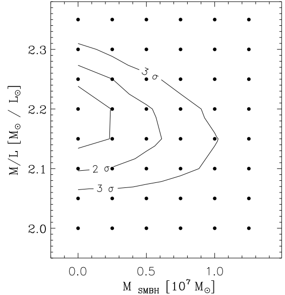
Figure 10. \chi^2 grid for models with different values of mass-to-light ratio and SMBH mass values. The continuous lines are the confidence levels on the best-fitting values of M_\bullet=0 M_\odot and (M/L)_\star=2.2 (M/L)_\odot .
