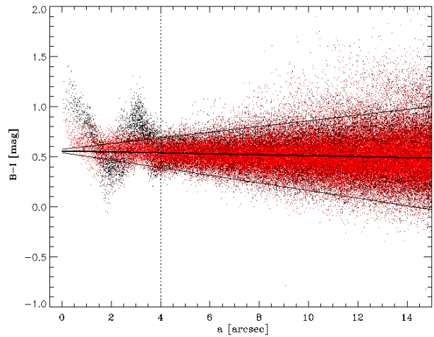
Figure 4. Calibrated Johnson B - I color for every pixel in the WFPC2 image of NGC 4435 as a function of its elliptical radius a . Black and red dots refer to pixel on the eastern and western side of the galaxy, respectively. The thick and two thin continuous lines correspond to fitted intrinsic color (B - I)_0 and E(B - I) thresholds, respectively. Thresholds have been derived for pixels at 4 < a < 15 arcsec and extrapolated to the innermost radii.
