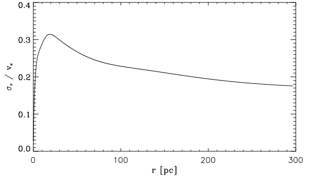
Figure 18. The ratio \sigma_r/v_c for the model with M_\bullet = 4 \cdot 10^7 M_\odot .
