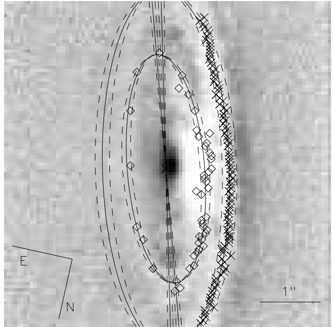
Figure 8. The orientation of the gaseous disc of NGC 4435. Diamonds and crosses corresponding to the points of the inner and outer dust lanes are overplotted to Figure 1b. Absorption features are brighter in this unsharp-masked image. The best-fit ellipses of the inner and outer dust lanes and their position angles are shown with solid ellipses and solid lines , respectively. The dashed ellipses and dashed lines enclose the 1\sigma confidence ranges on best-fit ellipticity and position angle for both the isophotes.
