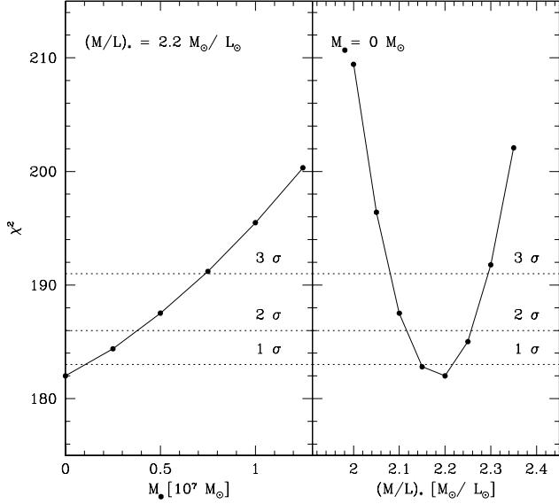
Figure 9. \chi^2 as a function of M_\bullet (left panel) and (M/L)_\star (right panel). The dotted horizontal lines indicate the confidence levels on the best fitting values of M_\bullet=0 M_\odot and (M/L)_\star=2.2 (M/L)_\odot .
