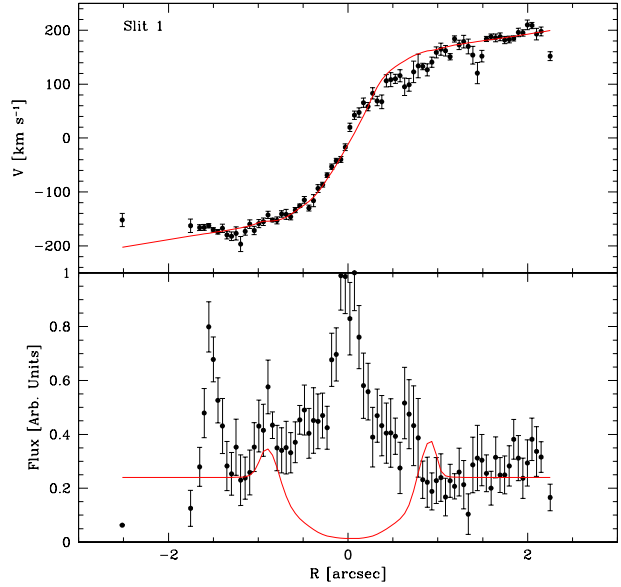
Figure 17. Observed [N II] \lambda 6583 (filled circles) and fitted (solid lines) kinematics in the innermost \pm 2.5 arcsec along the major axis of NGC 4435. The model is obtained using a M_{\bullet} = 4 \cdot 10^7 M_{\odot} , i = 70^{\circ} , \theta = 17^{\circ} , (M/L)_{\star} = 2.2 (M/L)_{\odot} , and an ad hoc flux distribution to reproduce the central gradient. The predicted flux radial profile is completely inconsistent with the observed one.
