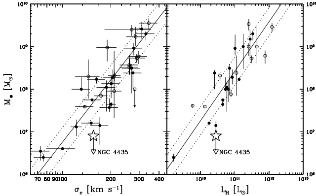
Figure 12. Location of the upper limit value of the SMBH mass of NGC 4435 with respect to the M_{\bullet}-\sigma_c relation by Ferrarese & Ford (2005, left panel ) and near-infrared M_{\bullet}-L_{bulge} relation by Marconi & Hunt (2003, right panel ). In the left panel, following Ferrarese & Ford (2005) we plot the SMBH masses based on resolved dynamical studies of ionized gas ( open circles ), water masers ( open squares ), and stars ( filled circles ). The upper limit of the SMBH mass of NGC 4435 (Verdoes Kleijn et al. 2002) has been included for sake of comparison (see Section 7). In the right panel we plot the SMBH masses for which H -band luminosity of the host spheroid is available in Marconi & Hunt (2003). In both panels dotted lines represent the 1\sigma scatter in M_{\bullet} .
