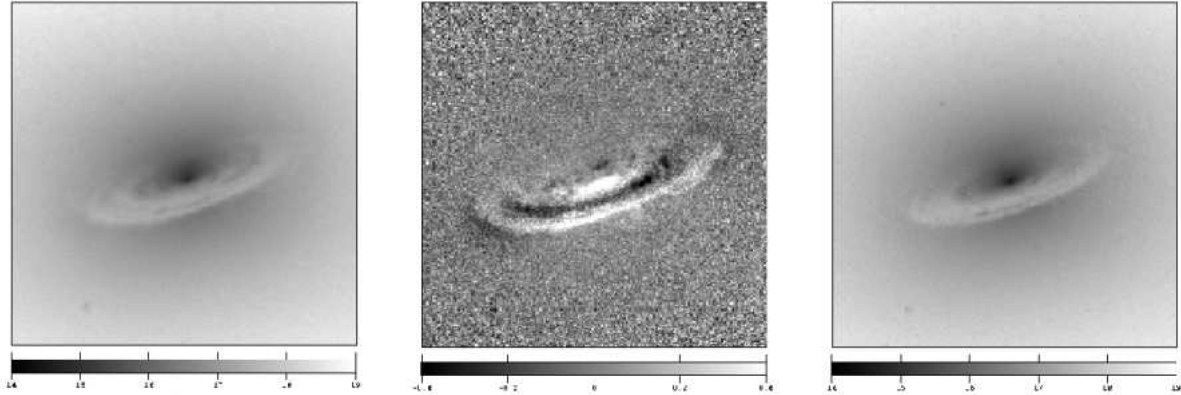
Figure 5. Dust correction of the WFPC2/F814W image of NGC 4435. Left panel: Observed WFPC2/F814W image after calibration to Johnson I -band. Middle panel: Map of the color excess E(B - I) . Right panel: Extinction-corrected I -band image. The field of view is 10.6 \times 10.6 arcsec 2 and the color scale is given in magnitudes.
