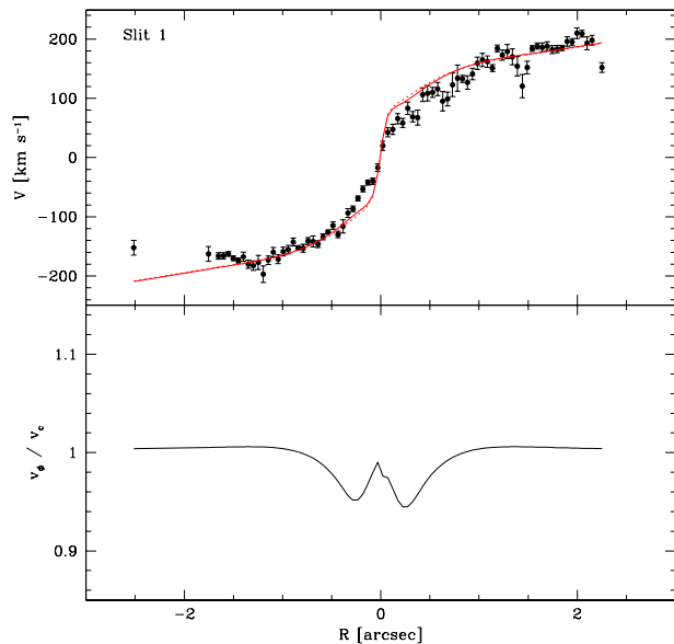
Figure 19. Upper panel: The observed [N II] \lambda 6583 (filled circles) along the the major axis of NGC 4435 is compared to the one obtained with M_\bullet = 4 \cdot 10^7 M_\odot , (M/L)_* = 2.2 (M/L)_\odot , \theta = 17^\circ and i = 70^\circ with (solid line) and without (dashed line) applying the asymmetric drift correction. Lower panel: Ratio between the rotation curves obtained with and without applying the asymmetric drift correction.
