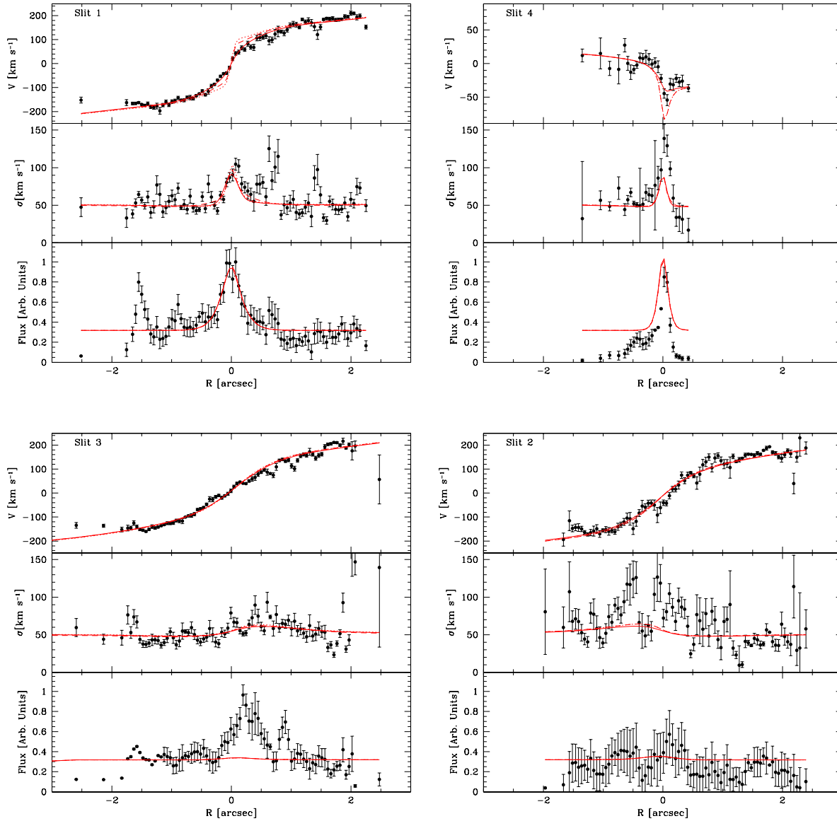
Figure 11. Observed [N II] \lambda 6583 kinematics (filled circles) along with the best-fitting model (solid line) and model predictions for the SMBH masses of NGC 4435 derived in Section 5.4 from the M_{\bullet}-\sigma_c relation by Ferrarese & Ford (2005, M_{\bullet} = 5 \cdot 10^7 M_{\odot} , dotted line) and from the near-infrared M_{\bullet}-L_{bulge} relation by Marconi et al. (2003, M_{\bullet} = 4 \cdot 10^7 M_{\odot} , dashed line). The observed and modeled velocity curve (top panel), velocity dispersion radial profile (middle panel) and flux radial profile (bottom panel) are shown for slit along the major axis (slit #1, upper left panels), close to minor axis (slit #4, upper right panel), along eastern offset (slit #3, lower left panel), and western offset (slit #2, lower right panel).
