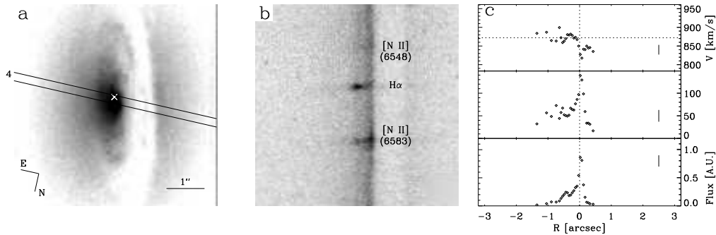
Figure 2. Similar to Figure 1, but for the archival spectrum of NGC 4435. The acquisition image of NGC 4435 with the slit location, a portion of the two-dimensional STIS spectrum after data reduction, and the [N II] \lambda 6583 kinematics are shown in panels a ), b ), and c ), respectively. In a ) the image orientation and scale is the same as in Figure 1a. In c ) the spatial axis ranges between -3.2 and +3.2 arcsec, and the wavelength axis ranges from 6549 to 6627 Å.
