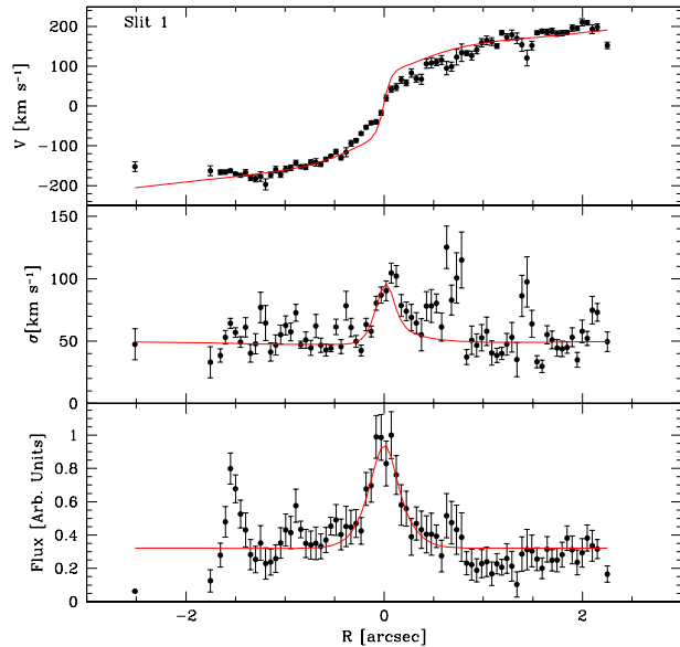
Figure 15. Observed [N II] \lambda 6583 (filled circles) and fitted (solid line) kinematics in the innermost \pm 2.5 arcsec along the major axis of NGC 4435 obtained with M_\bullet = 4 \cdot 10^7 M_\odot and ( M/L ) _\star = 2.2 (M/L)_\odot but allowing the position angle and inclination of the gaseous disc to vary. The central velocity gradient is not reproduced by any choice of disc inclination and position angle.
