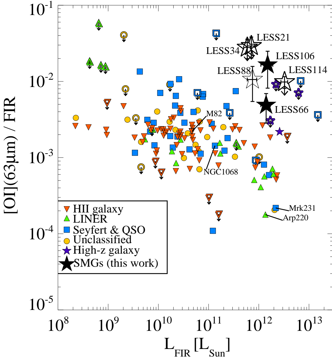
Figure 3. The observed [OI]63 \mu\text{m} -to-FIR continuum ratio as a function of L_{\text{FIR}} for SMGs from this paper (large black stars) compared with available literature values (compiled by Graciá-Carpio et al. 2011). The literature compilation includes all galaxies observed with ISO (Colbert et al. 1999; Negishi et al. 2001; Malhotra et al. 2001; Luhman et al. 2003; Dale et al. 2004; Brauer, Dale & Helou 2008) and with PACS (Graciá-Carpio et al. 2011). The high-redshift ( 1.13 < z < 3.04 ) galaxy comparison sample includes 3C 368 (Brauer, Dale & Helou 2008), SMMJ2135-0102 (Ivison et al. 2010), SDP.81 (Valtchanov et al. 2011), and MIPS J142824.0+352619 (Sturm et al. 2010), all of which have been corrected for gravitational lensing. Several familiar well-studied local galaxies are indicated on the plot for reference, including M82, NGC1068 (a LIRG), and ULIRGs Arp220 and Mrk231 (Fischer et al. 2010; Graciá-Carpio et al. 2011). The solid symbols represent the two SMGs with [OI]63 \mu\text{m} detections, and the open symbol represents the SMG which we have ‘tentatively’ detected. The open symbols with downward arrows indicate 3\sigma upper limits. In Section 3.2, we found that the FIR continuum flux and L_{\text{FIR}} are possibly underestimated by estimated factors of 2.8 and 1.7, respectively, for LESS21 and LESS34, and by factors of 1.6 and 1.5, respectively, for LESS106. Applying these correction factors to these SMGs would move these sources down and to the right in the plot by the same factors. The SMGs do not show an [OI]63 \mu\text{m} emission line deficit compared to local ULIRGs, similar to what is seen for the [CII]158 \mu\text{m} emission line for SMGs.
