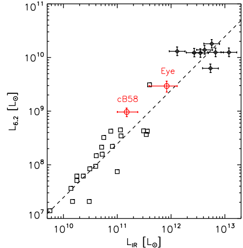
FIG. 7.— The 6.2 \mu\text{m} PAH strength vs. infrared luminosity. This figure is adapted from the top panel of Fig. 12 in Pope et al. (2008). Local starbursts (squares) are from Brandl et al. (2006) and high-redshift SMG (diamonds) are from Pope et al. (2008). The dashed line is the best-fit L_{6.2} -to- L_{IR} relation of Pope et al. (2008) for the low redshift starbursts. The L_{PAH}/L_{IR} ratios of the two lensed LBGs are consistent with the extrapolation (to higher luminosities) of the trend observed in local starbursts.
