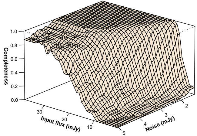
Figure 3. Completeness of the 450 \mu\text{m} catalogue as a function of local noise and input flux based on input-and-recovery simulations using jackknife realisations of the map noise. Modelling the completeness as a 2-dimensional function is required due to the radially varying sensitivity in the map (Fig. 1). The same simulations allow us to estimate the difference between true (input) flux and recovered (i.e. observed) flux densities across the same parameter space, and we use this information to correct the number counts accordingly.
