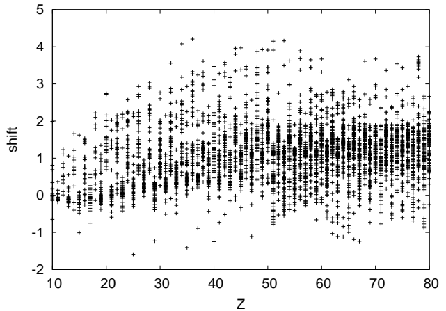
Figure 8: Shifts \delta (in MeV) of the maximum of the integrand relative to E_0 of the Gaussian approximation as a function of the target charge Z for (p, \alpha) reactions at T = 5 GK. The shifts are larger as for (\alpha, p) reactions and they are positive.
