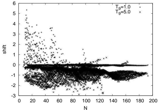
Figure 4: Shifts \delta (in MeV) of the maximum of the integrand relative to E_0 of the Gaussian approximation as a function of the target neutron number N for (p, \gamma) reactions at two temperatures. Almost no shift is observed at T_9 = 1.0 , except for proton-rich nuclei with negative reaction Q value. Shifts remain smaller than for (\alpha, \gamma) at T_9 = 5.0 .
