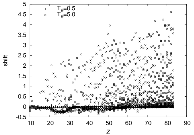
Figure 10: Shifts \delta (in MeV) of the maximum of the integrand relative to E_{\text{MB}} as a function of the target charge Z for (n,p) reactions at two temperatures. Almost no shift is observed at T_9 = 0.5 but shifts become large at T_9 = 5.0 .
