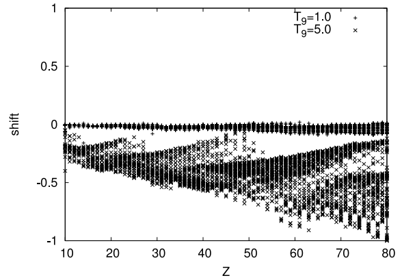
Figure 1: Shifts \delta (in MeV) of the maximum of the integrand relative to E_0 of the Gaussian approximation as a function of the target charge Z for (p,n) reactions at two temperatures. Almost no shift is observed at T_9 = 1.0 and shifts remain small for T_9 = 5.0 .
