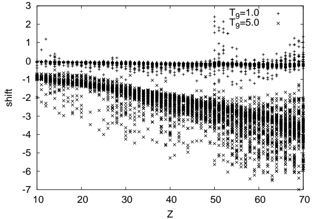
Figure 3: Shifts \delta (in MeV) of the maximum of the integrand relative to E_0 of the Gaussian approximation as a function of the target charge Z for (\alpha, \gamma) reactions at two temperatures. Almost no shift is observed at T_9 = 1.0 but shifts become large at T_9 = 5.0 .
