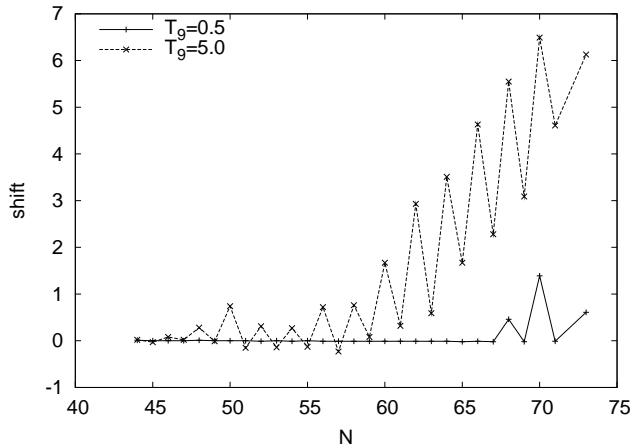
Figure 12: Shifts \delta of the maximum of the integrand relative to E_{\text{MB}} as function of the target neutron number N for (n,\alpha) reactions on Sn isotopes at two temperatures. Almost no shift is observed at T_9 = 0.5 but shifts become large at T_9 = 5.0 for the neutron-rich isotopes with small reaction Q value.
