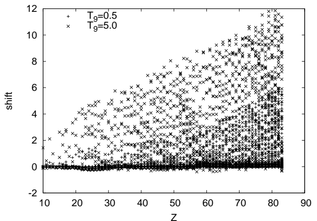
Figure 11: Shifts \delta (in MeV) of the maximum of the integrand relative to E_{\text{MB}} as a function of the target charge Z for (n,p) reactions at two temperatures. Almost no shift is observed at T_9 = 0.5 but shifts become very large at T_9 = 5.0 .
