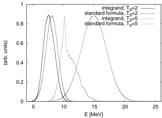
Figure 6: Comparison of actual reaction rate integrands \mathcal{F} and Gaussian approximations of the Gamow window for the reaction ^{169}\text{Tm}(\alpha,\gamma)^{173}\text{Lu} at T = 2 and 5 GK. The integrands and the Gaussians have been arbitrarily scaled to yield similar maximal values. While the shift is small for T_9 = 2 , it is about 5 MeV at T_9 = 5 . Also the asymmetry of the integrand can be clearly seen at T_9 = 5 .
