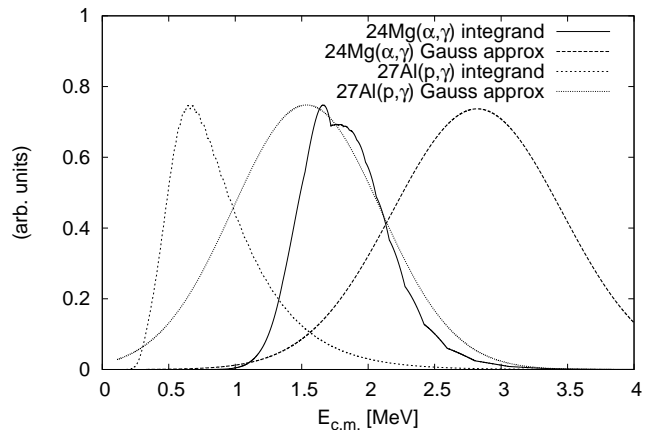
Figure 5: Comparison of actual reaction rate integrand \mathcal{F} and Gaussian approximation of the Gamow window for the reactions ^{24}\text{Mg}(\alpha,\gamma)^{28}\text{Si} at T = 2.5 GK and ^{27}\text{Al}(p,\gamma)^{28}\text{Si} at T = 3.5 GK. The integrands and the Gaussians have been arbitrarily scaled to yield similar maximal values.
