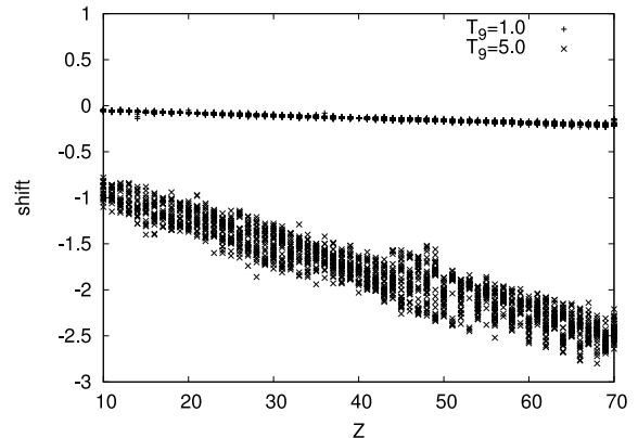
Figure 2: Shifts \delta (in MeV) of the maximum of the integrand relative to E_0 of the Gaussian approximation as a function of the target charge Z for (\alpha, n) reactions at two temperatures. Almost no shift is observed at T_9 = 1.0 and shifts reach a few MeV for T_9 = 5.0 .
