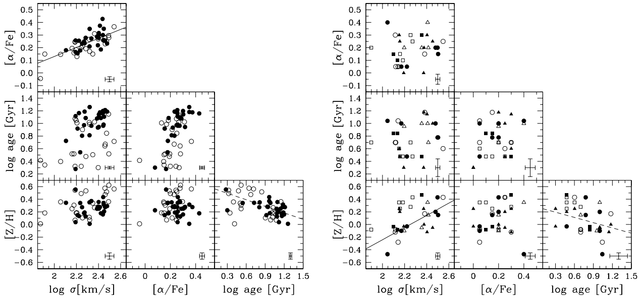
Figure 8. The global relations between \log age, [Z/H] , [\alpha/Fe] and \log \sigma are shown. The symbols are the same than figure 3, and figure 2. The left plot shows the clusters galaxies, the right panel combines the 2dFGRS and Colbert's samples with the LDE sample. The solid lines identify a least-square fit between the parameters. Typical error bars are shown at the lower-right corner of each diagram. These do not account for the fact that the errors on age, [Z/H] and [\alpha/Fe] can be correlated, which can impact the significance of the observed correlations between these parameters. In particular, this can be the case for the age- [Z/H] relations, which are shown by dashed lines.
