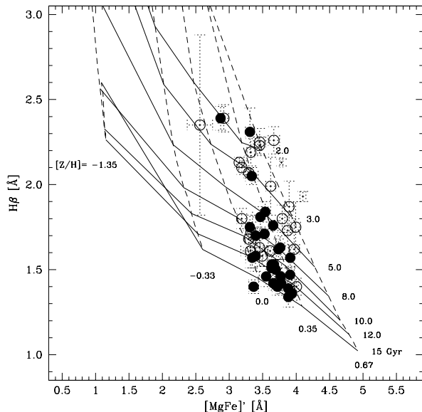
Figure 4. The age-sensitive index H\beta as a function of the metallicity-sensitive index [MgFe]' . Overplotted are the stellar population models of Thomas et al. (2003a). The solid lines are lines of constant age from 2 to 15 Gyr. The dashed, almost vertical, lines stand for constant metallicity from [Z/H] = -1.35 to 0.67 dex. The age and metallicity steps are indicated to the right and at the bottom of the model predictions. The symbol definitions are the same as in Figure 2.
