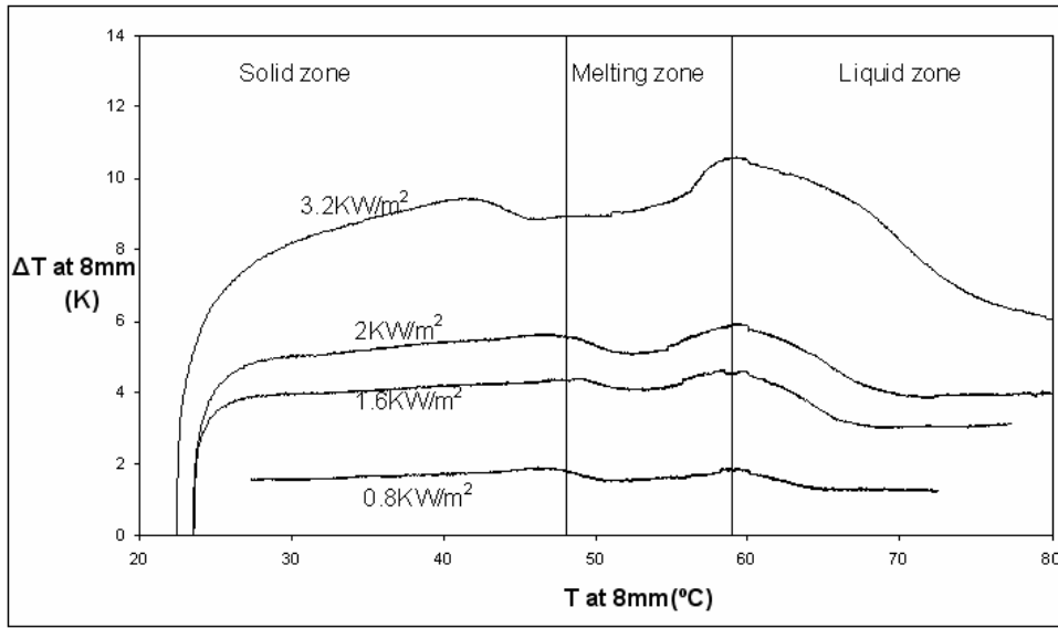
Figure 7 Effect of heat flux on the temperature difference between the heated wall temperature and the PCM temperature at 8mm during the melting process.
