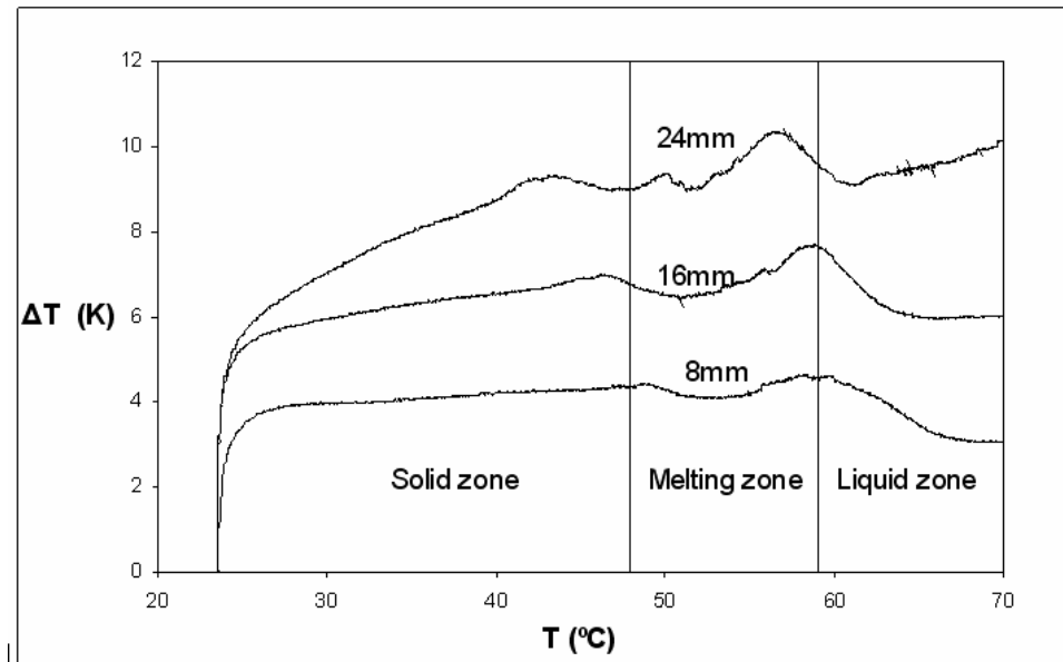
Figure 6 Variation of temperature difference with the local PCM temperature during the melting process ( 1.6\text{KW/m}^2 ).
