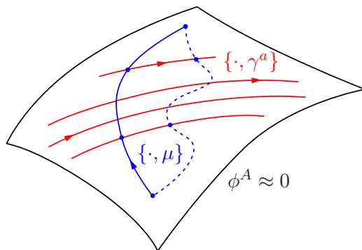
Figure 1. Symmetries in constrained systems.
