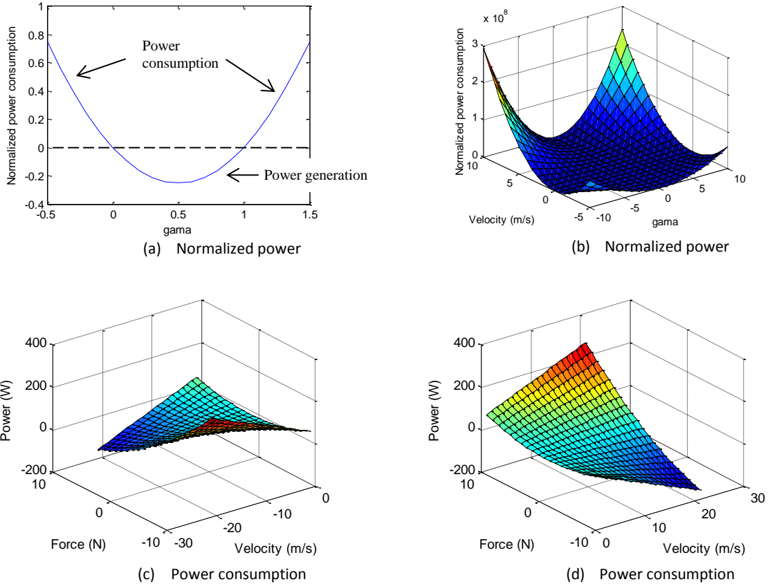
Figure 4: Power consumption and power generation by a regenerative system
