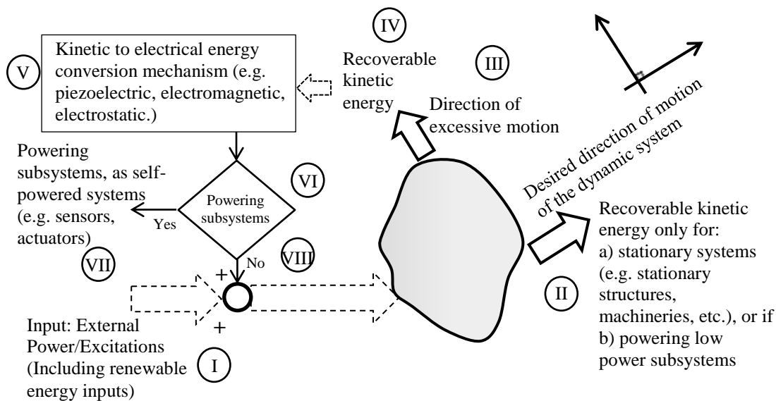
Figure 1: The concept of self-powered dynamic systems
