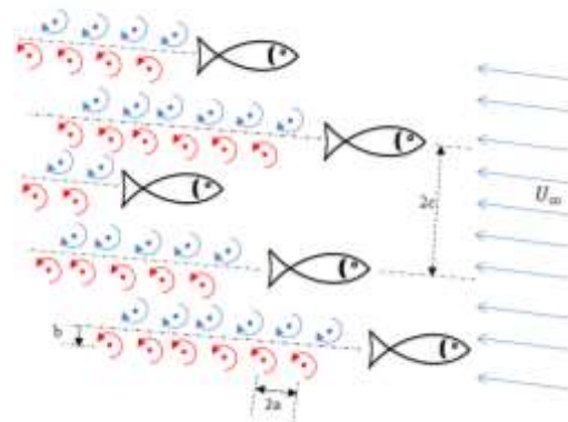
(b) Fish schooling and the vortices generated by fish locomotion as the basis of energy harvesters design
