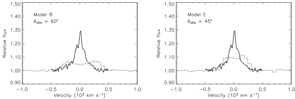
Figure 10. Comparison of the observed \text{Br}\alpha profile for GL989 (taken from Bunn et al. 1995; heavy line) with computed profiles from Model B (for viewing angle of 60^\circ ; light histogram on left) and Model E (for viewing angle of 45^\circ ; light histogram on right). These models and angles have been chosen for comparison of profile shapes since they give \text{Br}\alpha equivalent-widths which are similar to that observed for GL989. We show \text{Br}\alpha only – since there are discrepancies between the modelled and observed EWRs (see text), the models shown significantly underpredict the \text{Br}\gamma -EW and therefore do not simultaneously allow useful comparisons of line shapes for all lines. Comparing the observed \text{Br}\gamma or \text{Pf}\gamma profiles to models which reproduce their EWs leads to the same conclusions obtained from considering \text{Br}\alpha only.
