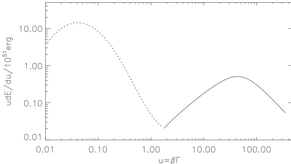
Fig. 1. – Schematic figure showing the distribution of energy E as a function of four velocity u \equiv \Gamma\beta = (\Gamma^2 - 1)^{1/2} ( dE/d\ln u , in units of 10^{51} erg), that is implied if the flat decay phase is due to type (1) energy injection (from [17]). It has one relativistic component ( solid line ) with total energy \sim 10^{51} erg and peak at u \sim 30 - 50 that produces the GRB ( u \gtrsim 10^2 ) and the afterglow radiations. The power-law index above the peak for this component is well constrained by the X-ray data (the shallow part of the light-curve) and is dE/d\ln u \propto u^{-a} with 1 \lesssim a \lesssim 2.5 for a uniform external medium. The slope below the peak is not well constrained (either than being positive) and is taken to be 1. The second component (dashed curve) shows schematically the kinetic energy in non-relativistic ejecta in the supernova accompanying the GRB, which peaks at a typical velocity around \sim 10^4 km s ^{-1} , and has an energy of the order of \sim 10^{52} erg.
